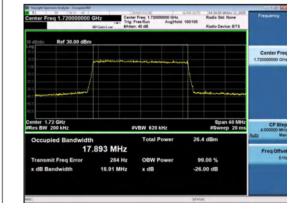
Band4-20MHz-16QAM-20050-100RB#0-PASS
