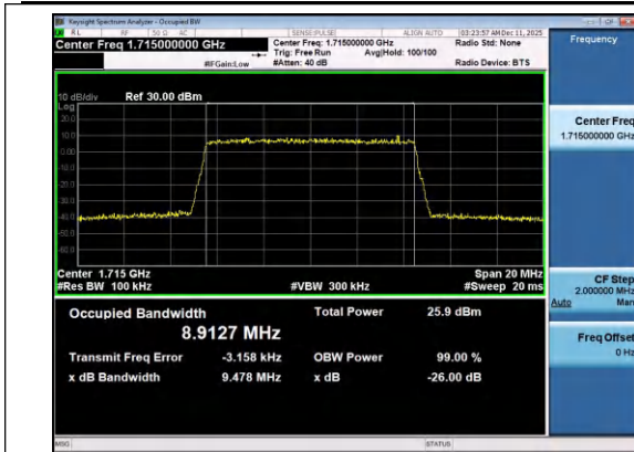
Band4-10MHz-16QAM-20000-50RB#0-PASS
