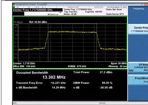
Band4-15MHz-QPSK-20025-75RB#0-PASS
