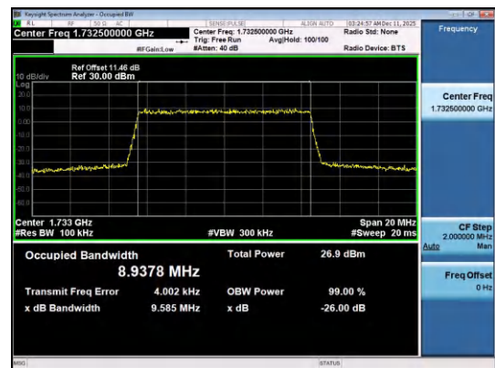
Band4-10MHz-QPSK-20175-50RB#0-PASS
