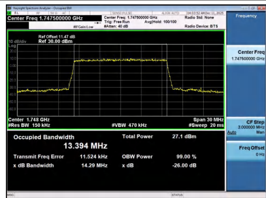
Band4-15MHz-QPSK-20325-75RB#0-PASS
