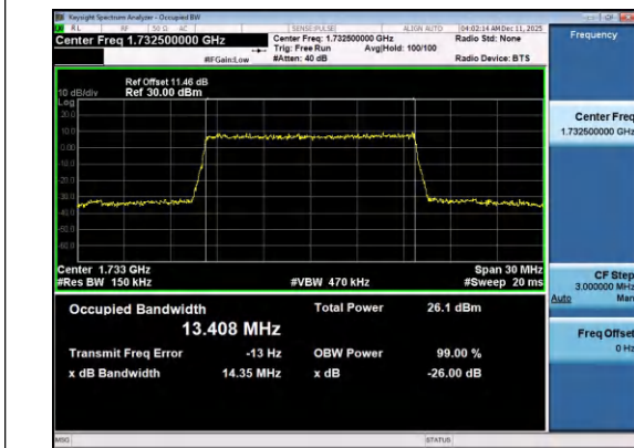
Band4-15MHz-16QAM-20175-75RB#0-PASS
