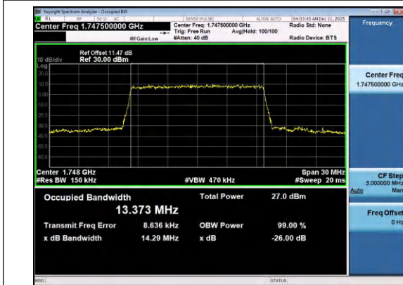
Band4-15MHz-QPSK-20325-75RB#0-PASS
