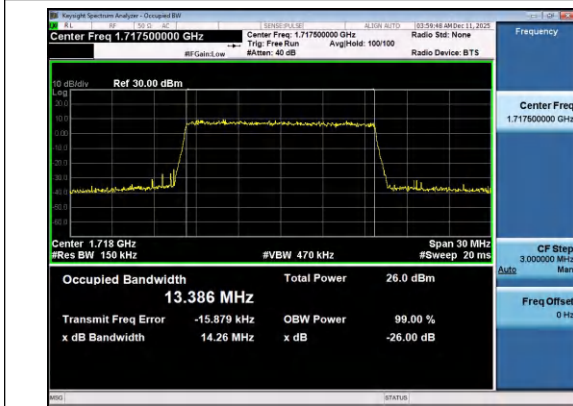
Band4-15MHz-16QAM-20025-75RB#0-PASS
