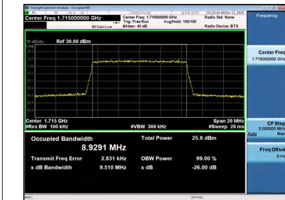
Band4-10MHz-16QAM-20000-50RB#0-PASS
