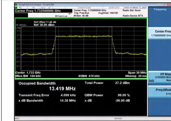
Band4-15MHz-QPSK-20175-75RB#0-PASS
