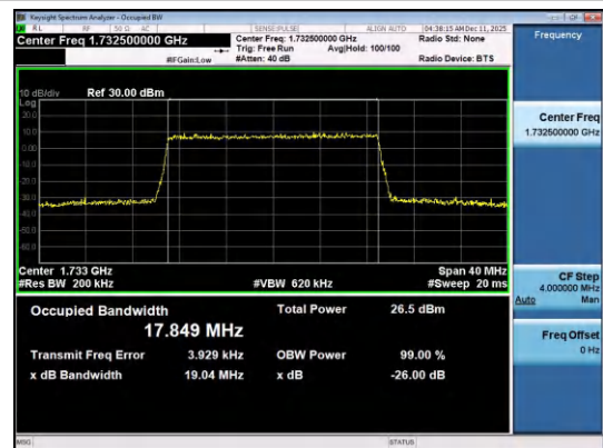
Band4-20MHz-16QAM-20175-100RB#0-PASS
