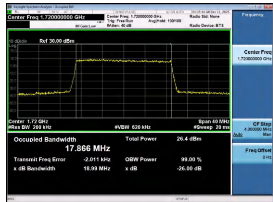
Band4-20MHz-16QAM-20050-100RB#0-PASS
