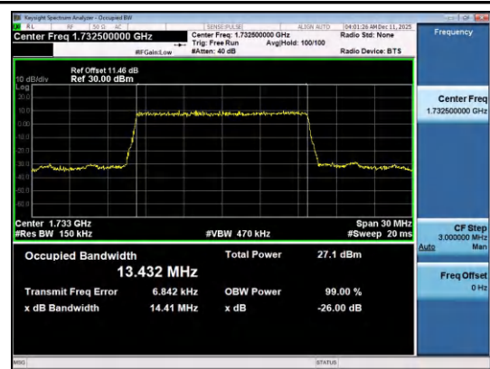
Band4-15MHz-QPSK-20175-75RB#0-PASS
