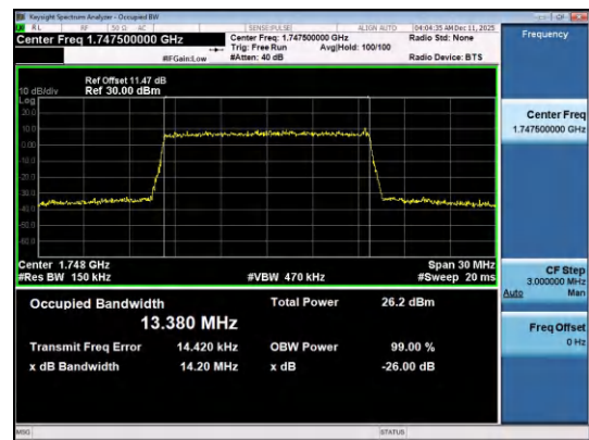
Band4-15MHz-16QAM-20325-75RB#0-PASS
