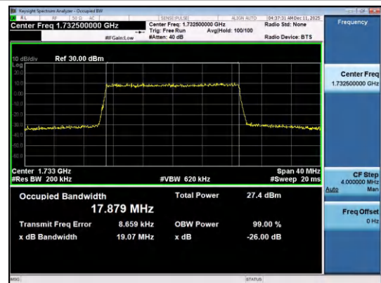
Band4-20MHz-QPSK-20175-100RB#0-PASS
