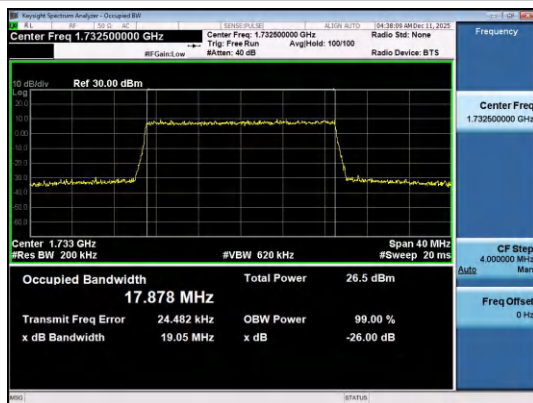
Band4-20MHz-16QAM-20175-100RB#0-PASS
