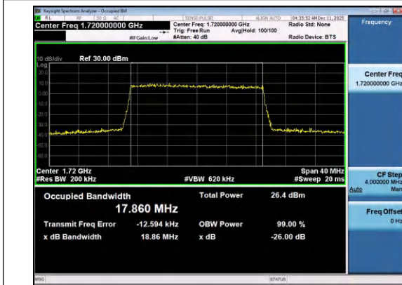
Band4-20MHz-16QAM-20050-100RB#0-PASS
