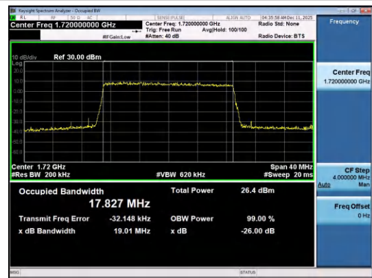
Band4-20MHz-16QAM-20050-100RB#0-PASS
