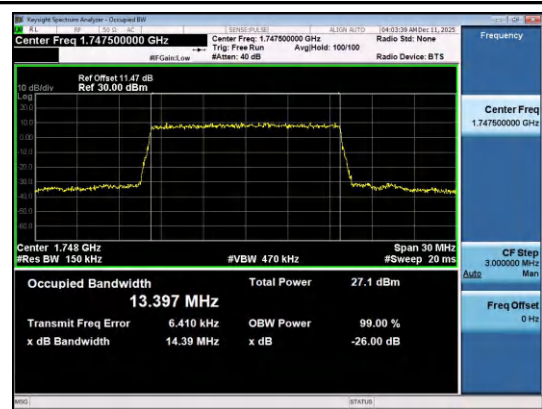
Band4-15MHz-QPSK-20325-75RB#0-PASS
