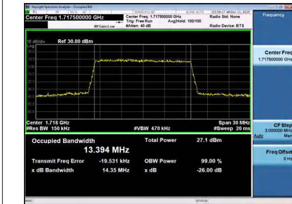
Band4-15MHz-QPSK-20025-75RB#0-PASS
