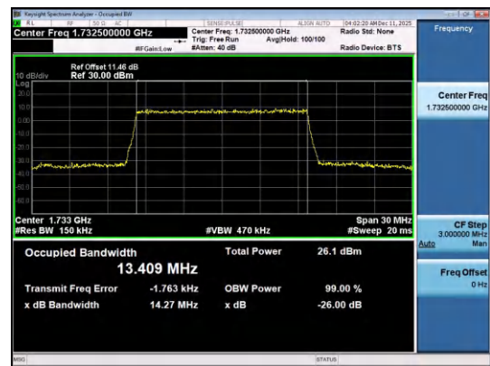
Band4-15MHz-16QAM-20175-75RB#0-PASS
