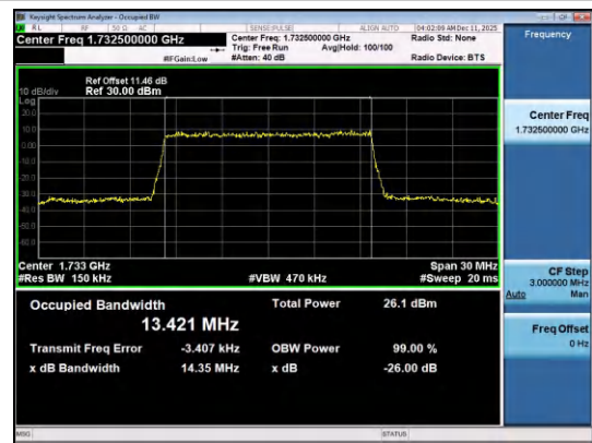
Band4-15MHz-16QAM-20175-75RB#0-PASS
