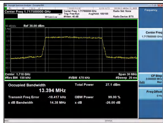
Band4-15MHz-QPSK-20025-75RB#0-PASS
