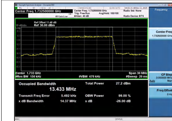
Band4-15MHz-QPSK-20175-75RB#0-PASS
