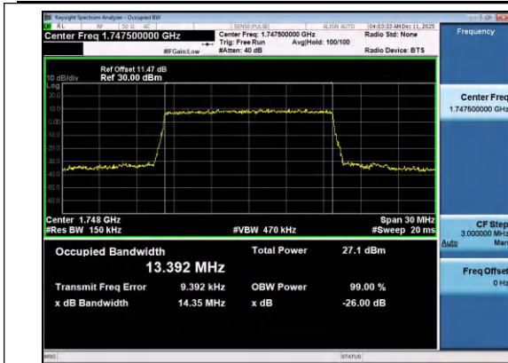
Band4-15MHz-QPSK-20325-75RB#0-PASS
