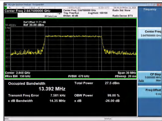
Band41(2535-2655)-15MHz-16QAM-41165-75RB#0-P ASS
