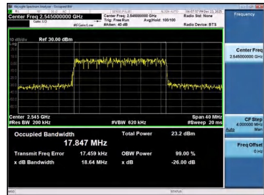
Band41(2535-2655)-20MHz-16QAM-40140-100RB#0- PASS
