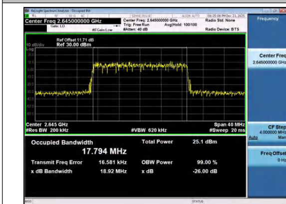
Band41(2535-2655)-20MHz-QPSK-41140-100RB#0-P ASS
