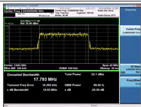
Band41(2535-2655)-20MHz-QPSK-41140-100RB#0-P ASS
