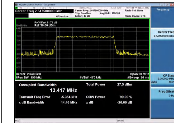
Band41(2535-2655)-15MHz-16QAM-41165-75RB#0-P ASS
