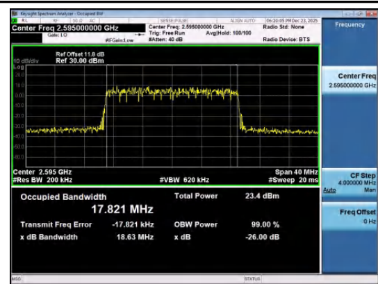
Band41(2535-2655)-20MHz-16QAM-40640-100RB#0- PASS
