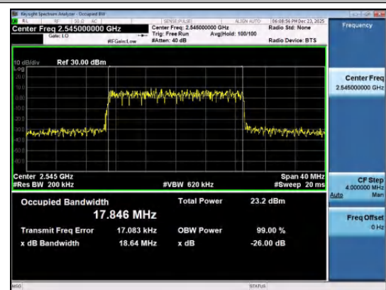
Band41(2535-2655)-20MHz-16QAM-40140-100RB#0- PASS
