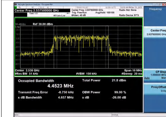
Band41(2535-2655)-5MHz-16QAM-40065-25RB#0-PA
