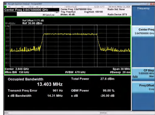
Band41(2535-2655)-15MHz-16QAM-41165-75RB#0-P ASS
