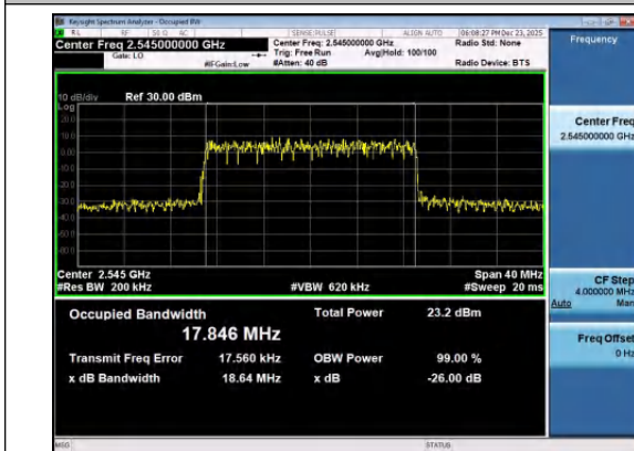
Band41(2535-2655)-20MHz-16QAM-40140-100RB#0- PASS
