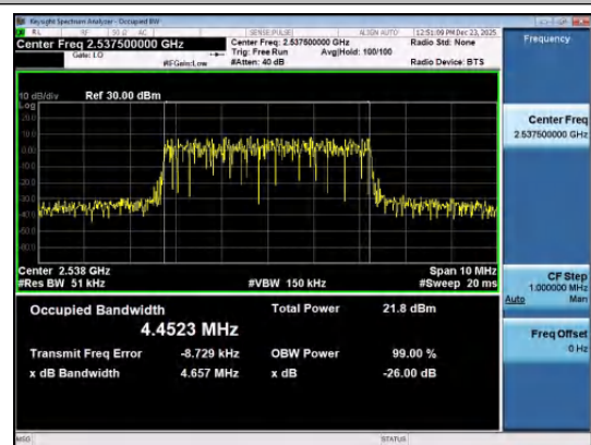
Band41(2535-2655)-5MHz-16QAM-40065-25RB#0-PA
