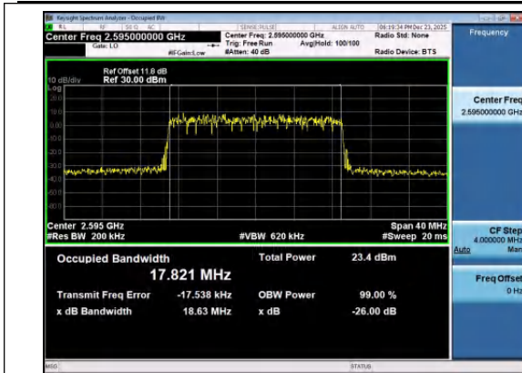
Band41(2535-2655)-20MHz-16QAM-40640-100RB#0- PASS
