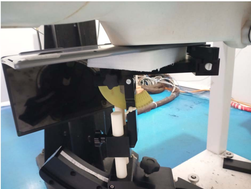
Body Back ANT 2 Setup Photo(0mm)
