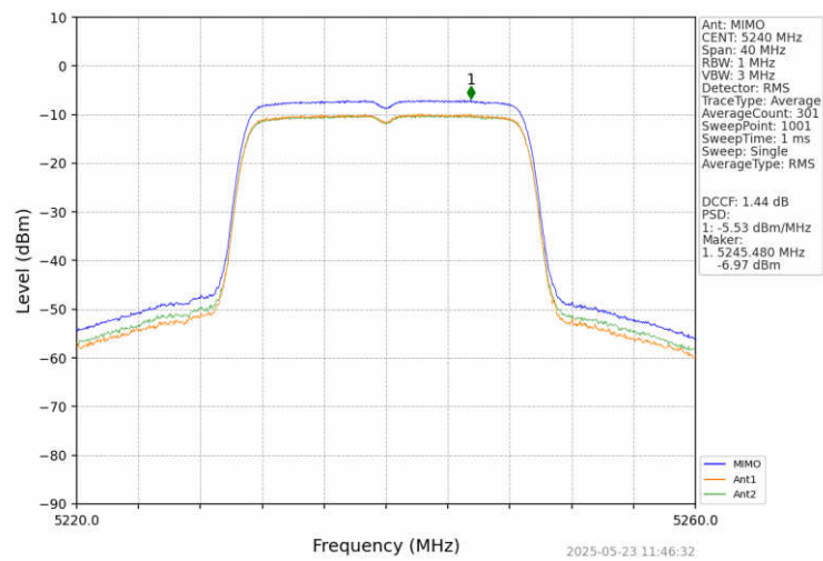
802.11ac(VHT20)_HCH_5240MHz_MIMO_NTNV
