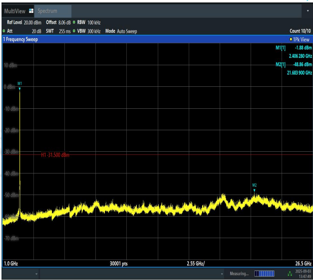
11N20SISO-Ant1-2412-1000~26500-PASS
