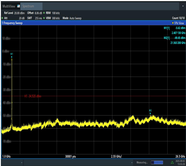
11N40SISO-Ant1-2422-1000~26500-PASS
