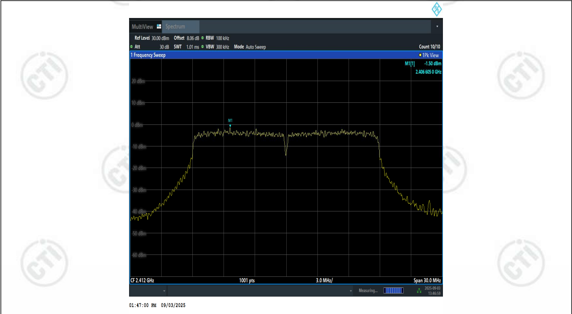
11N20SISO-Ant1-2412-0~Reference-PASS
