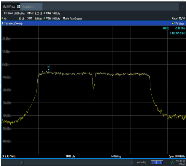
11N40SISO-Ant1-2437-0~Reference-PASS
