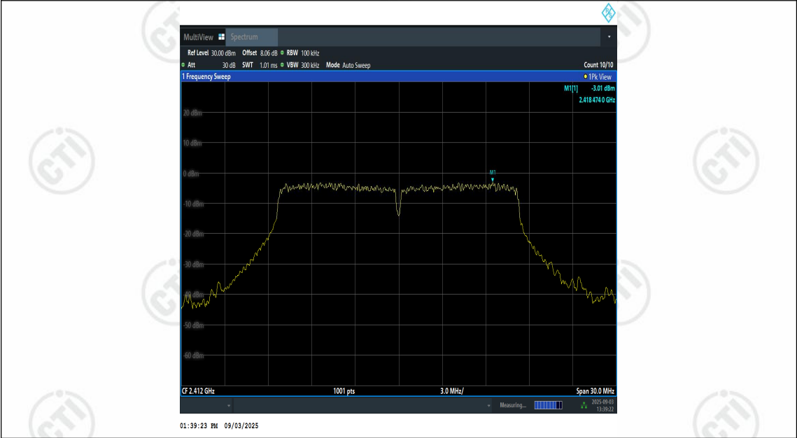
11G-Ant1-2412-0~Reference-PASS
