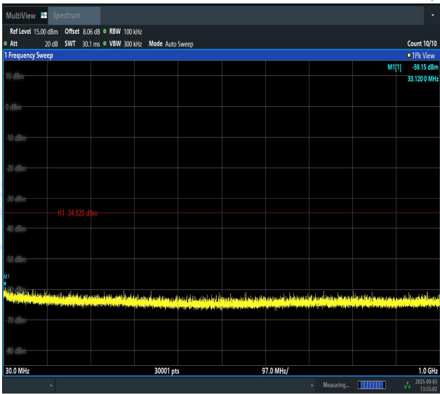
11N40SISO-Ant1-2422-30~1000-PASS
