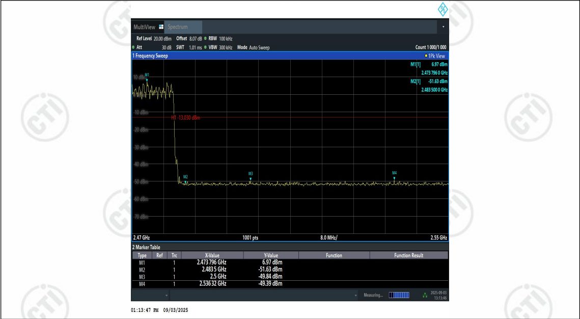
3DH5-Ant1-Hop_2480-PASS
