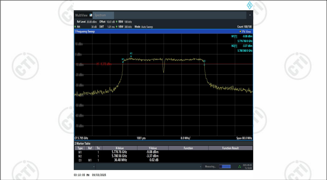
11N40SISO-Ant1-5795-PASS
