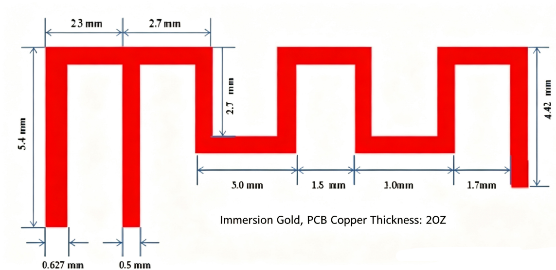
Antenna Dimension for ESP-F
