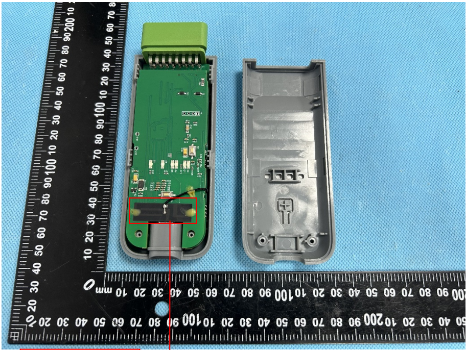
WIFI Ant.
