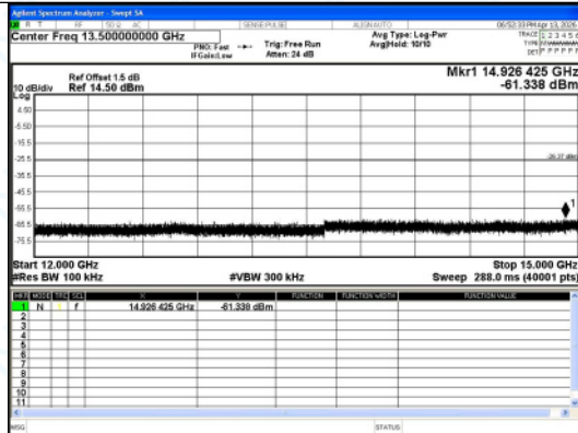
12000.0 MHz - 15000.0 MHz GFSK DH5 Channel 78
