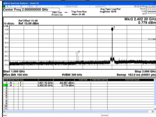
1000.0 MHz - 3000.0 MHz 8DPSK 3-DH5 Channel 0
