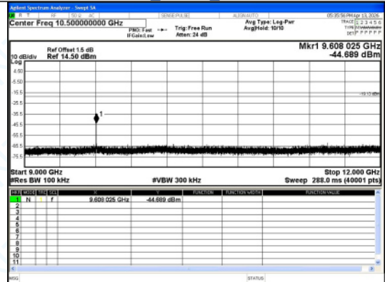
9000.0 MHz - 12000.0 MHz 8DPSK 3-DH5 Channel 0
