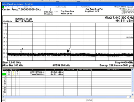
6000.0 MHz - 9000.0 MHz \pi/4 DQPSK 2-DH5 Channel 78
