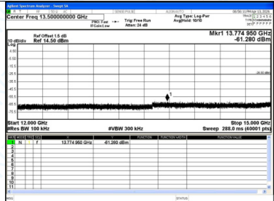
12000.0 MHz - 15000.0 MHz pi/4DQPSK 2-DH5 Channel 78
