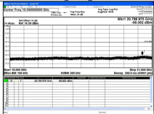
18000.0 MHz - 21000.0 MHz pi/4DQPSK 2-DH5 Channel 78
