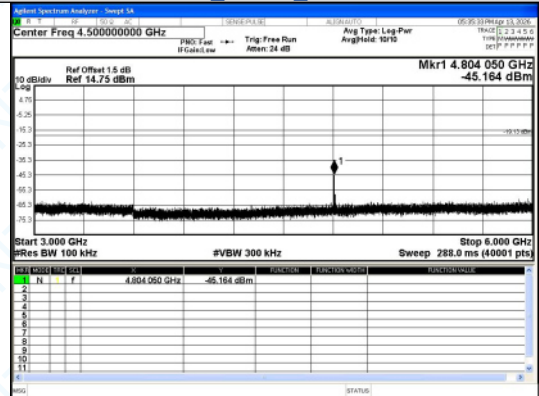
3000.0 MHz - 6000.0 MHz 8DPSK 3-DH5 Channel 0
