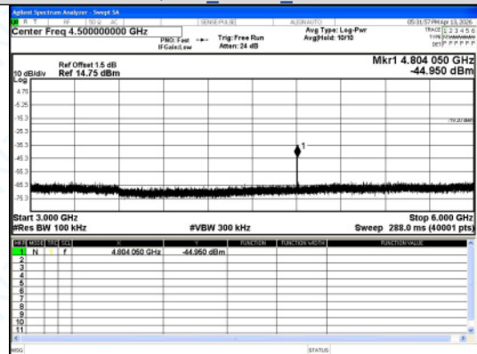
3000.0 MHz - 6000.0 MHz \pi/4 DQPSK 2-DH5 Channel 0
