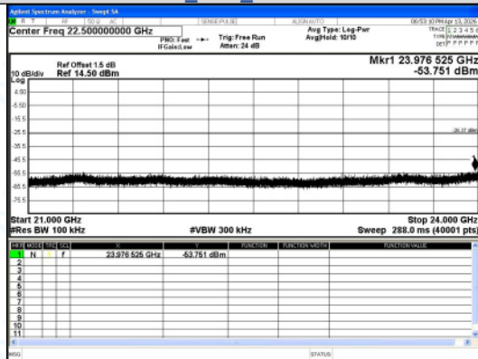
21000.0 MHz - 24000.0 MHz GFSK DH5 Channel 78
