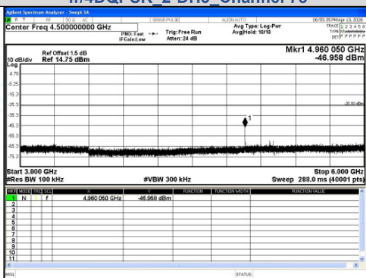
3000.0 MHz - 6000.0 MHz \pi/4 DQPSK 2-DH5 Channel 78
