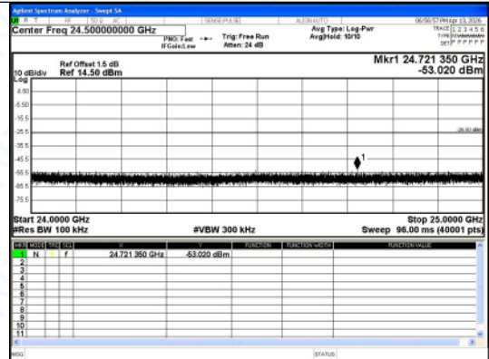
24000.0 MHz - 25000.0 MHz \pi/4 DQPSK 2-DH5 Channel 78
