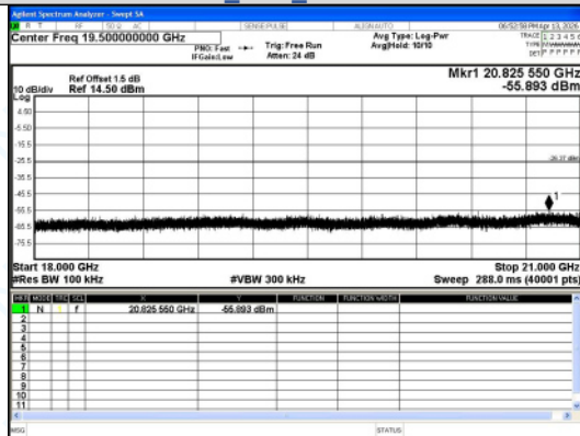
18000.0 MHz - 21000.0 MHz GFSK DH5 Channel 78
