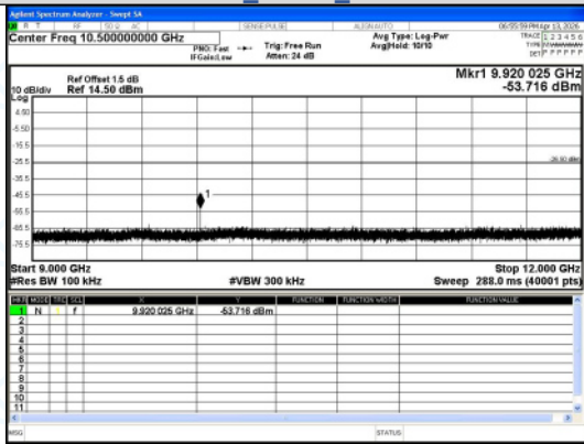
9000.0 MHz - 12000.0 MHz \pi/4 DQPSK 2-DH5 Channel 78
