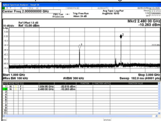
1000.0 MHz - 3000.0 MHz \pi/4 DQPSK 2-DH5 Channel 78
