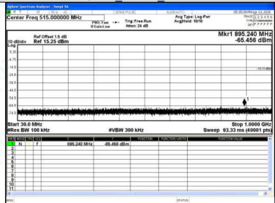
30.0 MHz - 1000.0 MHz 8DPSK 3-DH5 Channel 0
