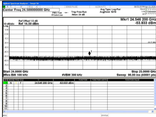
24000.0 MHz - 25000.0 MHz GFSK DH5 Channel 78
