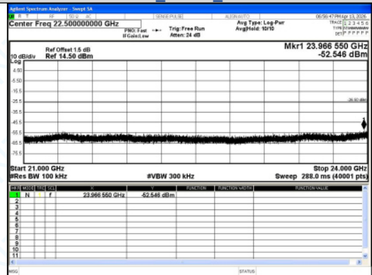
21000.0 MHz - 24000.0 MHz pi/4DQPSK 2-DH5 Channel 78
