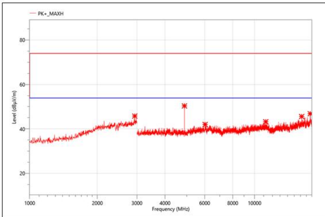
3-DH5 2441
