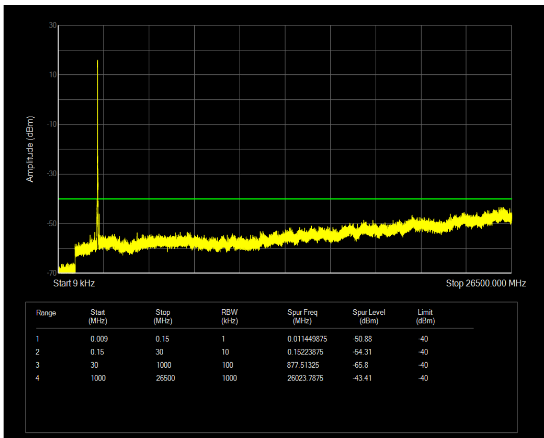
Band40a QPSK BW=5MHz Channel=38725 RB Size=1 Position=#0
