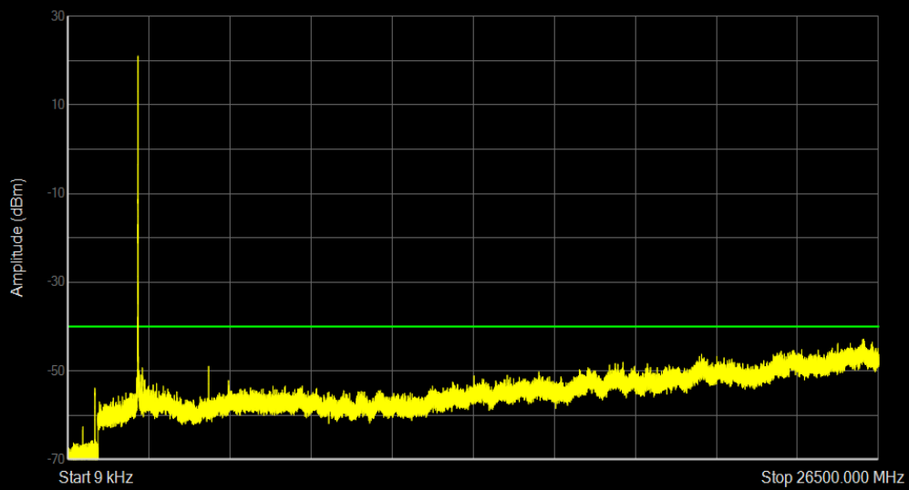
Band40a QPSK BW=5MHz Channel=38750 RB Size=1 Position=#0
