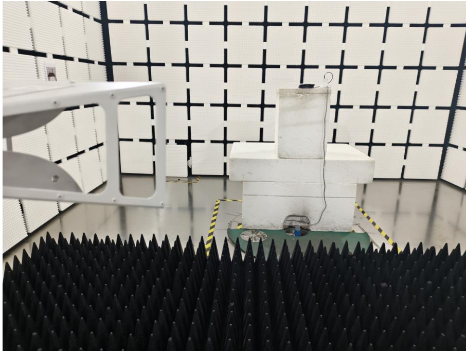
Above 1GHz-BT
