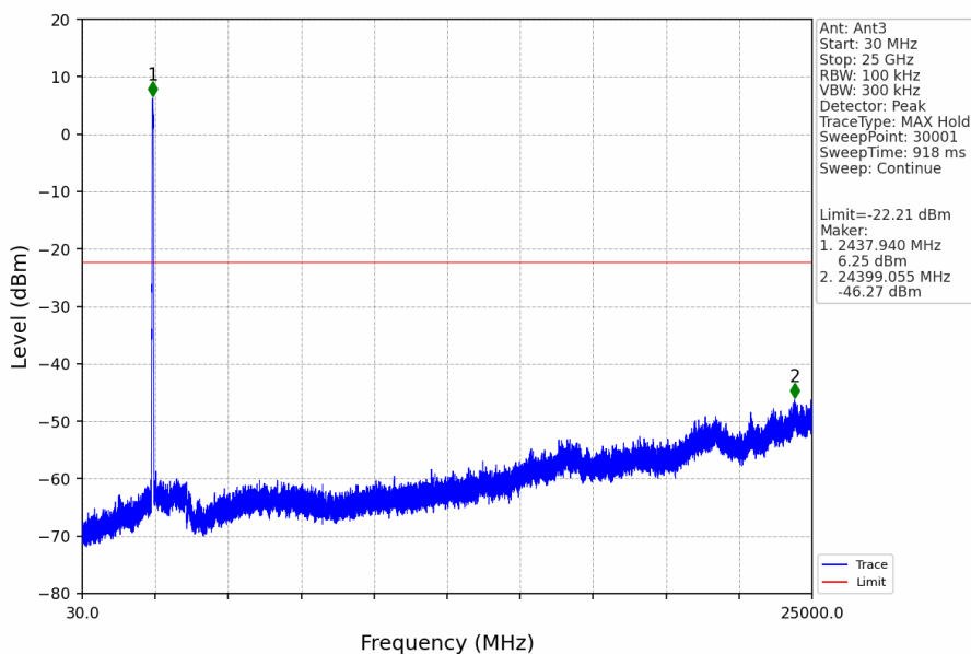
60M_HCH_2442.5MHz_Ant3_NTNV
