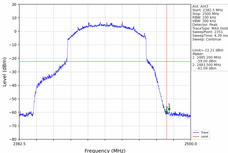
60M_HCH_2442.5MHz_Ant3_NTNV
