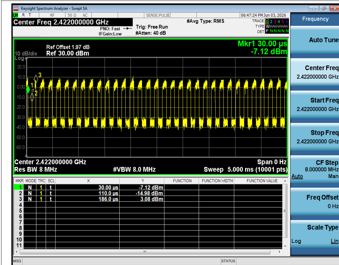
Duty Cycle NVNT n40 2422MHz Ant1
