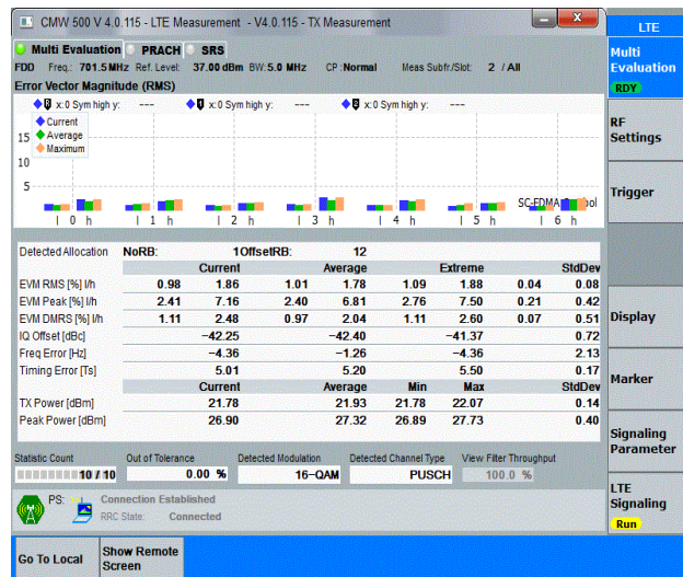
Band12-5MHz-16QAM-23035-1RB#12-PASS
