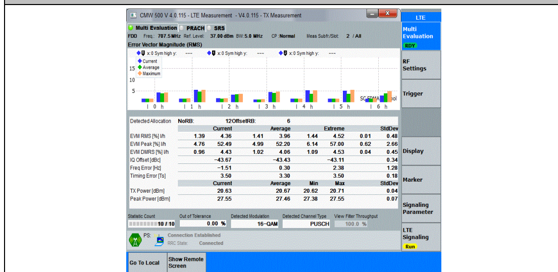
Band12-5MHz-16QAM-23095-12RB#6-PASS
