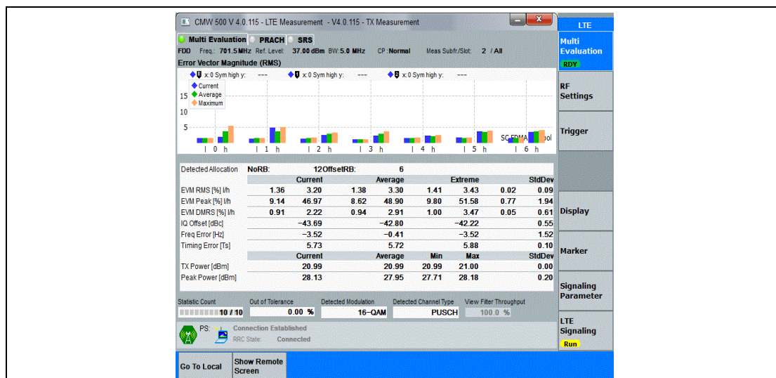
Band12-5MHz-16QAM-23035-12RB#6-PASS
