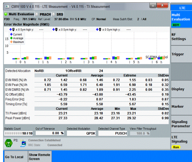
Band12-5MHz-QPSK-23035-1RB#24-PASS
