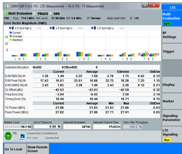
Band12-3MHz-QPSK-23165-8RB#0-PASS
