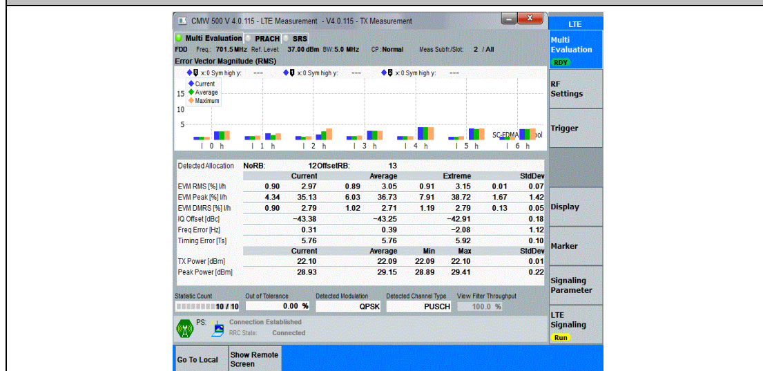
Band12-5MHz-QPSK-23035-12RB#13-PASS
