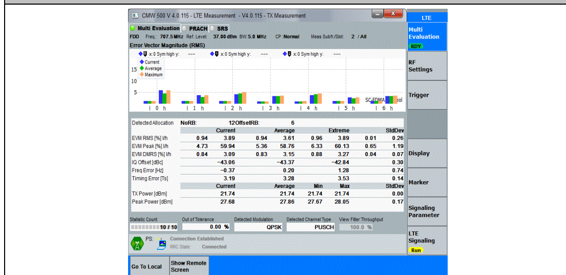
Band12-5MHz-QPSK-23095-12RB#6-PASS
