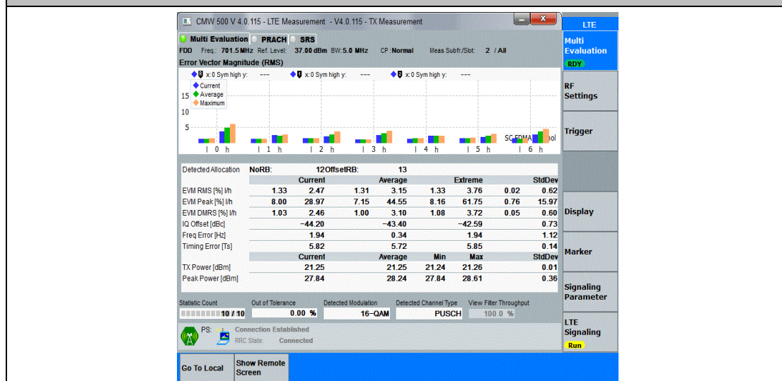
Band12-5MHz-16QAM-23035-12RB#13-PASS
