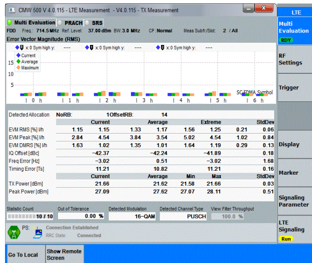
Band12-3MHz-16QAM-23165-1RB#14-PASS
