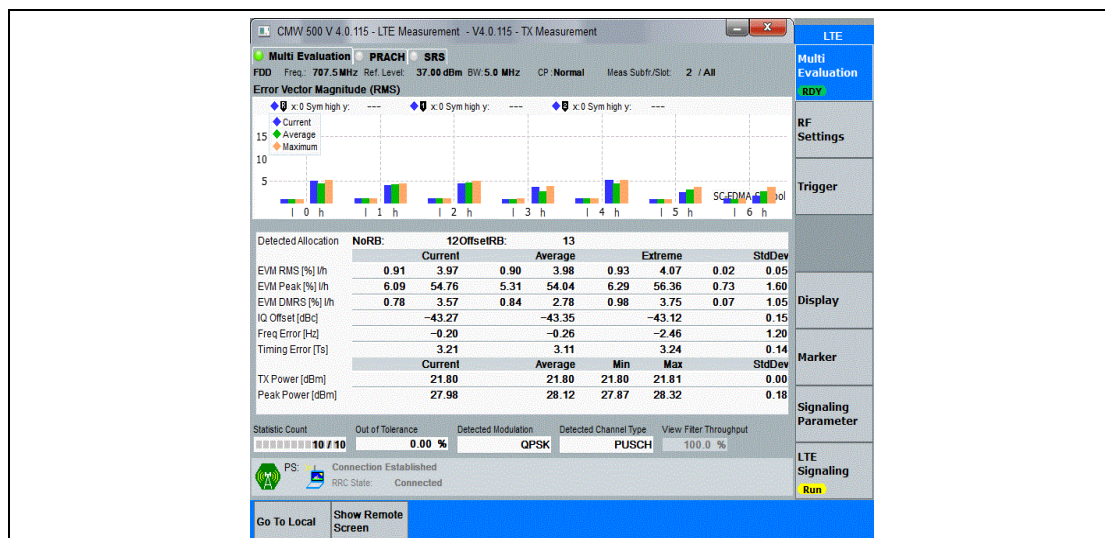
Band12-5MHz-QPSK-23095-12RB#13-PASS
