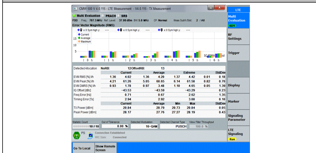
Band12-5MHz-16QAM-23095-12RB#13-PASS
