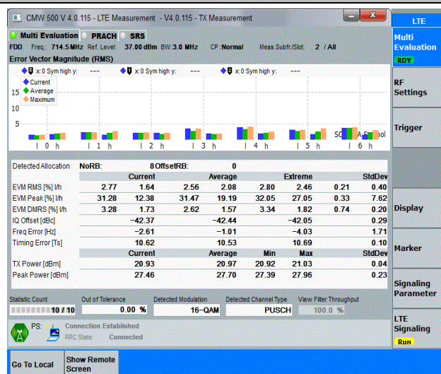
Band12-3MHz-16QAM-23165-8RB#0-PASS
