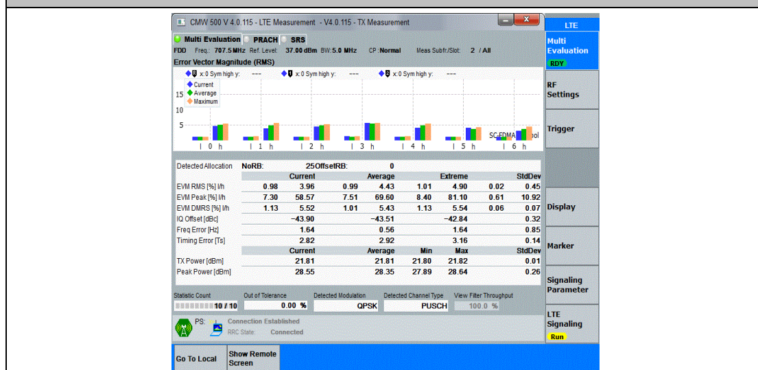
Band12-5MHz-QPSK-23095-25RB#0-PASS
