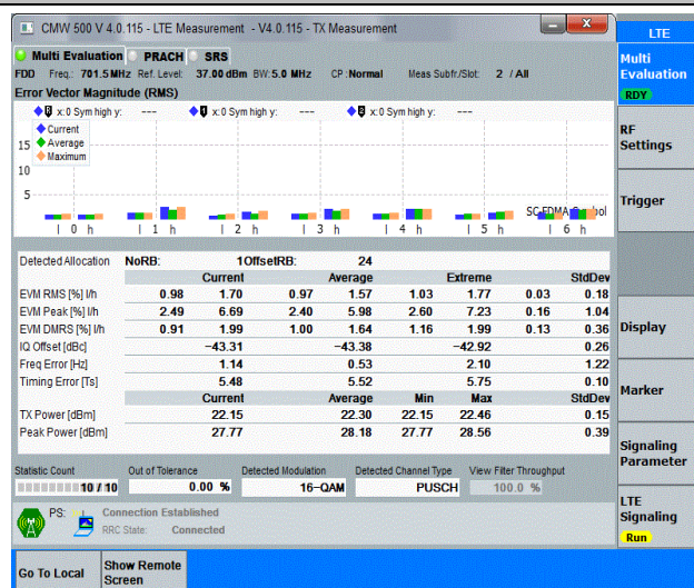
Band12-5MHz-16QAM-23035-1RB#24-PASS
