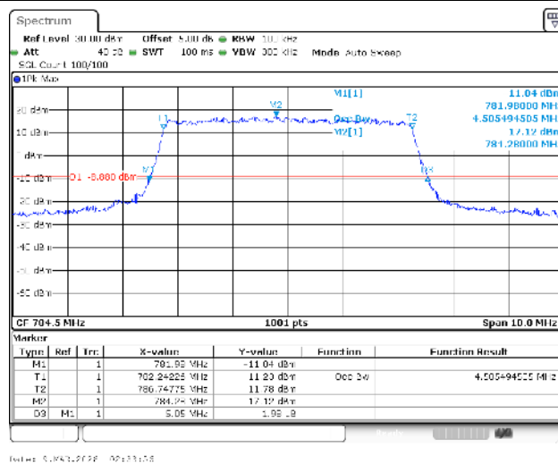
Band13-5MHz-16QAM-23255-25RB#0-PASS
