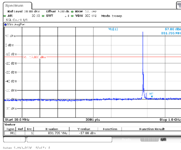
Band13-5MHz-16QAM-23255-1RB#0-30~1000-PASS
