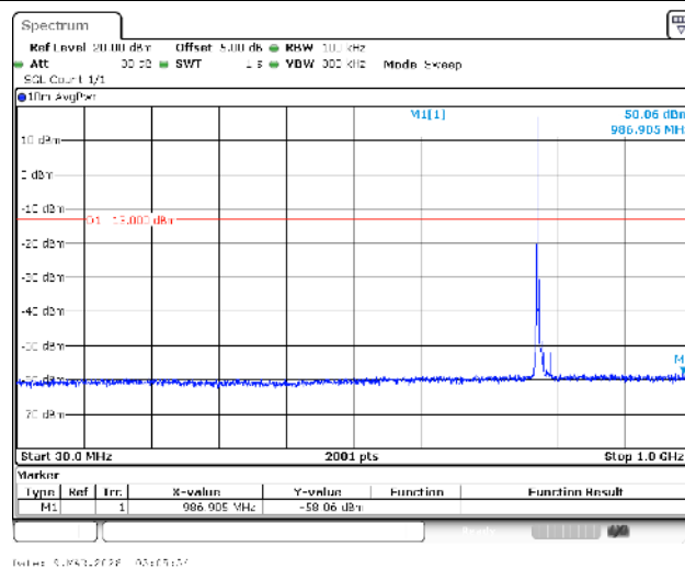
Band13-5MHz-16QAM-23205-1RB#0-30~1000-PASS
