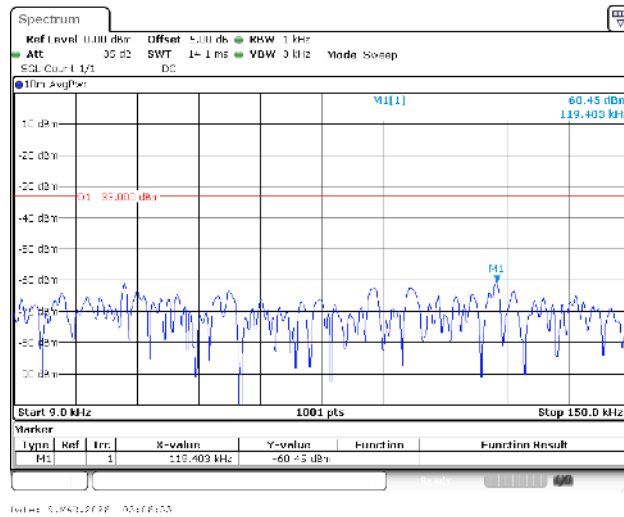
Band13-5MHz-16QAM-23230-1RB#0-0.009~0.15-PASS
