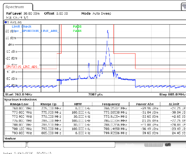
Band13-5MHz-16QAM-23255-1RB#24-PASS
