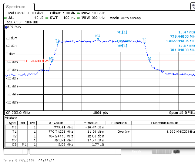
Band13-5MHz-QPSK-23230-25RB#0-PASS
