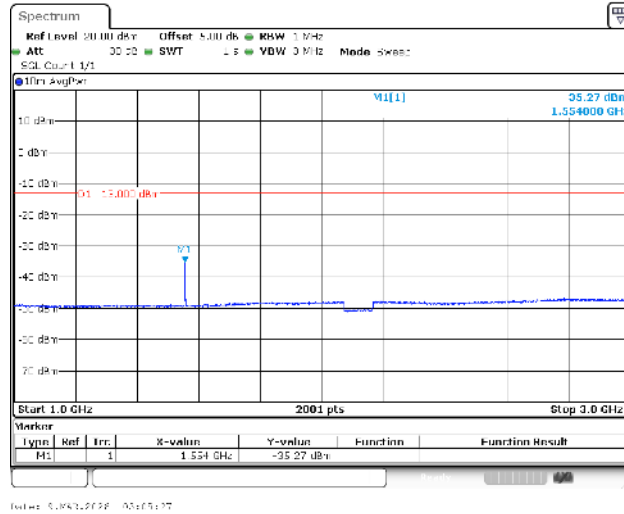
Band13-5MHz-QPSK-23205-1RB#0-1000~3000-PASS
