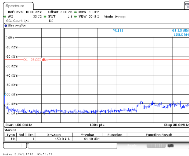
Band13-10MHz-16QAM-23230-1RB#0-0.15~30-PASS
