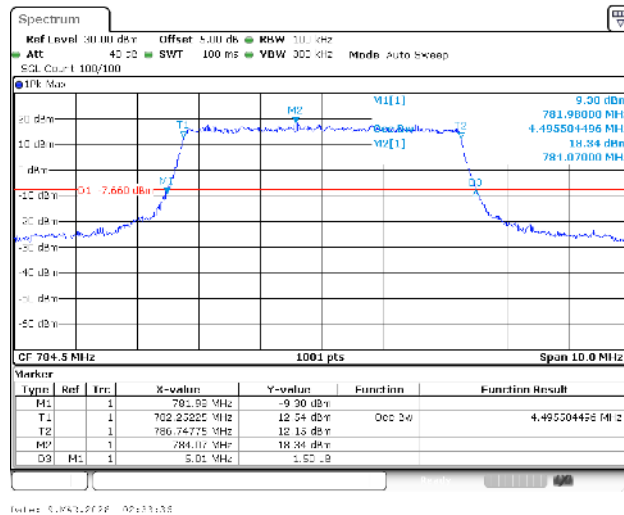
Band13-5MHz-QPSK-23255-25RB#0-PASS
