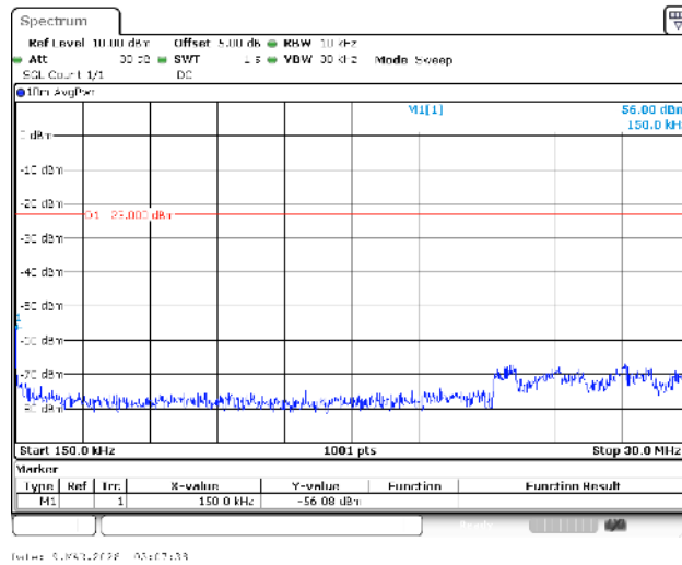
Band13-5MHz-QPSK-23255-1RB#0-0.15~30-PASS
