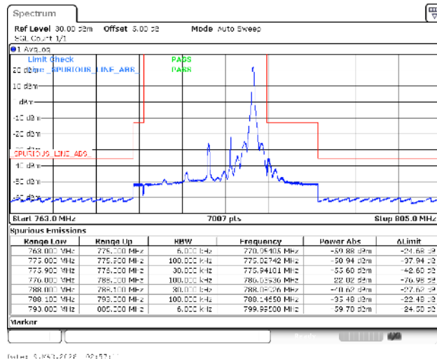
Band13-5MHz-QPSK-23255-1RB#24-PASS
