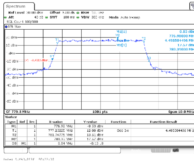
Band13-5MHz-QPSK-23205-25RB#0-PASS
