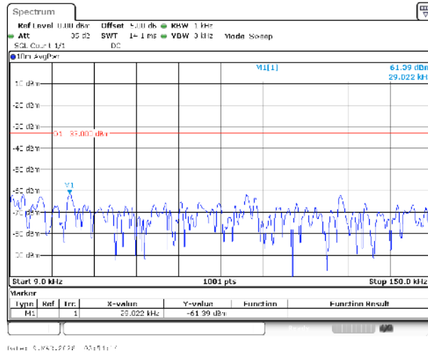
Band13-10MHz-16QAM-23230-1RB#0-0.009~0.15-PASS
