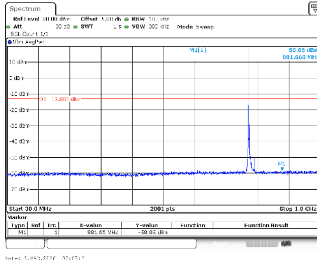
Band13-5MHz-QPSK-23205-1RB#0-30~1000-PASS
