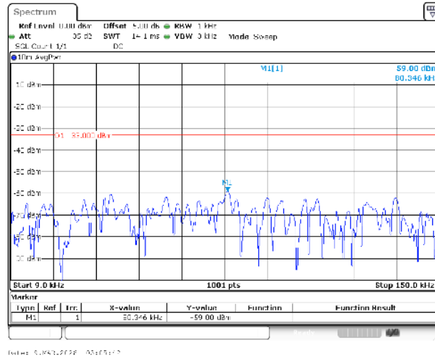
Band13-5MHz-16QAM-23205-1RB#0-0.009~0.15-PASS
