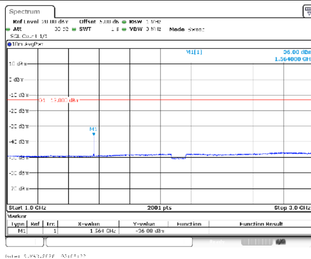
Band13-5MHz-16QAM-23255-1RB#0-1000~3000-PASS
