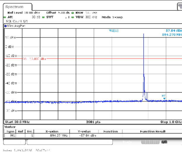
Band13-5MHz-QPSK-23255-1RB#0-30~1000-PASS
