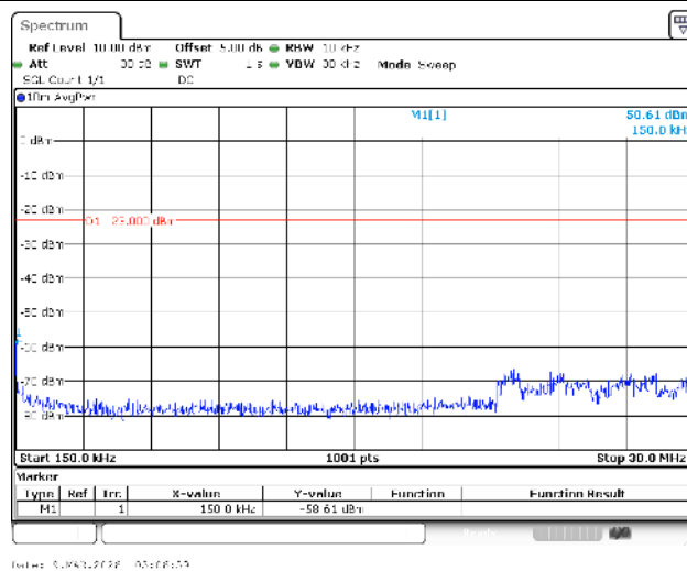
Band13-5MHz-16QAM-23230-1RB#0-0.15~30-PASS
