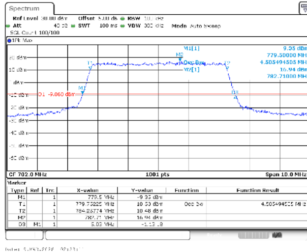
Band13-5MHz-16QAM-23230-25RB#0-PASS
