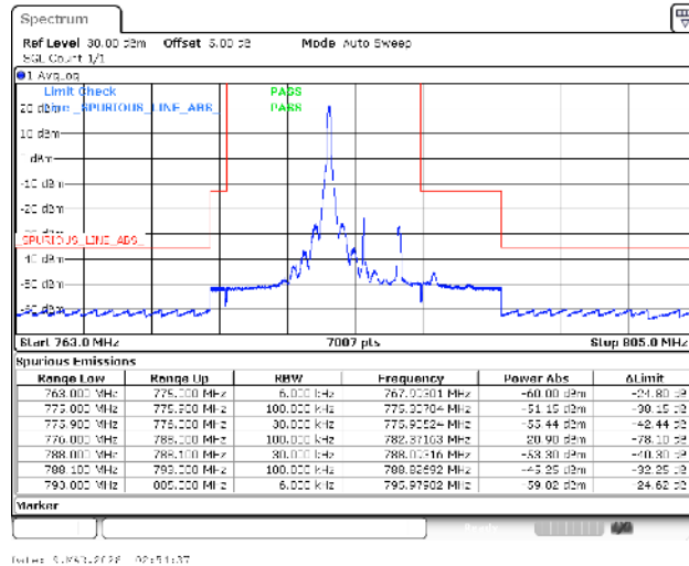
Band13-5MHz-16QAM-23255-1RB#0-PASS
