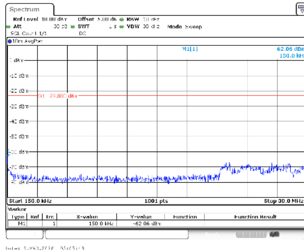
Band13-5MHz-16QAM-23205-1RB#0-0.15~30-PASS
