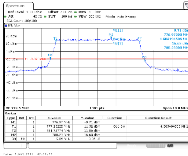
Band13-5MHz-16QAM-23205-25RB#0-PASS
