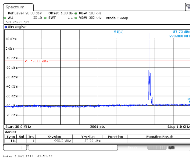
Band13-10MHz-16QAM-23230-1RB#0-30~1000-PASS
