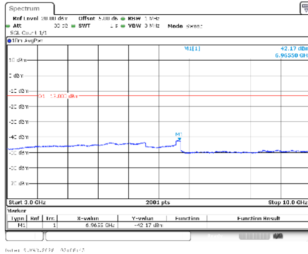
Band13-5MHz-QPSK-23230-1RB#0-3000~10000-PASS
