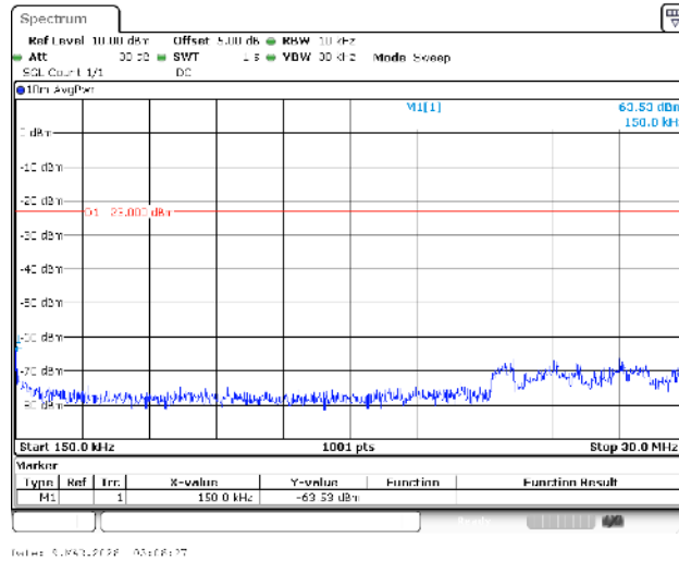
Band13-5MHz-QPSK-23230-1RB#0-0.15~30-PASS
