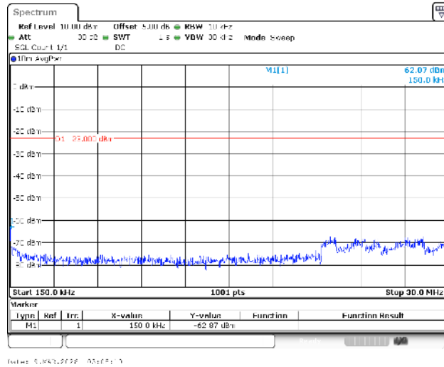
Band13-5MHz-16QAM-23255-1RB#0-0.15~30-PASS
