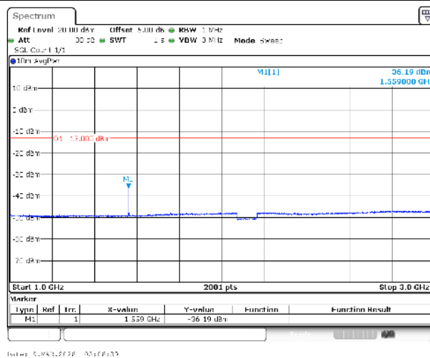
Band13-5MHz-QPSK-23230-1RB#0-1000~3000-PASS
