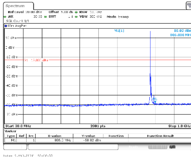
Band13-5MHz-QPSK-23230-1RB#0-30~1000-PASS
