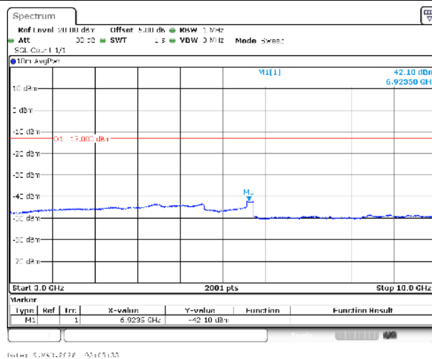
Band13-5MHz-QPSK-23205-1RB#0-3000~10000-PASS
