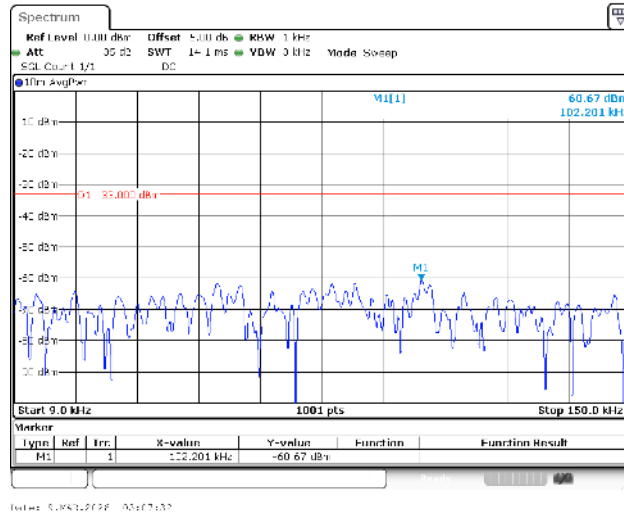
Band13-5MHz-QPSK-23255-1RB#0-0.009~0.15-PASS
