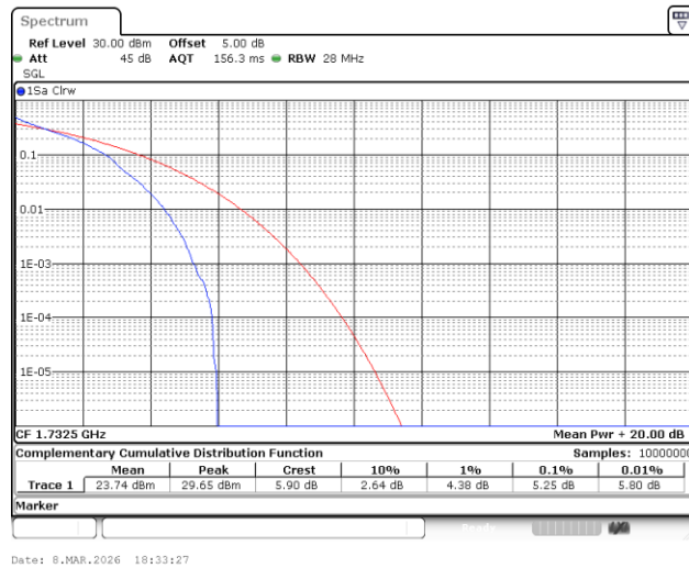
Band4-3MHz-QPSK-20175-1RB#0-PASS
