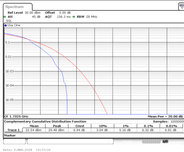
Band4-3MHz-16QAM-20175-1RB#0-PASS
