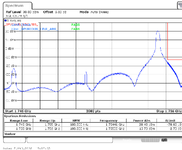
Band4-10MHz-16QAM-20350-1RB#49-PASS
