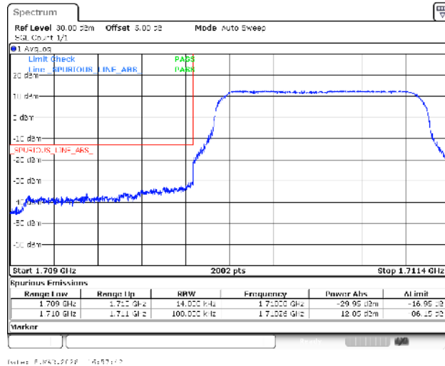
Band4-1.4MHz-QPSK-19957-6RB#0-PASS
