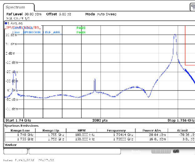
Band4-15MHz-16QAM-20325-1RB#74-PASS
