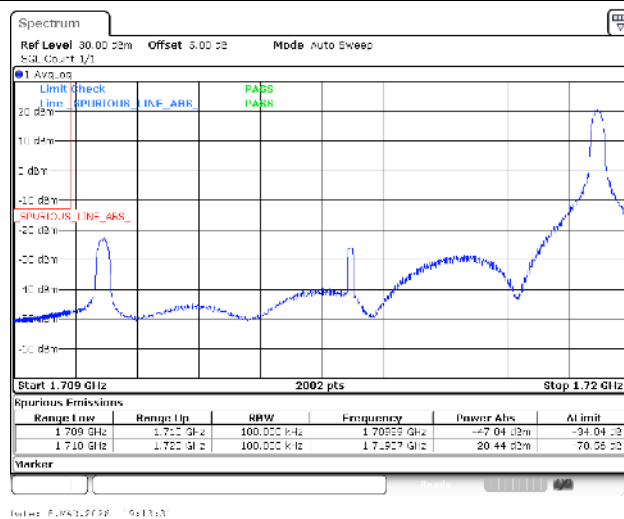
Band4-10MHz-16QAM-20000-1RB#49-PASS
