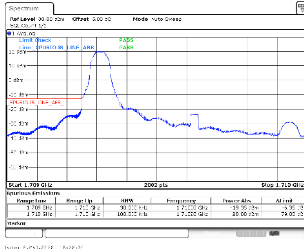
Band4-3MHz-16QAM-19965-1RB#0-PASS
