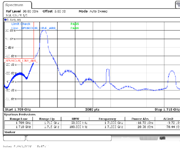
Band4-5MHz-16QAM-19975-1RB#0-PASS
