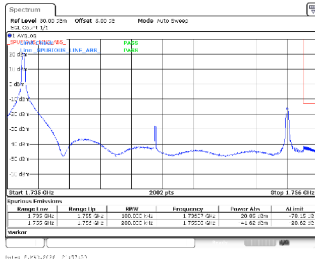
Band4-20MHz-16QAM-20300-1RB#0-PASS
