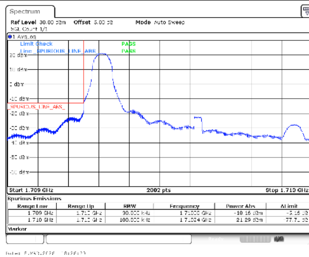
Band4-3MHz-QPSK-19965-1RB#0-PASS
