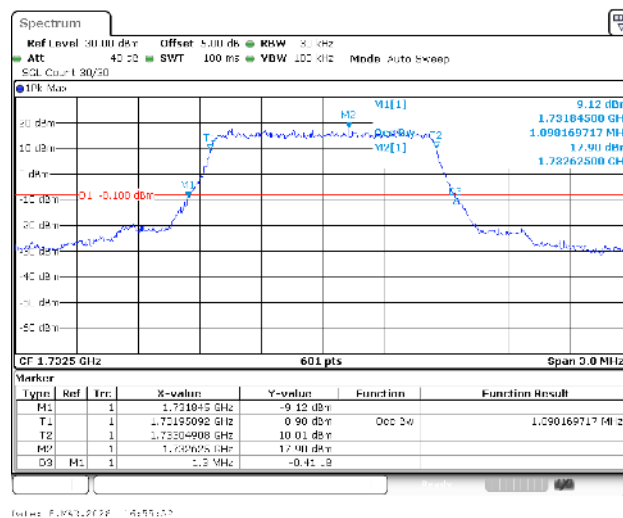
Band4-1.4MHz-QPSK-20175-6RB#0-PASS
