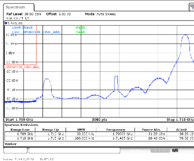
Band4-5MHz-16QAM-19975-1RB#24-PASS
