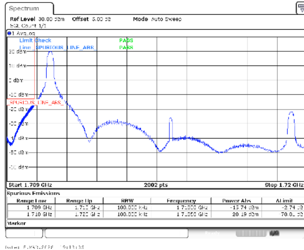
Band4-10MHz-16QAM-20000-1RB#0-PASS
