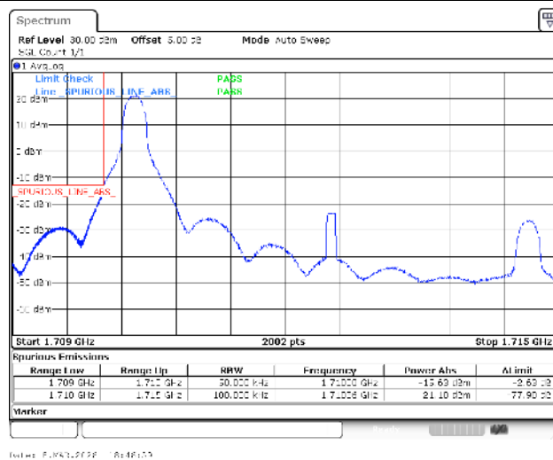
Band4-5MHz-QPSK-19975-1RB#0-PASS
