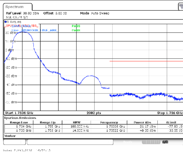
Band4-1.4MHz-QPSK-20393-1RB#0-PASS
