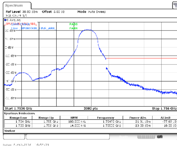
Band4-1.4MHz-QPSK-20393-1RB#5-PASS
