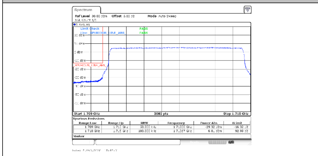
Band4-5MHz-16QAM-19975-25RB#0-PASS
