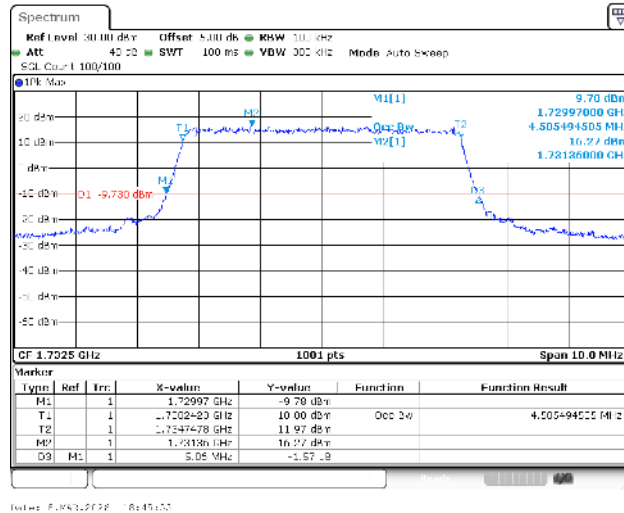
Band4-5MHz-16QAM-20175-25RB#0-PASS
