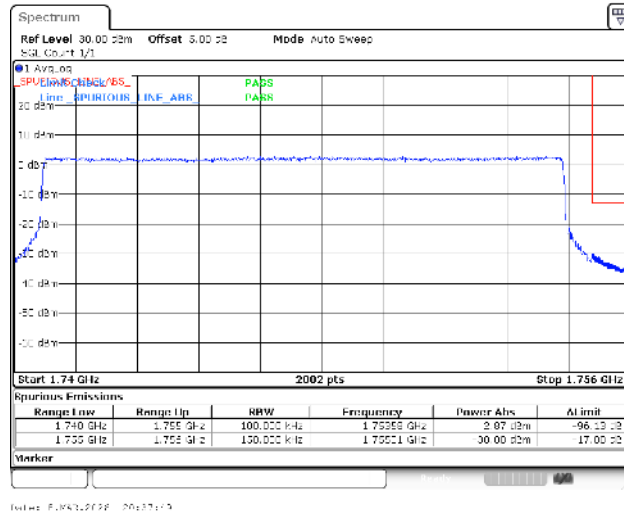
Band4-15MHz-QPSK-20325-75RB#0-PASS
