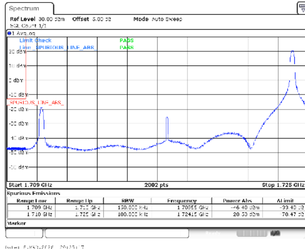
Band4-15MHz-16QAM-20025-1RB#74-PASS
