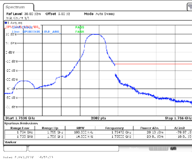
Band4-1.4MHz-16QAM-20393-1RB#5-PASS
