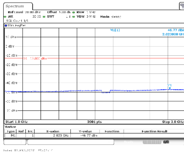
Band4-1.4MHz-QPSK-20175-1RB#0-1000~3000-PASS
