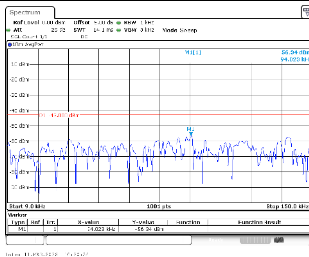
Band4-1.4MHz-QPSK-20175-1RB#0-0.009~0.15-PASS
