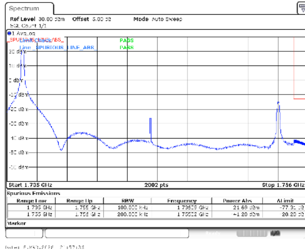
Band4-20MHz-QPSK-20300-1RB#0-PASS
