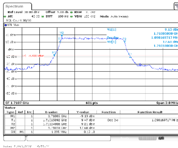
Band4-1.4MHz-QPSK-19957-6RB#0-PASS
