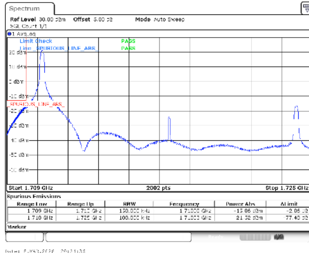
Band4-15MHz-QPSK-20025-1RB#0-PASS
