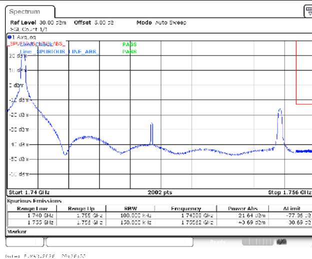
Band4-15MHz-QPSK-20325-1RB#0-PASS
