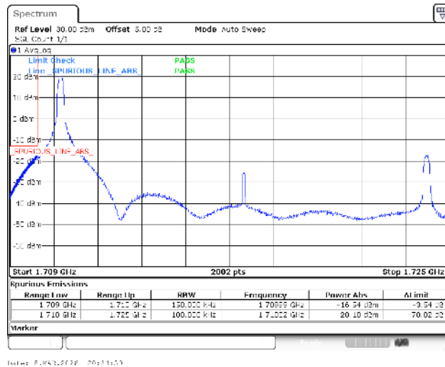
Band4-15MHz-16QAM-20025-1RB#0-PASS
