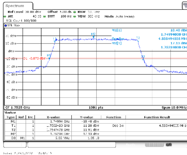
Band4-5MHz-QPSK-20375-25RB#0-PASS
