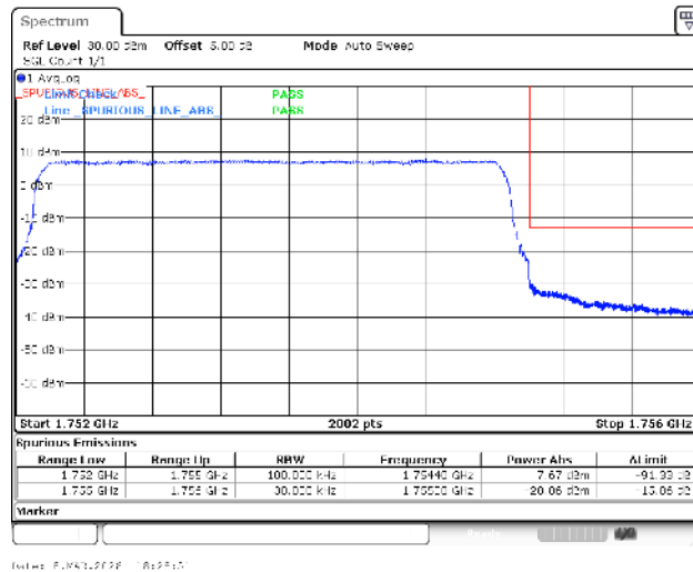
Band4-3MHz-16QAM-20385-15RB#0-PASS
