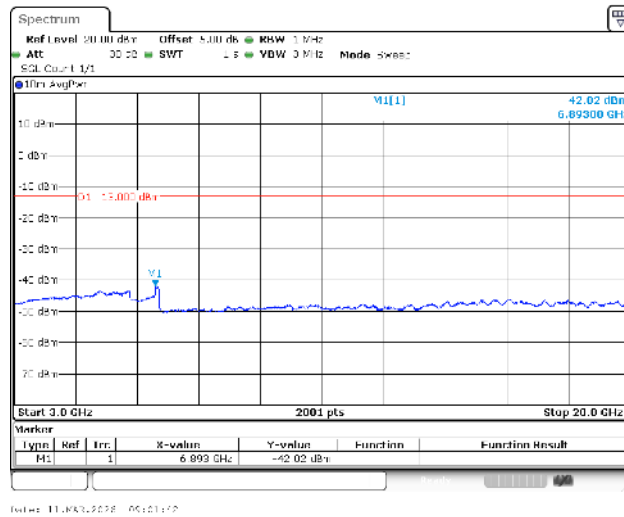
Band4-1.4MHz-16QAM-19957-1RB#0-3000~20000-PASS
