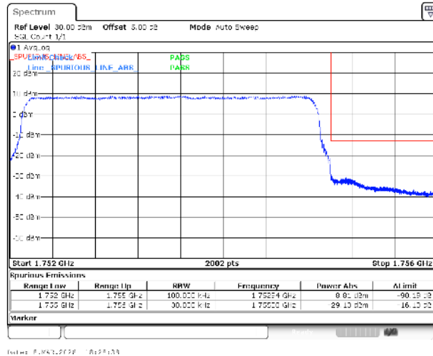
Band4-3MHz-QPSK-20385-15RB#0-PASS
