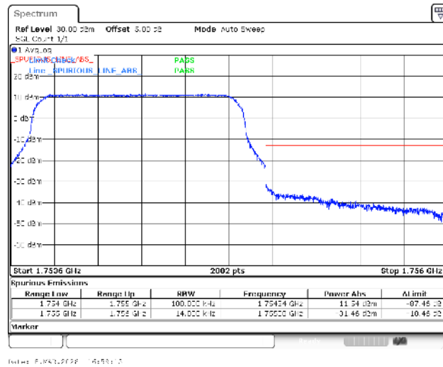
Band4-1.4MHz-16QAM-20393-6RB#0-PASS
