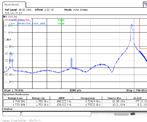
Band4-15MHz-QPSK-20325-1RB#74-PASS
