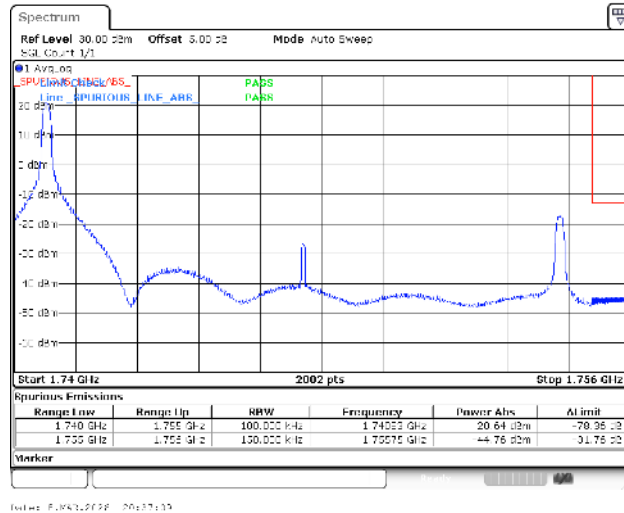
Band4-15MHz-16QAM-20325-1RB#0-PASS
