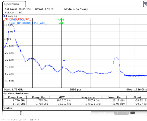
Band4-5MHz-16QAM-20375-1RB#0-PASS
