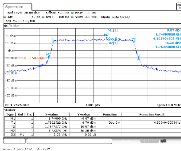
Band4-5MHz-16QAM-20375-25RB#0-PASS
