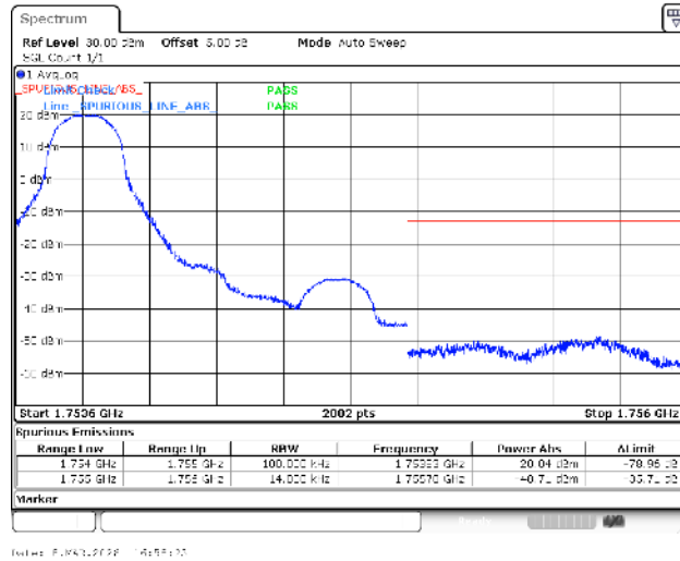
Band4-1.4MHz-16QAM-20393-1RB#0-PASS
