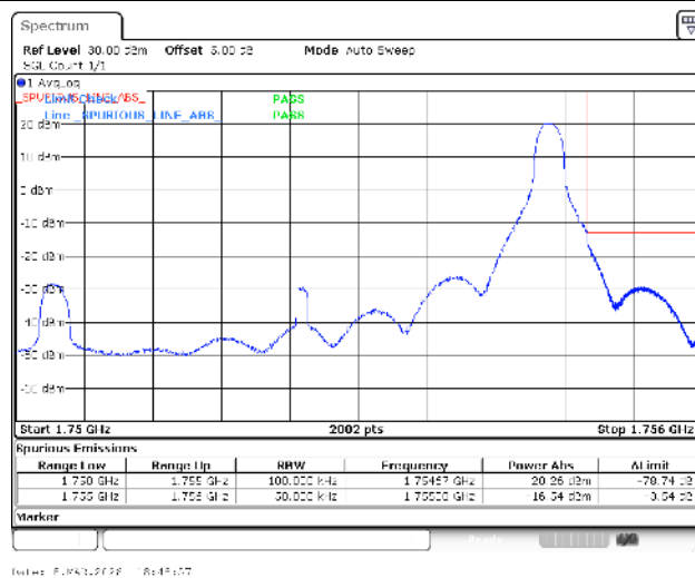
Band4-5MHz-16QAM-20375-1RB#24-PASS
