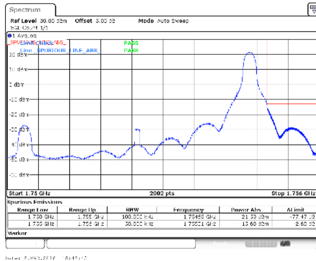
Band4-5MHz-QPSK-20375-1RB#24-PASS
