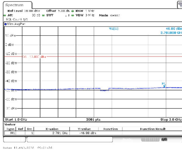
Band4-1.4MHz-16QAM-19957-1RB#0-1000~3000-PASS
