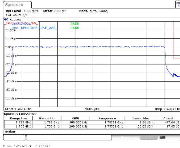
Band4-20MHz-QPSK-20300-100RB#0-PASS
