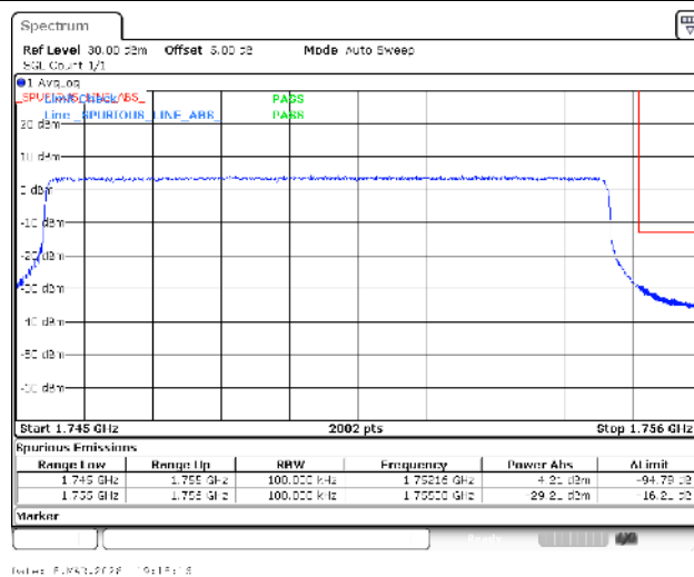
Band4-10MHz-QPSK-20350-50RB#0-PASS
