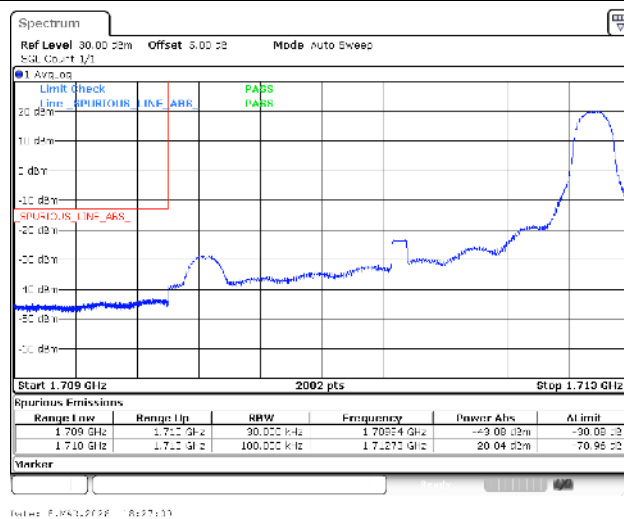
Band4-3MHz-16QAM-19965-1RB#14-PASS
