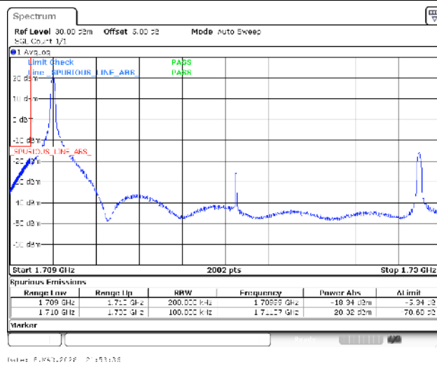
Band4-20MHz-16QAM-20050-1RB#0-PASS
