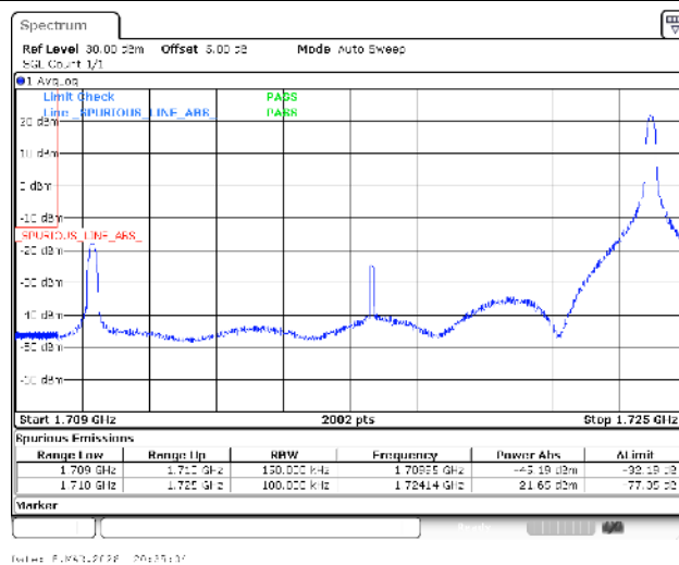
Band4-15MHz-QPSK-20025-1RB#74-PASS
