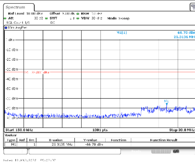
Band4-1.4MHz-QPSK-20175-1RB#0-0.15~30-PASS
