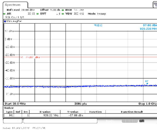
Band4-1.4MHz-QPSK-20175-1RB#0-30~1000-PASS
