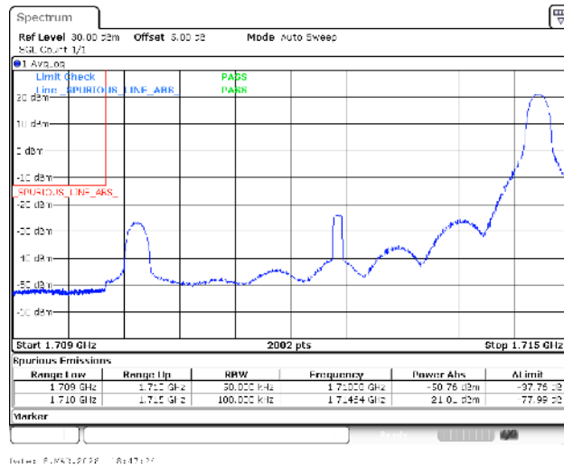
Band4-5MHz-QPSK-19975-1RB#24-PASS
