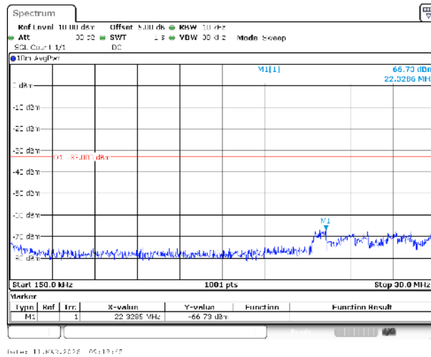
Band4-20MHz-16QAM-20050-1RB#0-0.15~30-PASS
