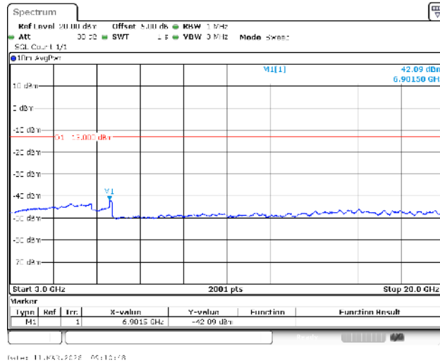
Band4-5MHz-QPSK-20375-1RB#0-3000~20000-PASS
