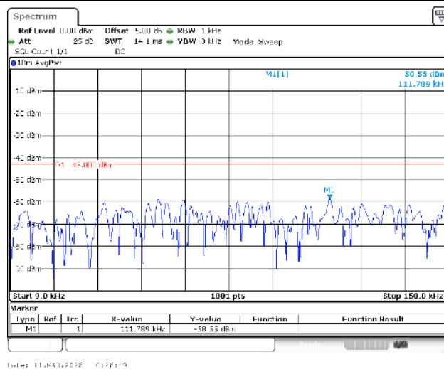
Band4-15MHz-QPSK-20025-1RB#0-0.009~0.15-PASS
