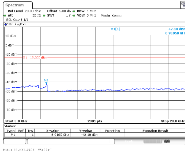
Band4-20MHz-QPSK-20175-1RB#0-3000~20000-PASS
