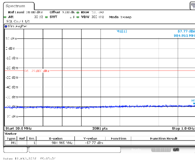
Band4-15MHz-QPSK-20025-1RB#0-30~1000-PASS
