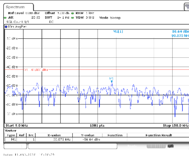
Band4-15MHz-16QAM-20025-1RB#0-0.009~0.15-PASS
