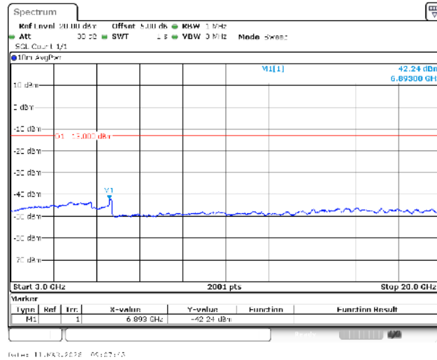
Band4-3MHz-16QAM-20385-1RB#0-3000~20000-PASS
