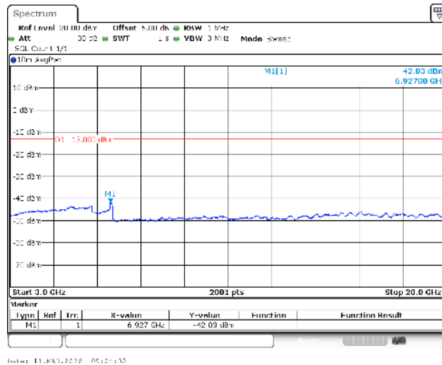
Band4-1.4MHz-16QAM-20393-1RB#0-3000~20000-PASS
