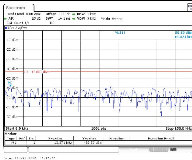
Band4-15MHz-16QAM-20175-1RB#0-0.009~0.15-PASS
