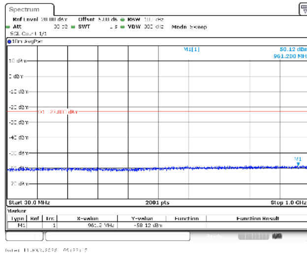
Band4-20MHz-16QAM-20300-1RB#0-30~1000-PASS
