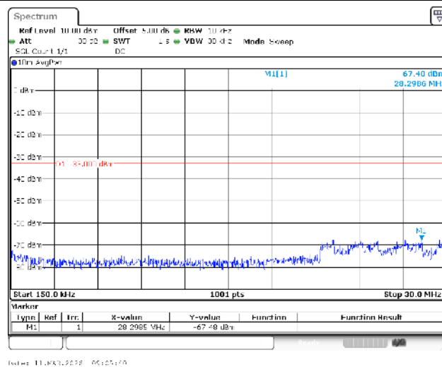
Band4-3MHz-QPSK-20175-1RB#0-0.15~30-PASS
