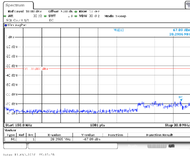
Band4-15MHz-QPSK-20025-1RB#0-0.15~30-PASS
