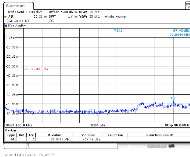
Band4-5MHz-QPSK-19975-1RB#0-0.15~30-PASS
