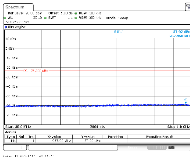
Band4-20MHz-16QAM-20050-1RB#0-30~1000-PASS
