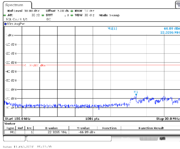
Band4-20MHz-16QAM-20300-1RB#0-0.15~30-PASS
