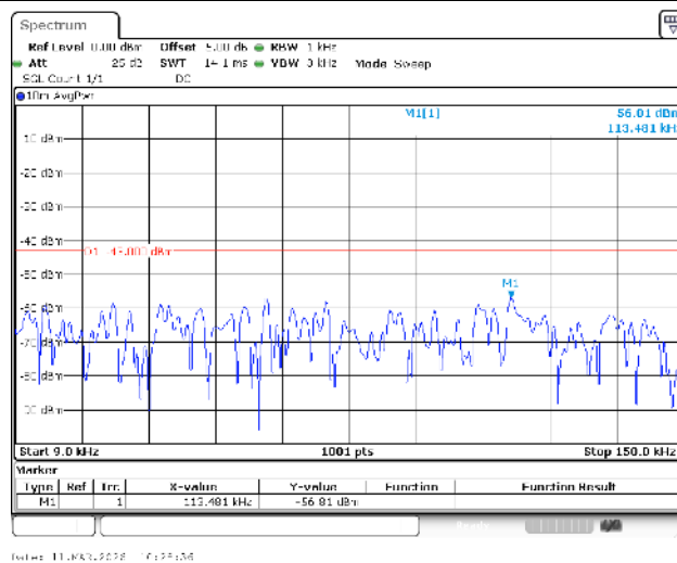
Band4-20MHz-16QAM-20175-1RB#0-0.009~0.15-PASS
