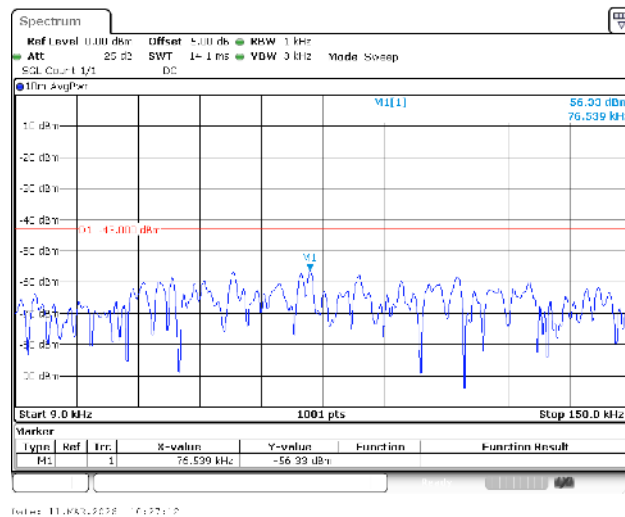
Band4-15MHz-QPSK-20175-1RB#0-0.009~0.15-PASS
