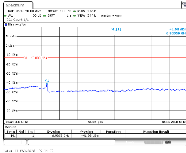
Band4-10MHz-QPSK-20350-1RB#0-3000~20000-PASS
