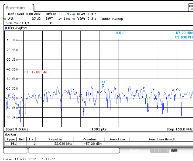
Band4-3MHz-QPSK-19965-1RB#0-0.009~0.15-PASS
