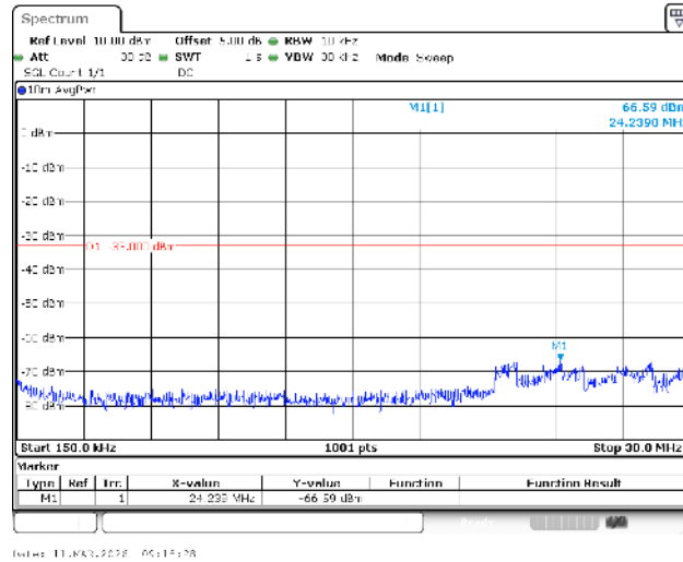
Band4-15MHz-16QAM-20325-1RB#0-0.15~30-PASS
