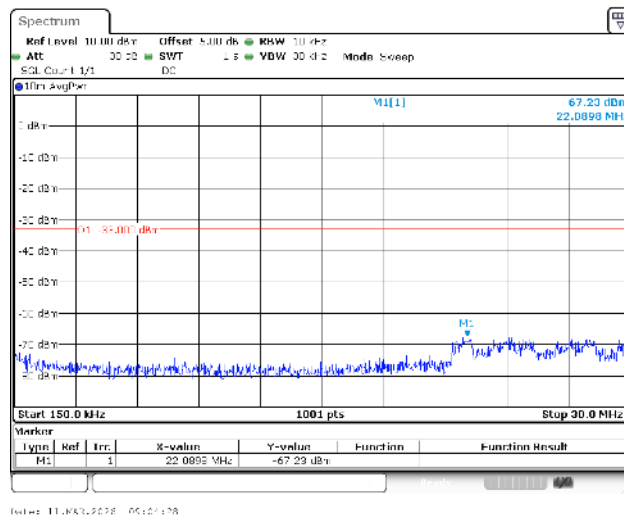
Band4-3MHz-QPSK-19965-1RB#0-0.15~30-PASS
