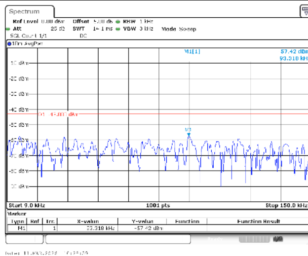
Band4-20MHz-16QAM-20300-1RB#0-0.009~0.15-PASS
