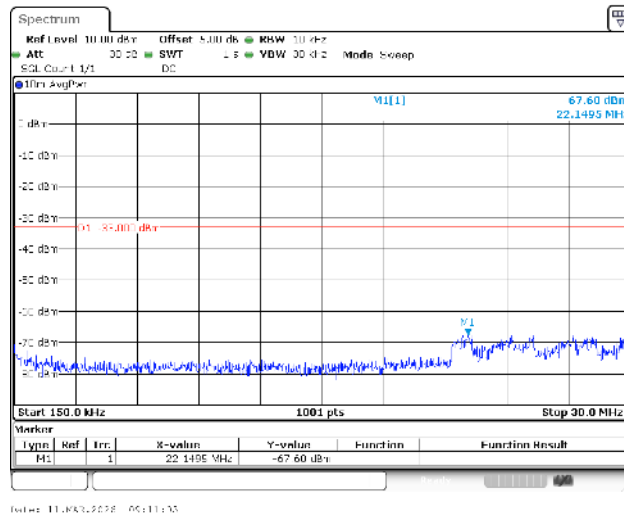
Band4-5MHz-16QAM-20375-1RB#0-0.15~30-PASS
