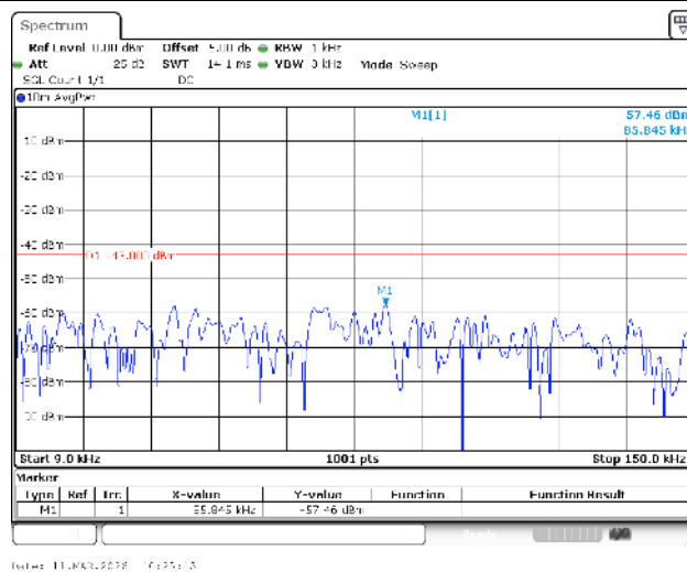
Band4-5MHz-16QAM-20375-1RB#0-0.009~0.15-PASS
