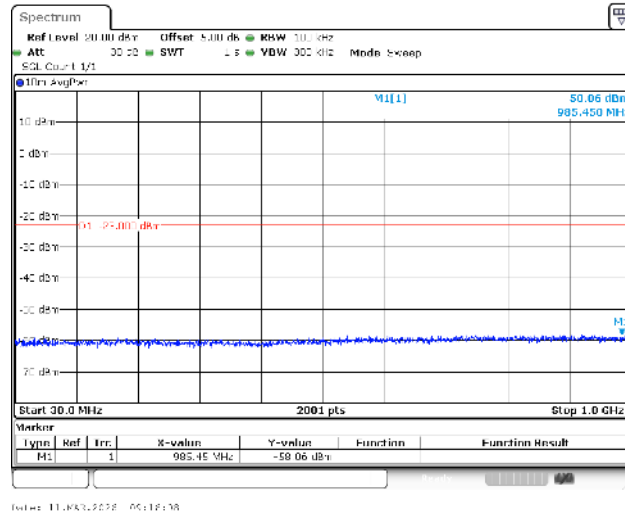
Band4-15MHz-16QAM-20025-1RB#0-30~1000-PASS
