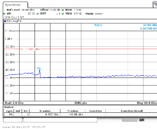
Band4-3MHz-16QAM-19965-1RB#0-3000~20000-PASS
