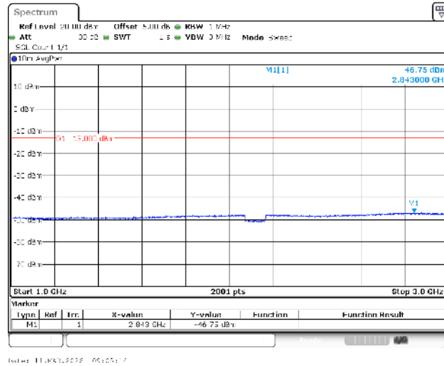
Band4-3MHz-16QAM-19965-1RB#0-1000~3000-PASS
