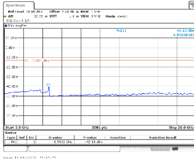
Band4-20MHz-QPSK-20050-1RB#0-3000~20000-PASS
