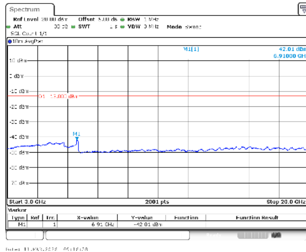
Band4-15MHz-QPSK-20175-1RB#0-3000~20000-PASS
