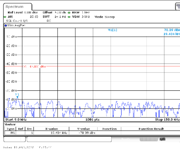
Band4-5MHz-QPSK-19975-1RB#0-0.009~0.15-PASS
