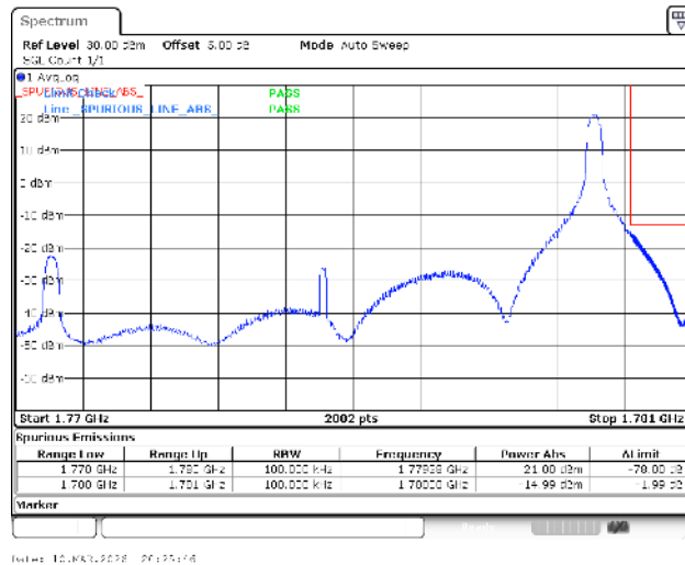
Band66-10MHz-16QAM-132622-1RB#49-PASS
