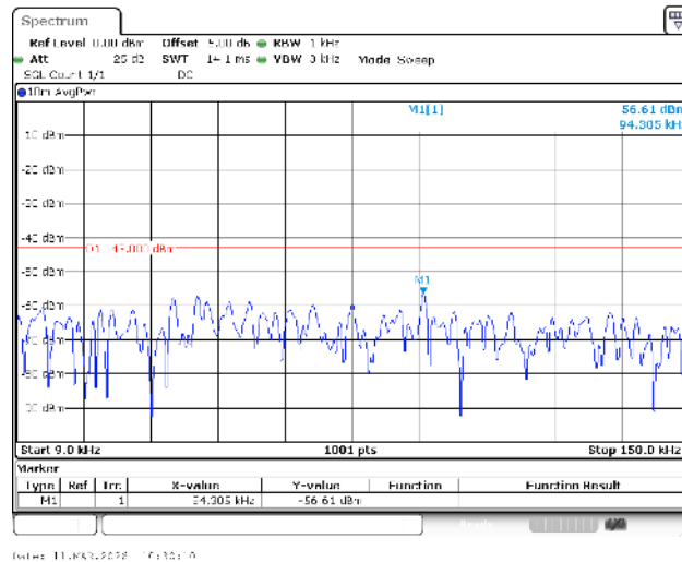
Band66-1.4MHz-16QAM-132322-1RB#0-0.009~0.15-PASS
