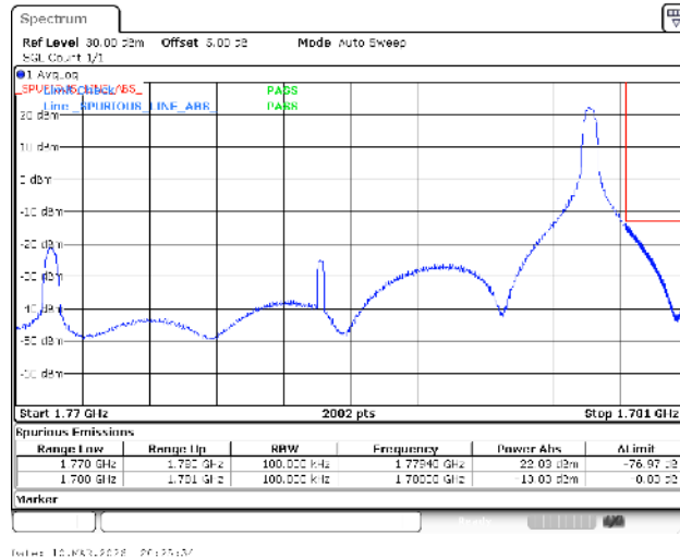
Band66-10MHz-QPSK-132622-1RB#49-PASS
