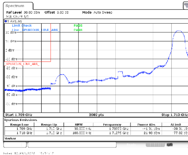
Band66-3MHz-QPSK-131987-1RB#14-PASS
