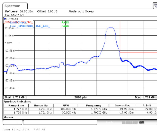
Band66-3MHz-16QAM-132657-1RB#14-PASS
