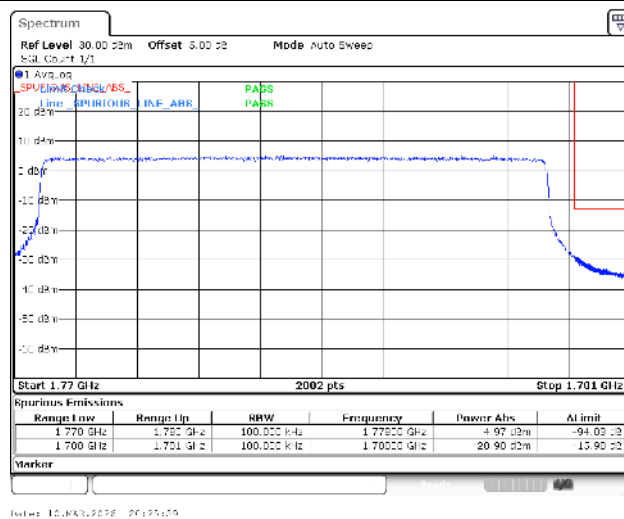
Band66-10MHz-QPSK-132622-50RB#0-PASS
