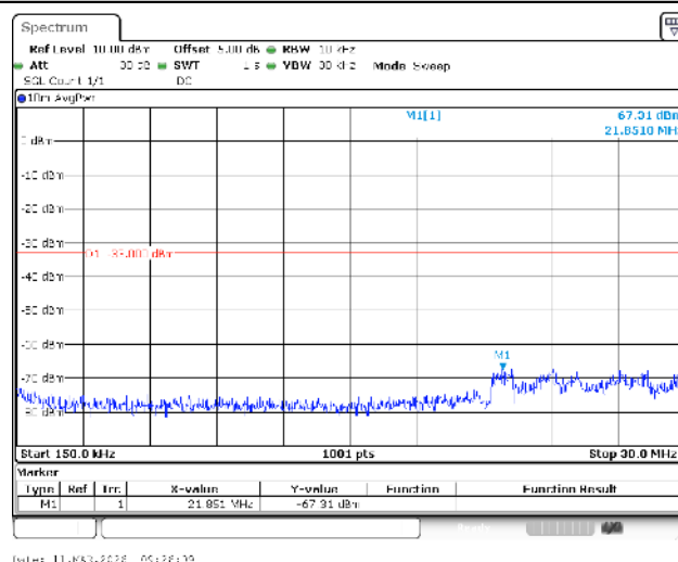
Band66-1.4MHz-16QAM-132665-1RB#0-0.15~30-PASS
