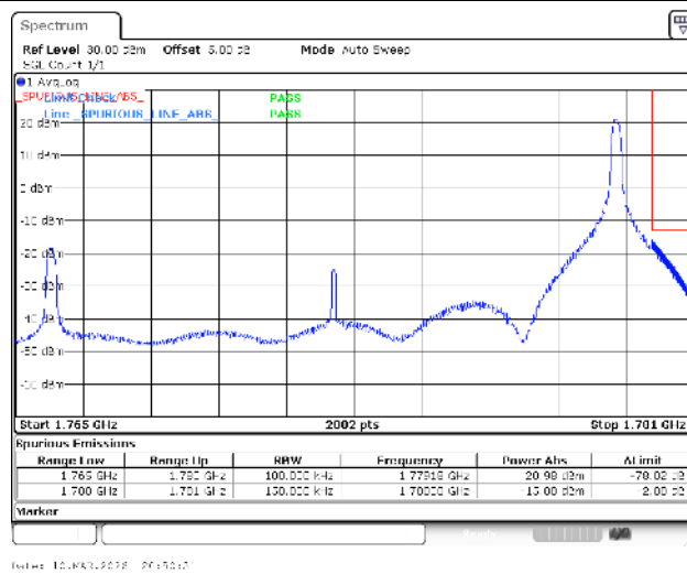
Band66-15MHz-16QAM-132597-1RB#74-PASS
