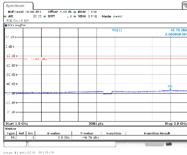
Band66-1.4MHz-16QAM-131979-1RB#0-1000~3000-PASS
