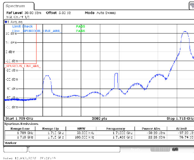
Band66-5MHz-QPSK-131997-1RB#24-PASS
