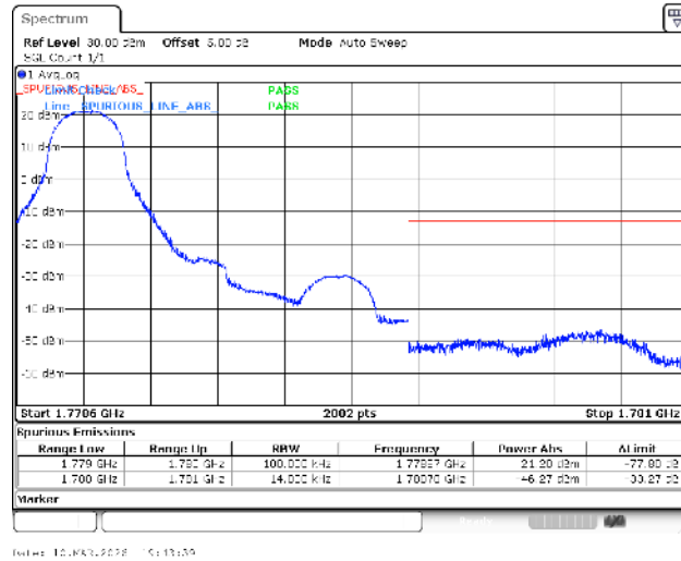
Band66-1.4MHz-16QAM-132665-1RB#0-PASS
