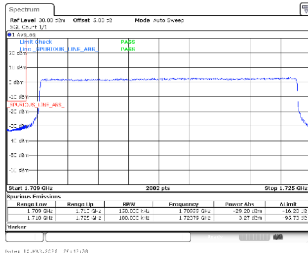
Band66-15MHz-QPSK-132047-75RB#0-PASS
