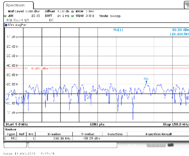
Band66-1.4MHz-16QAM-131979-1RB#0-0.009~0.15-PASS
