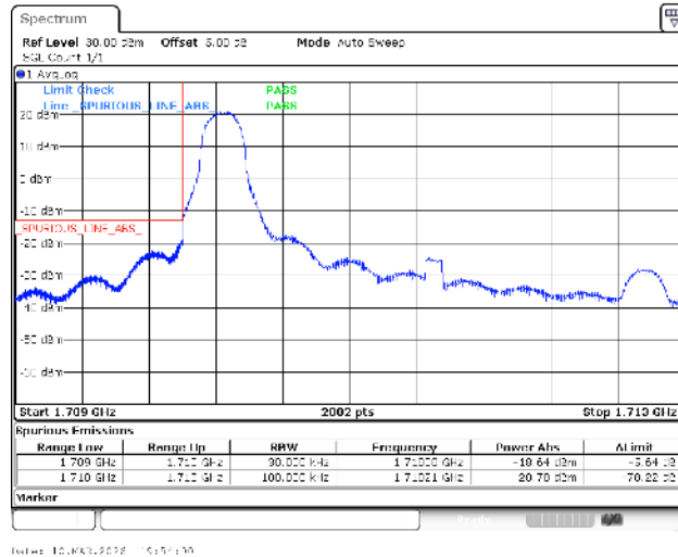
Band66-3MHz-16QAM-131987-1RB#0-PASS
