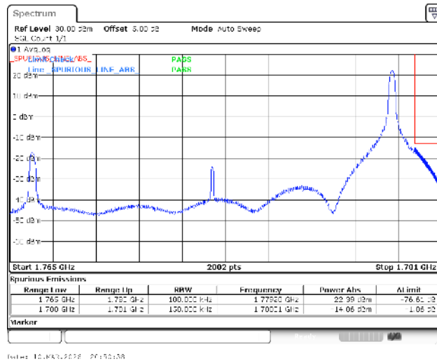
Band66-15MHz-QPSK-132597-1RB#74-PASS
