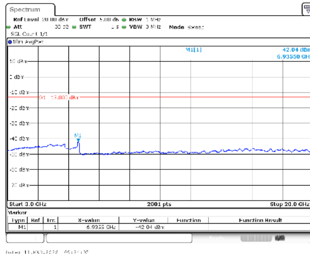
Band66-1.4MHz-16QAM-131979-1RB#0-3000~20000-PASS
