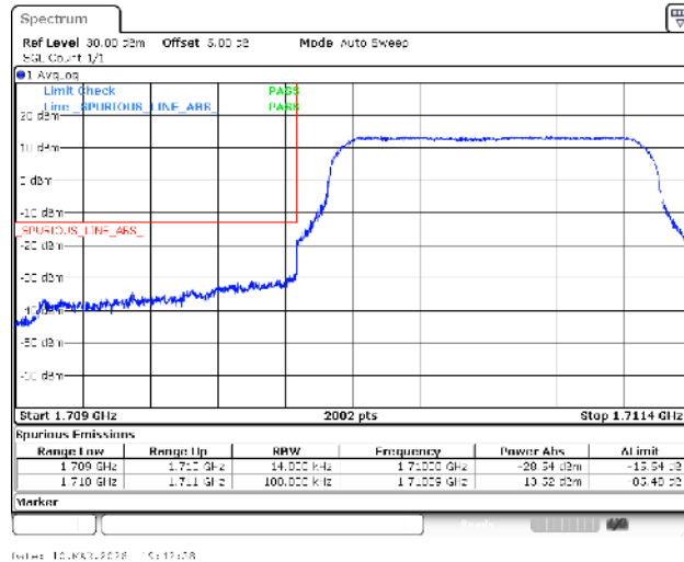
Band66-1.4MHz-QPSK-131979-6RB#0-PASS
