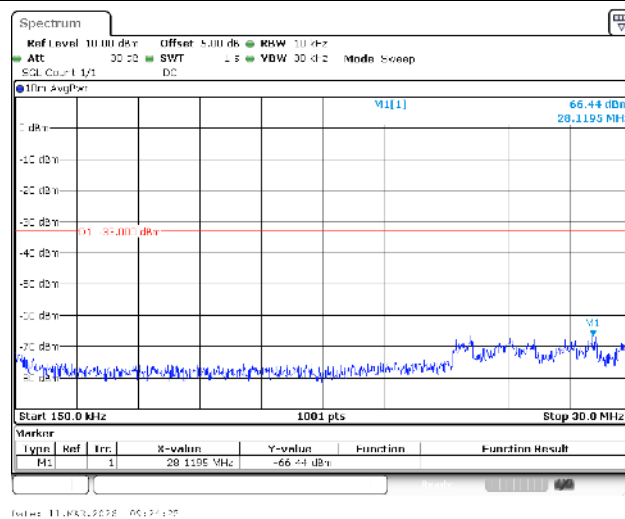
Band66-1.4MHz-QPSK-132322-1RB#0-0.15~30-PASS
