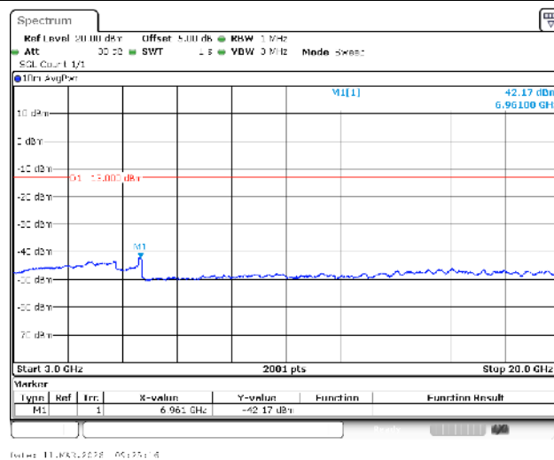
Band66-1.4MHz-16QAM-132322-1RB#0-3000~20000-PASS
