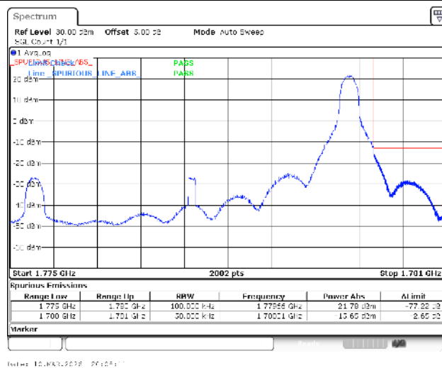
Band66-5MHz-16QAM-132647-1RB#24-PASS
