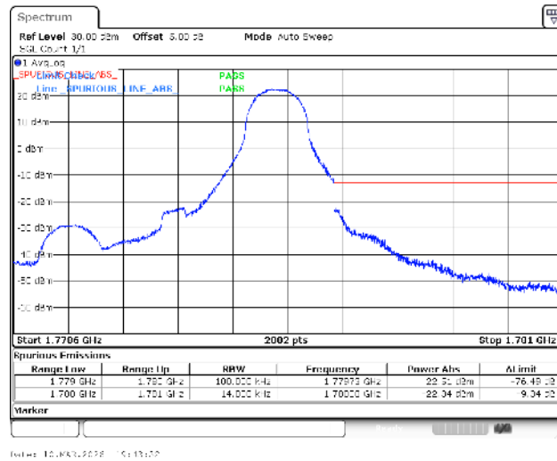
Band66-1.4MHz-QPSK-132665-1RB#5-PASS
