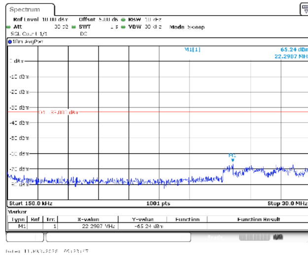
Band66-1.4MHz-16QAM-131979-1RB#0-0.15~30-PASS
