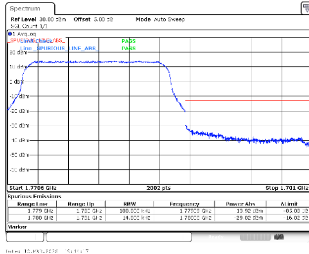
Band66-1.4MHz-QPSK-132665-6RB#0-PASS
