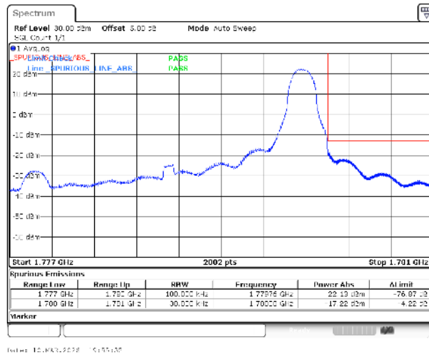
Band66-3MHz-QPSK-132657-1RB#14-PASS
