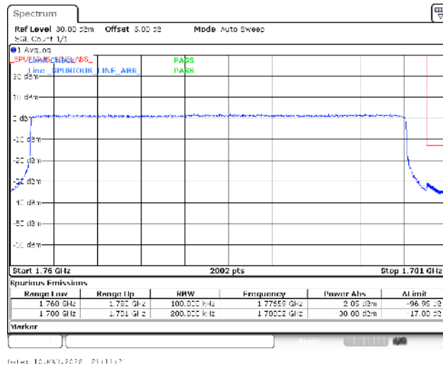
Band66-20MHz-QPSK-132572-100RB#0-PASS
