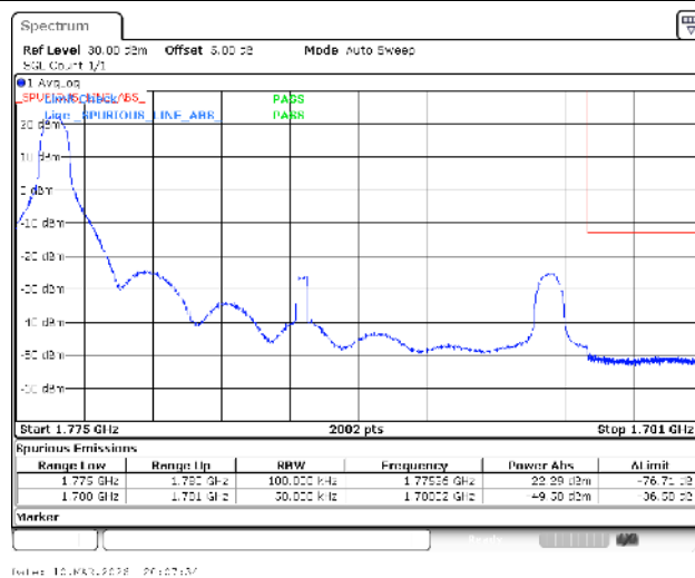
Band66-5MHz-QPSK-132647-1RB#0-PASS
