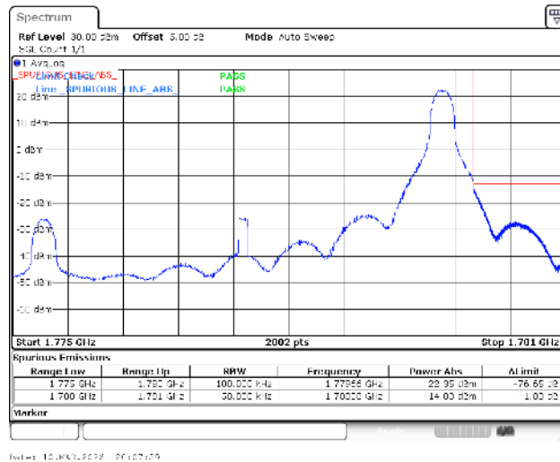
Band66-5MHz-QPSK-132647-1RB#24-PASS
