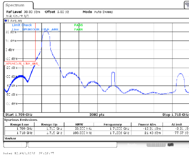
Band66-5MHz-16QAM-131997-1RB#0-PASS
