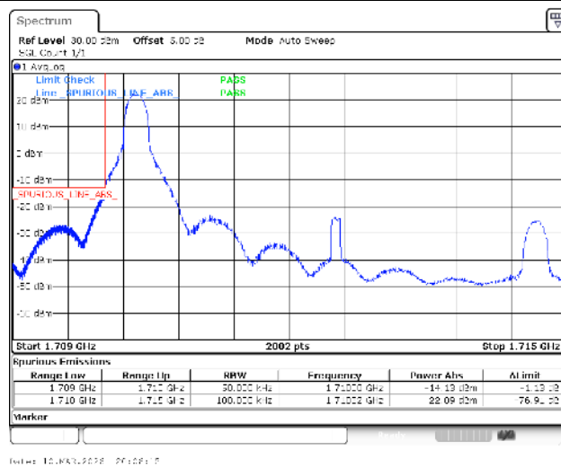
Band66-5MHz-QPSK-131997-1RB#0-PASS
