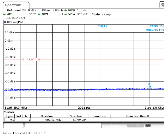
Band66-1.4MHz-QPSK-132322-1RB#0-30~1000-PASS
