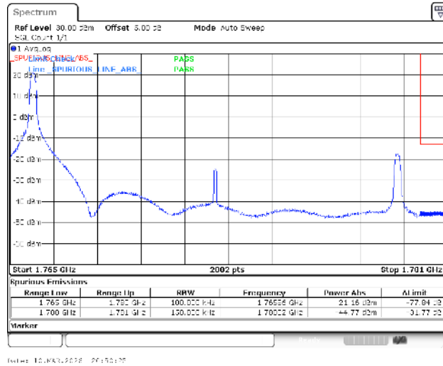
Band66-15MHz-16QAM-132597-1RB#0-PASS
