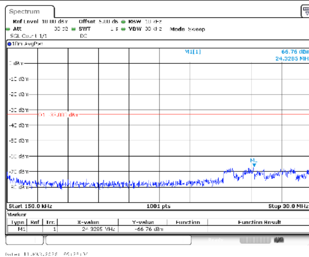
Band66-3MHz-QPSK-132322-1RB#0-0.15~30-PASS
