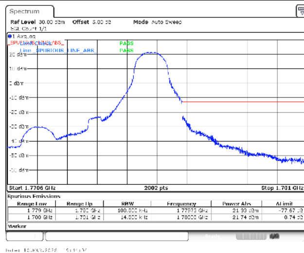
Band66-1.4MHz-16QAM-132665-1RB#5-PASS
