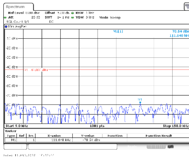
Band66-1.4MHz-QPSK-132665-1RB#0-0.009~0.15-PASS
