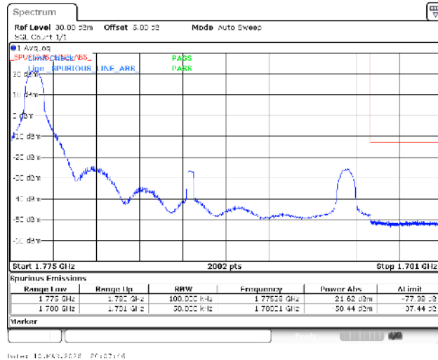
Band66-5MHz-16QAM-132647-1RB#0-PASS
