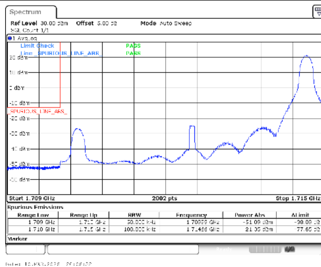
Band66-5MHz-16QAM-131997-1RB#24-PASS
