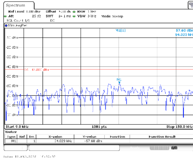
Band66-1.4MHz-QPSK-132322-1RB#0-0.009~0.15-PASS
