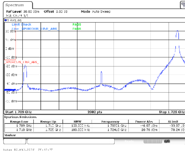
Band66-15MHz-16QAM-132047-1RB#74-PASS
