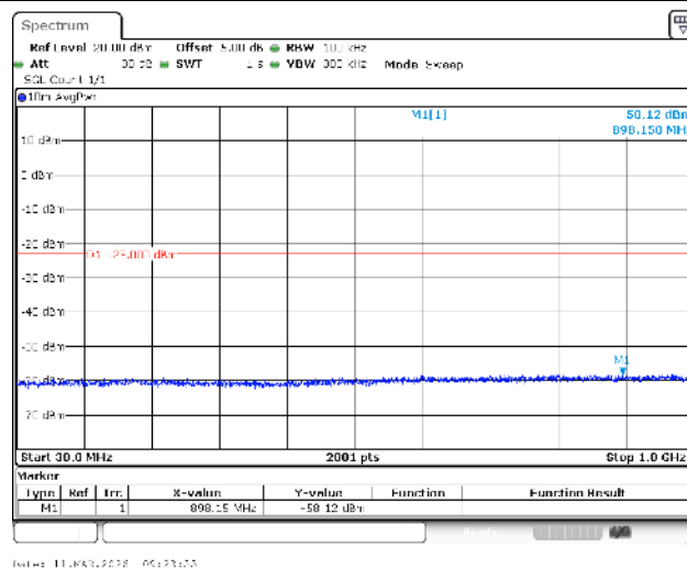
Band66-1.4MHz-16QAM-131979-1RB#0-30~1000-PASS
