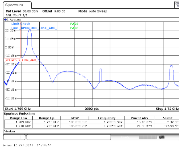
Band66-10MHz-16QAM-132022-1RB#0-PASS
