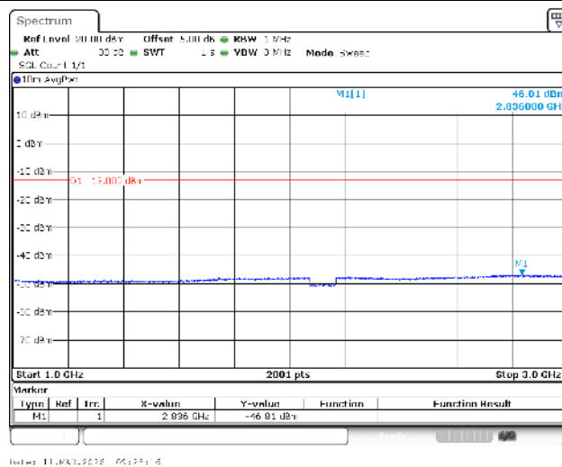
Band66-3MHz-QPSK-132322-1RB#0-1000~3000-PASS
