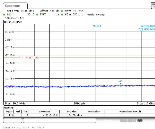
Band66-3MHz-QPSK-131987-1RB#0-30~1000-PASS
