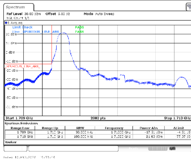
Band66-3MHz-QPSK-131987-1RB#0-PASS
