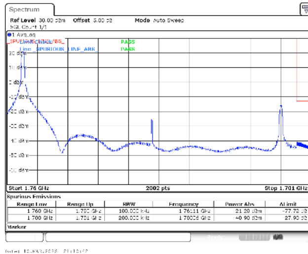
Band66-20MHz-16QAM-132572-1RB#0-PASS
