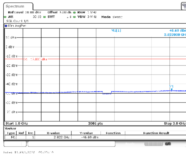
Band66-1.4MHz-16QAM-132322-1RB#0-1000~3000-PASS
