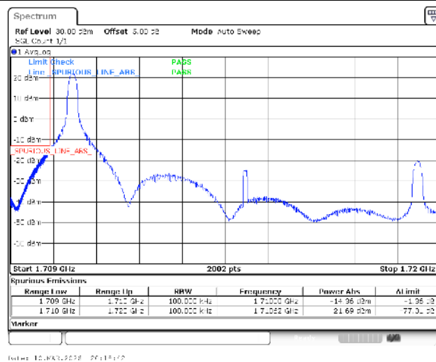
Band66-10MHz-QPSK-132022-1RB#0-PASS
