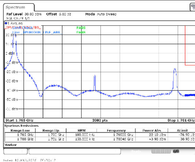
Band66-15MHz-QPSK-132597-1RB#0-PASS
