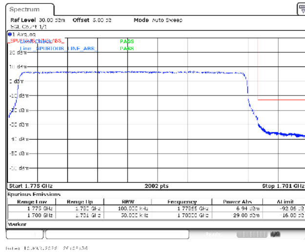
Band66-5MHz-16QAM-132647-25RB#0-PASS
