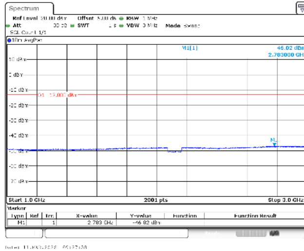
Band66-3MHz-16QAM-131987-1RB#0-1000~3000-PASS
