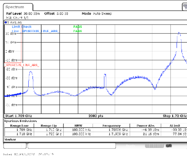
Band66-10MHz-16QAM-132022-1RB#49-PASS
