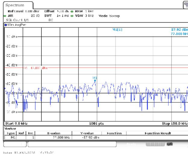
Band66-3MHz-QPSK-132322-1RB#0-0.009~0.15-PASS
