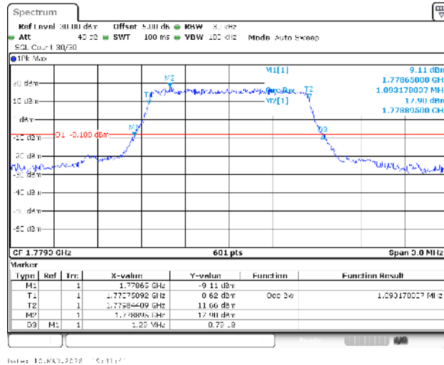
Band66-1.4MHz-16QAM-132665-6RB#0-PASS
