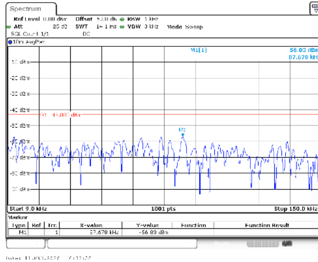
Band66-1.4MHz-16QAM-132665-1RB#0-0.009~0.15-PASS
