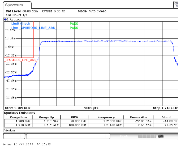
Band66-5MHz-QPSK-131997-25RB#0-PASS
