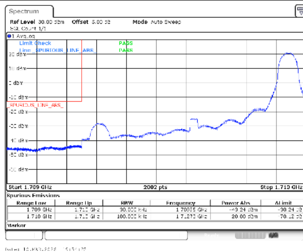
Band66-3MHz-16QAM-131987-1RB#14-PASS
