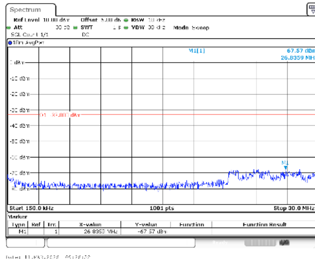
Band66-3MHz-QPSK-131987-1RB#0-0.15~30-PASS
