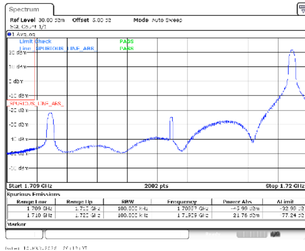
Band66-10MHz-QPSK-132022-1RB#49-PASS
