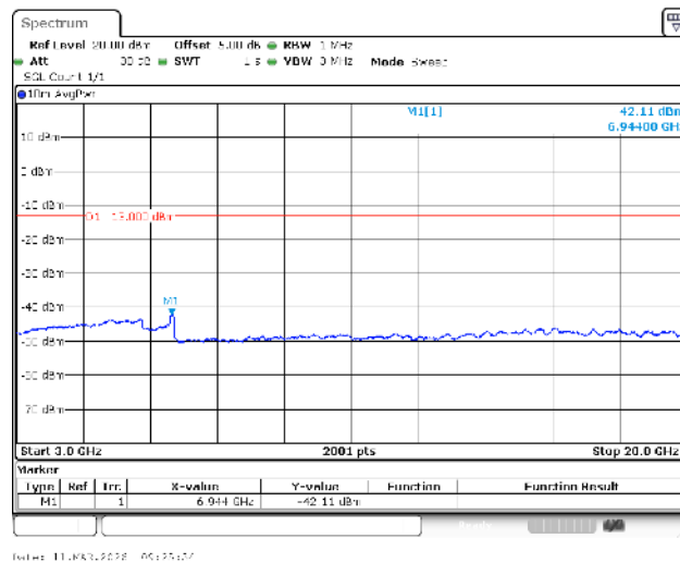
Band66-1.4MHz-QPSK-132665-1RB#0-3000~20000-PASS
