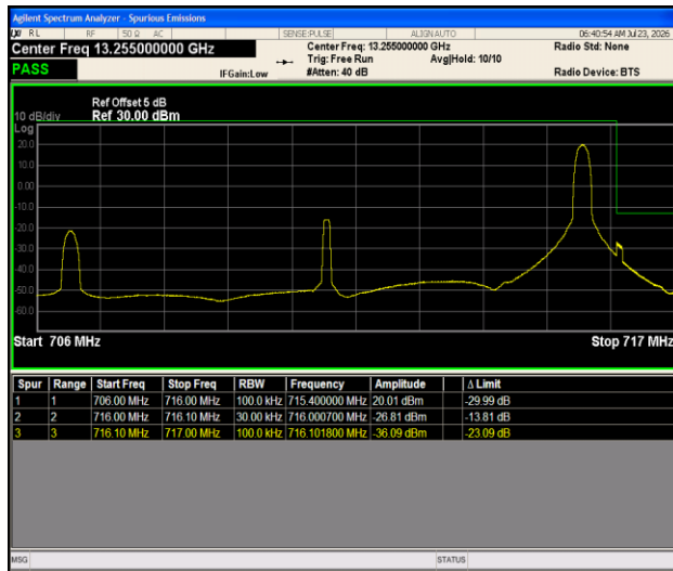
Band12-10MHz-QPSK-23130-1RB#49-PASS
