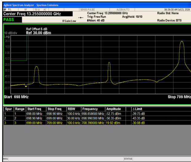
Band12-10MHz-QPSK-23060-1RB#49-PASS
