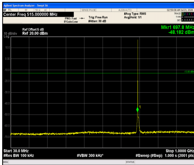
Band12-1.4MHz- 16QAM-23017-1RB#0-30~1000-PASS
