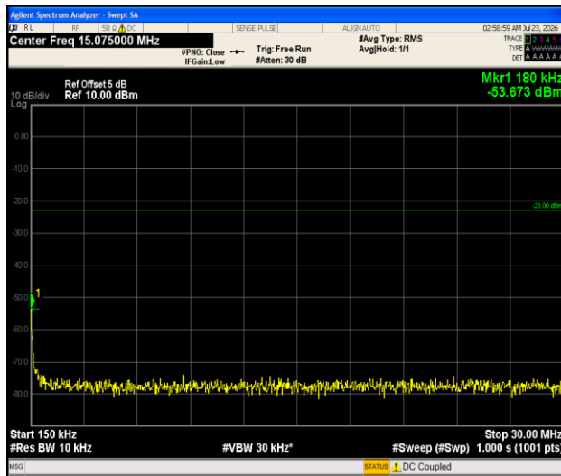
Band12-1.4MHz- 16QAM-23017-1RB#0-0.15~30-PASS
