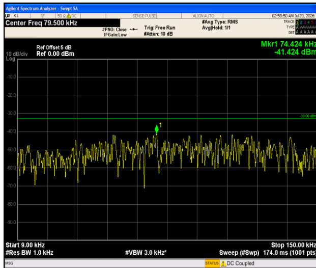
Band12-1.4MHz- 16QAM-23017-1RB#0-0.009~0.15-PASS
