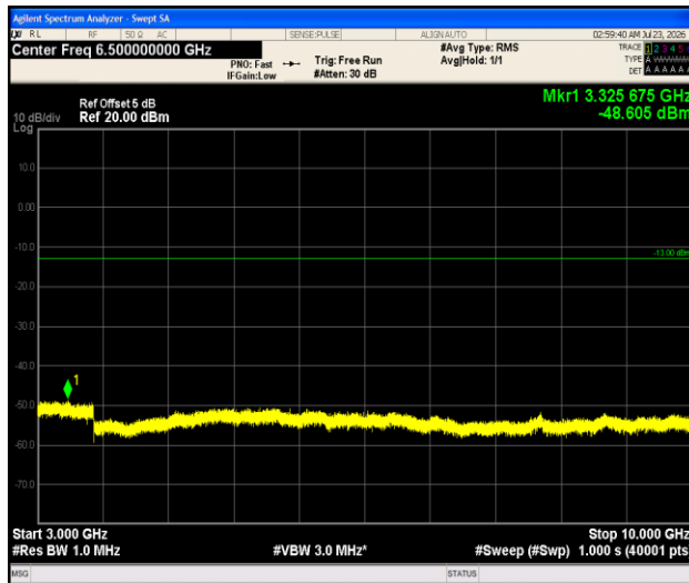
Band12-1.4MHz- 16QAM-23017-1RB#0-3000~10000-PASS
