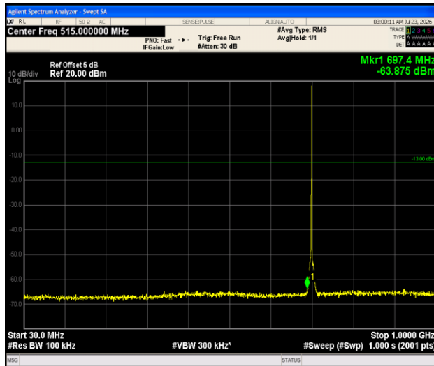
Band12-1.4MHz-QPSK-23095-1RB#0-30~1000-PASS
