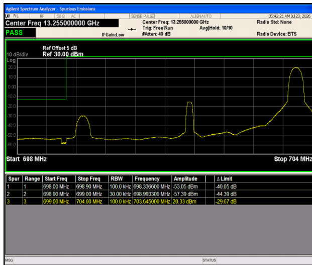
Band12-5MHz-QPSK-23035-1RB#24-PASS
