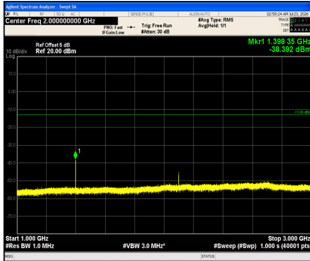
Band12-1.4MHz- 16QAM-23017-1RB#0-1000~3000-PASS
