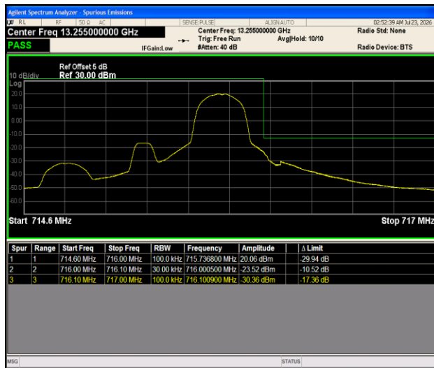
Band12-1.4MHz-QPSK-23173-1RB#5-PASS
