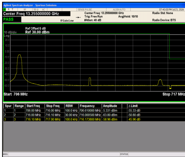
Band12-10MHz-16QAM-23130-1RB#0-PASS
