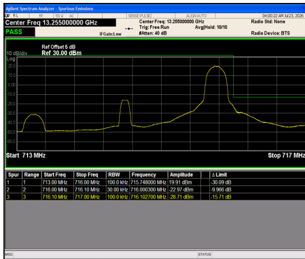
Band12-3MHz-QPSK-23165-1RB#14-PASS
