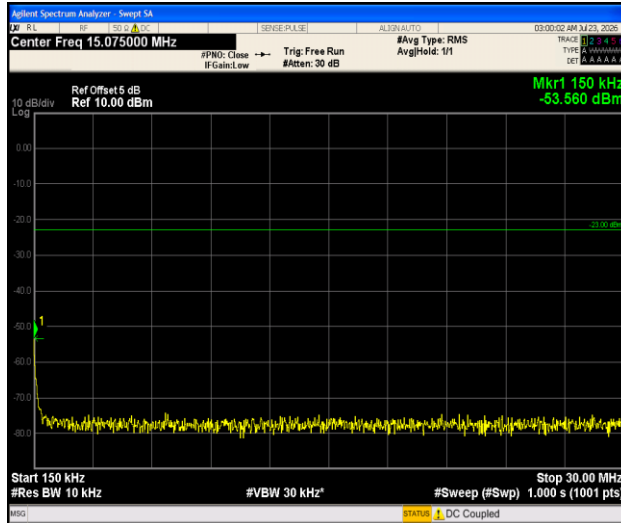
Band12-1.4MHz-QPSK-23095-1RB#0-0.15~30-PASS
