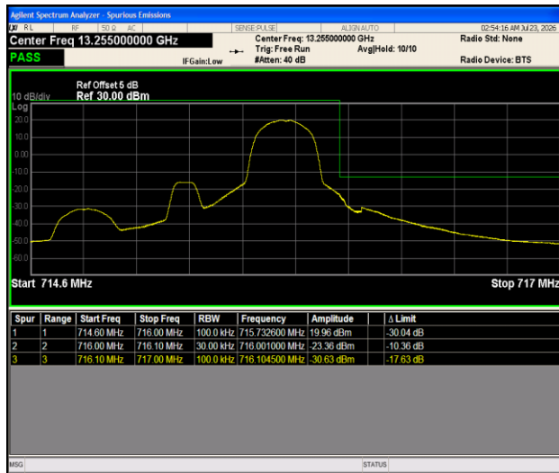
Band12-1.4MHz- 16QAM-23173-1RB#5-PASS
