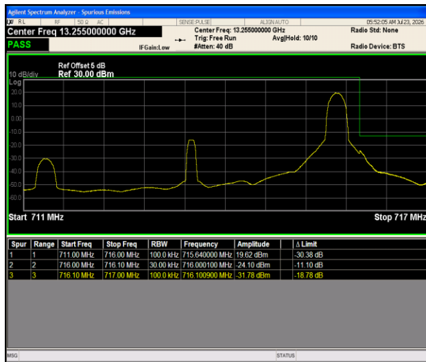
Band12-5MHz-QPSK-23155-1RB#24-PASS
