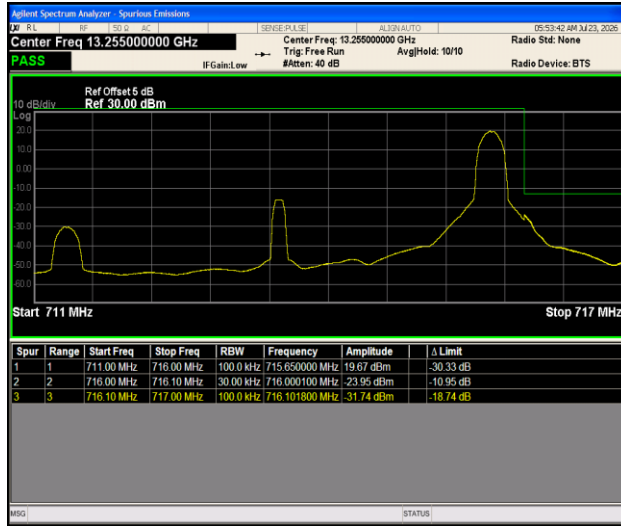
Band12-5MHz- 16QAM-23155-1RB#24-PASS
