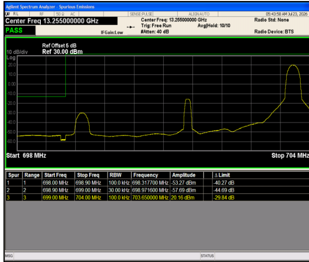
Band12-5MHz- 16QAM-23035-1RB#24-PASS
