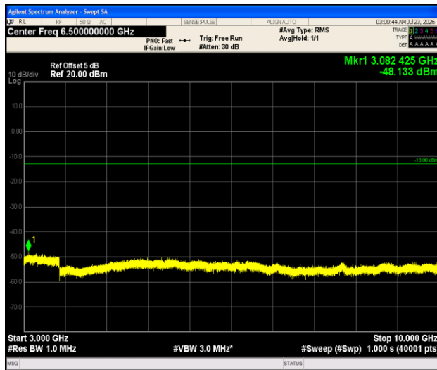
Band12-1.4MHz-QPSK-23095-1RB#0-3000~10000-PASS
