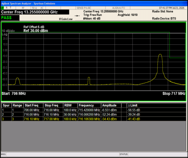
Band12-10MHz-16QAM-23130-1RB#49-PASS
