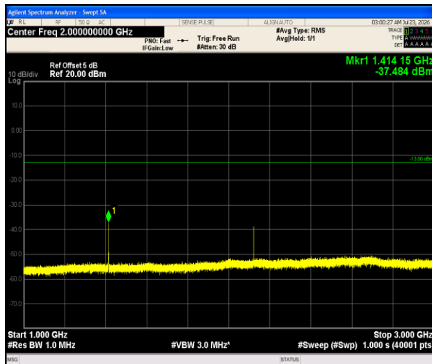
Band12-1.4MHz-QPSK-23095-1RB#0-1000~3000-PASS
