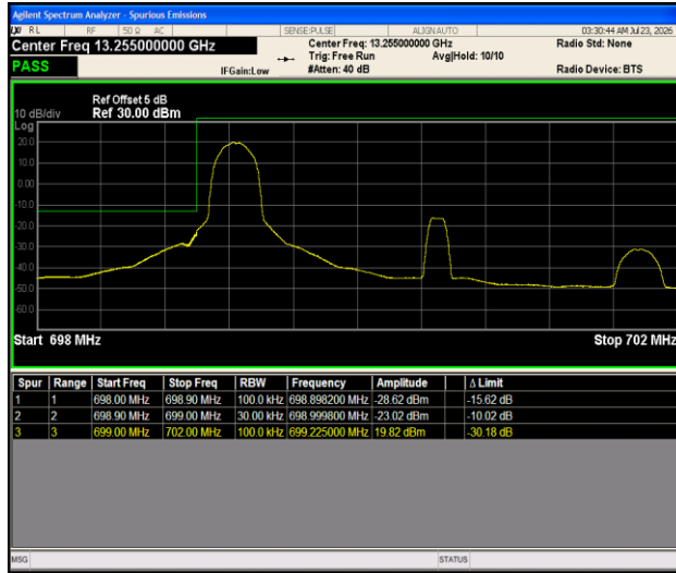
Band12-3MHz-QPSK-23025-1RB#0-PASS
