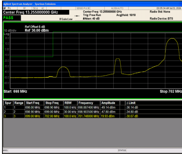
Band12-3MHz- 16QAM-23025-1RB#14-PASS
