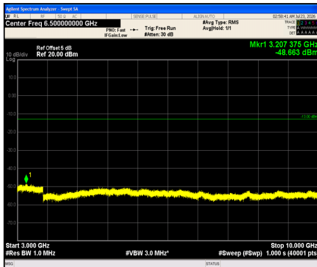
Band12-1.4MHz-QPSK-23017-1RB#0-3000~10000-PASS
