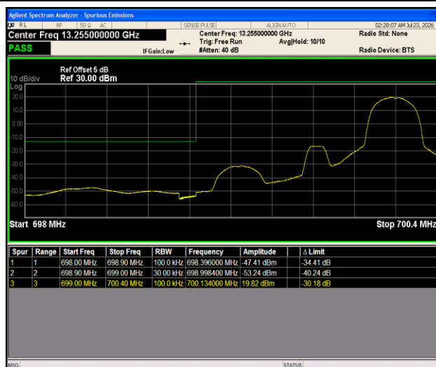
Band12-1.4MHz- 16QAM-23017-1RB#0-PASS
