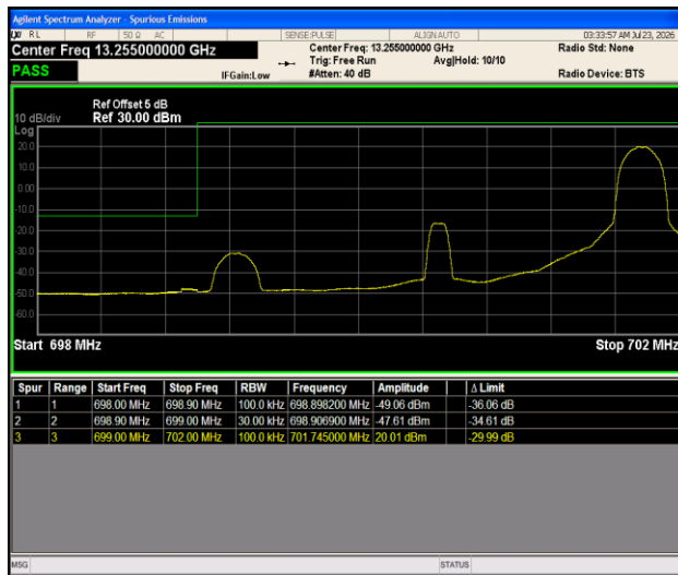
Band12-3MHz-QPSK-23025-1RB#14-PASS
