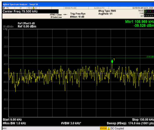
Band12-1.4MHz-QPSK-23095-1RB#0-0.009~0.15-PASS
