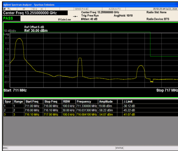
Band12-5MHz- 16QAM-23155-1RB#0-PASS
