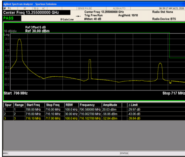
Band12-10MHz-QPSK-23130-1RB#0-PASS
