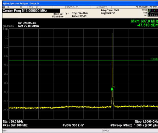
Band12-1.4MHz-QPSK-23017-1RB#0-30~1000-PASS
