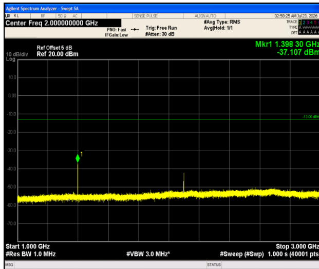
Band12-1.4MHz-QPSK-23017-1RB#0-1000~3000-PASS
