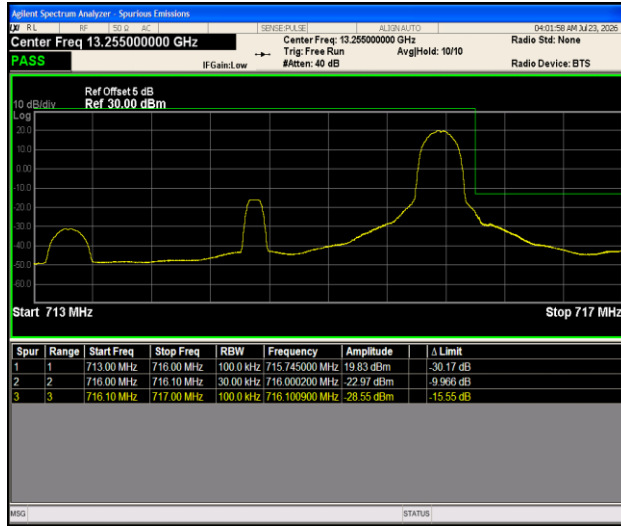
Band12-3MHz- 16QAM-23165-1RB#14-PASS
