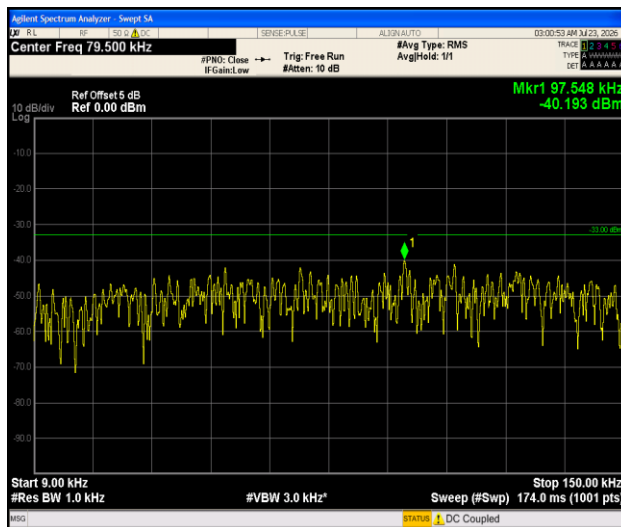
Band12-1.4MHz- 16QAM-23095-1RB#0-0.009~0.15-PASS
