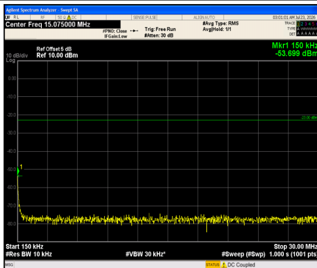
Band12-1.4MHz- 16QAM-23095-1RB#0-0.15~30-PASS
