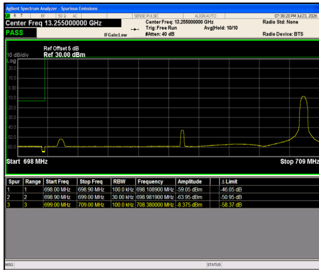
Band12-10MHz-16QAM-23060-1RB#49-PASS
