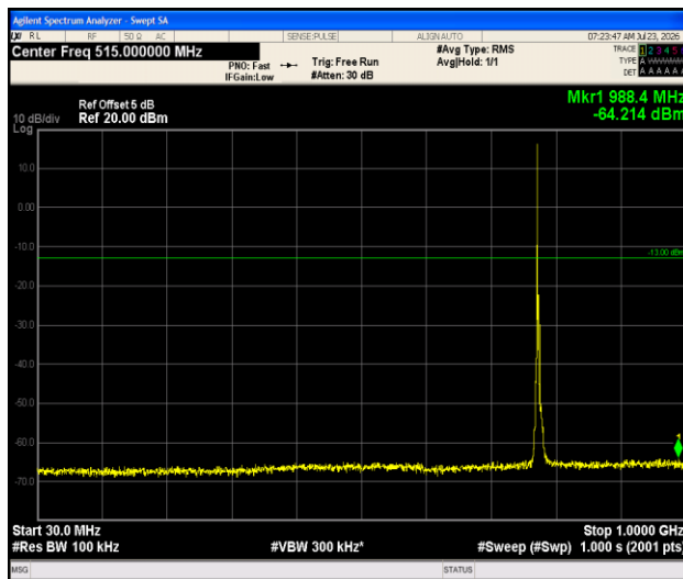
Band13-5MHz- 16QAM-23205-1RB#0-30~1000-PASS
