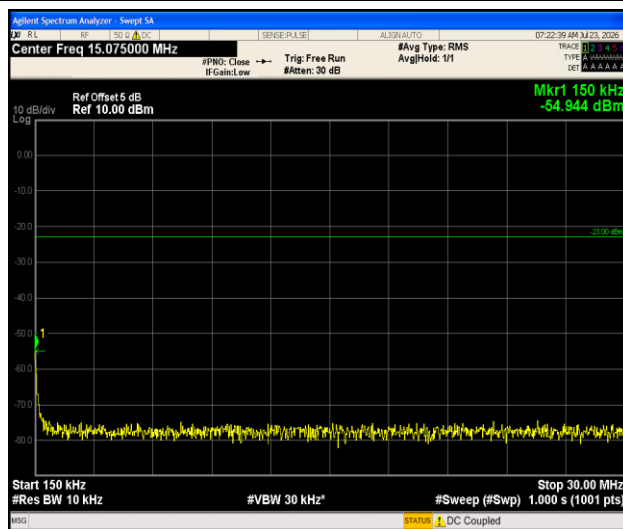
Band13-5MHz-QPSK-23205-1RB#0-0.15~30-PASS
