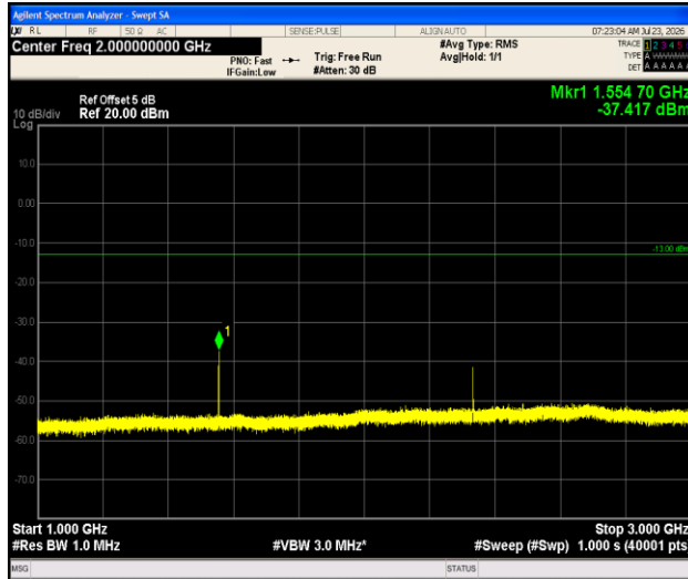
Band13-5MHz-QPSK-23205-1RB#0-1000~3000-PASS
