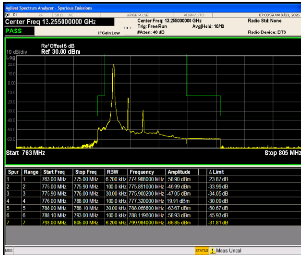
Band13-5MHz- 16QAM-23205-1RB#0-PASS
