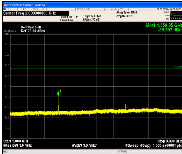
Band13-5MHz-QPSK-23230-1RB#0-1000~3000-PASS
