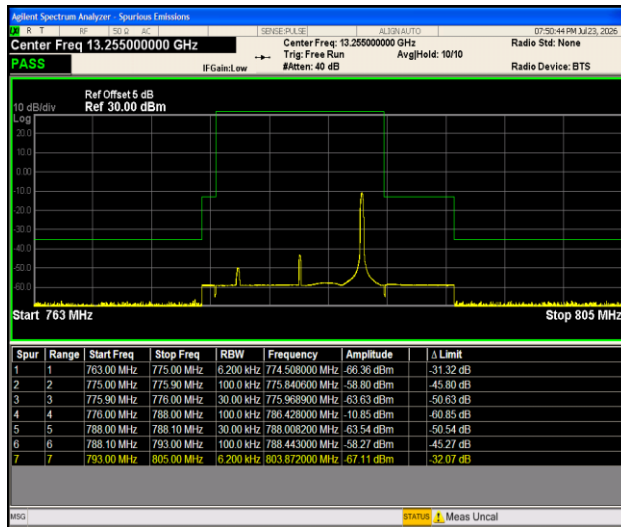
Band13-10MHz-16QAM-23230-1RB#49-PASS
