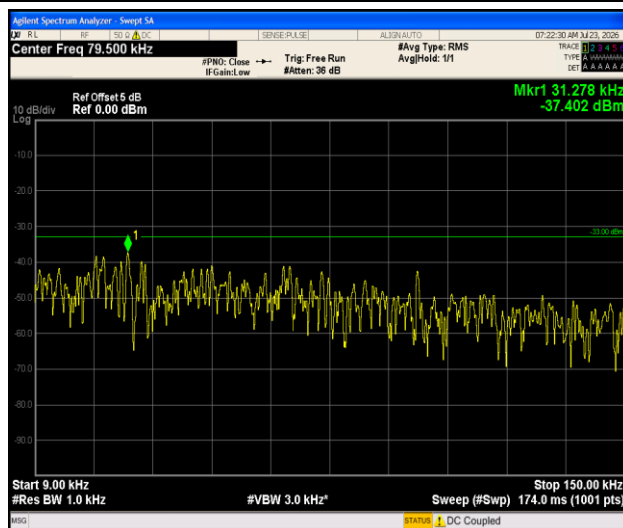
Band13-5MHz-QPSK-23205-1RB#0-0.009~0.15-PASS
