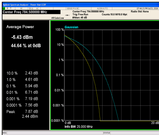
Band13-5MHz- 16QAM-23255-25RB#0-PASS
