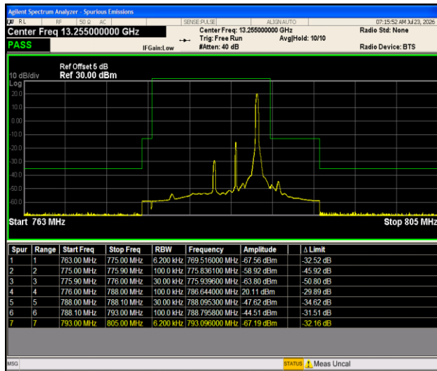
Band13-5MHz-QPSK-23255-1RB#24-PASS
