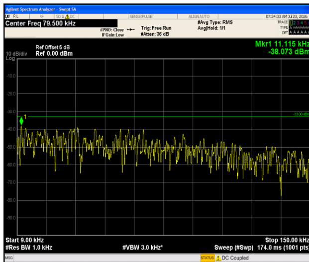
Band13-5MHz-QPSK-23230-1RB#0-0.009~0.15-PASS
