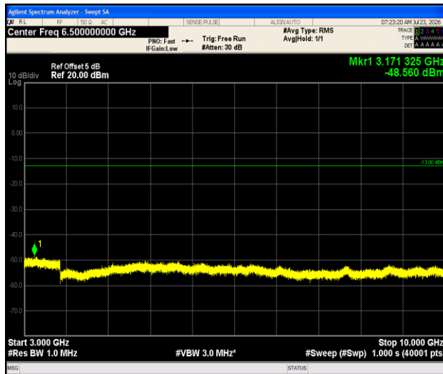
Band13-5MHz-QPSK-23205-1RB#0-3000~10000-PASS
