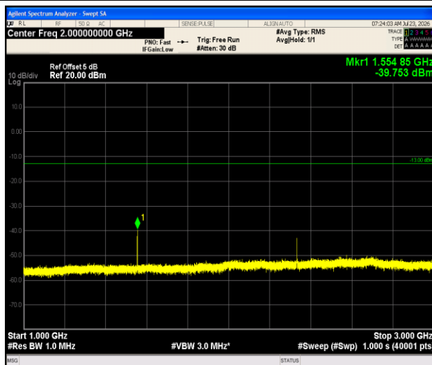
Band13-5MHz- 16QAM-23205-1RB#0-1000~3000-PASS
