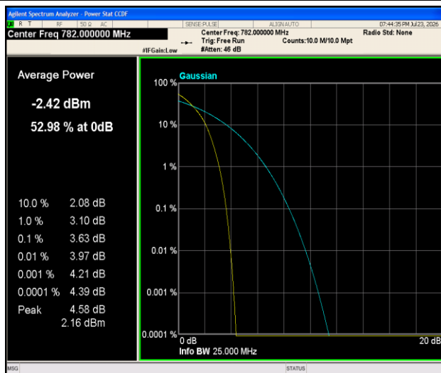
Band13-5MHz- 16QAM-23230-1RB#0-PASS
