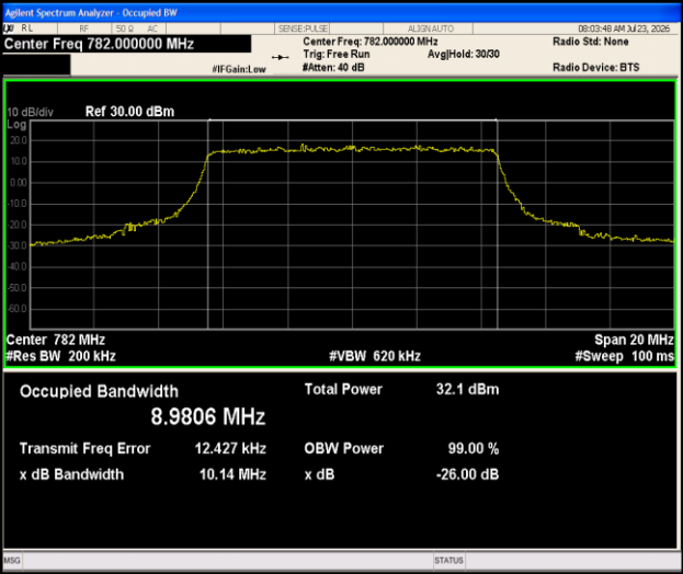
Band13-10MHz-QPSK-23230-50RB#0-PASS
