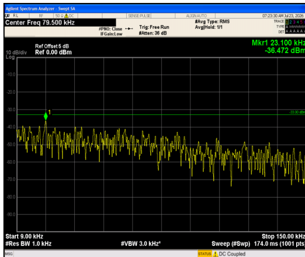
Band13-5MHz- 16QAM-23205-1RB#0-0.009~0.15-PASS
