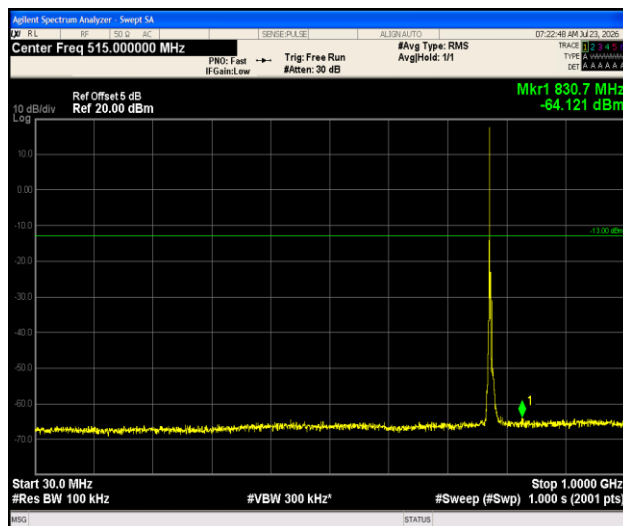
Band13-5MHz-QPSK-23205-1RB#0-30~1000-PASS
