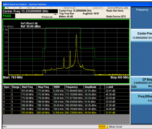
Band13-5MHz-16QAM-23255-1RB#24-PASS
