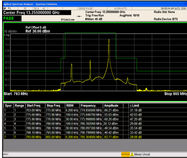
Band13-10MHz-QPSK-23230-1RB#49-PASS
