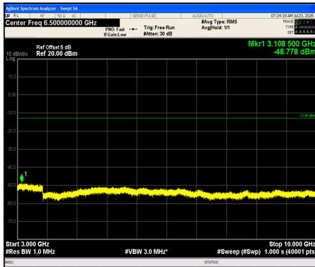
Band13-5MHz- 16QAM-23205-1RB#0-3000~10000-PASS
