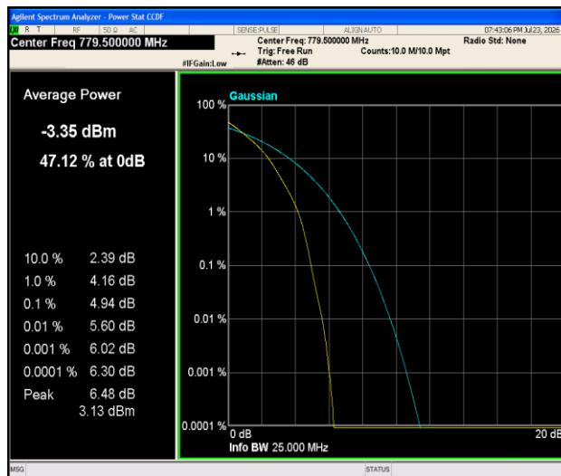
Band13-5MHz-QPSK-23205-1RB#0-PASS
