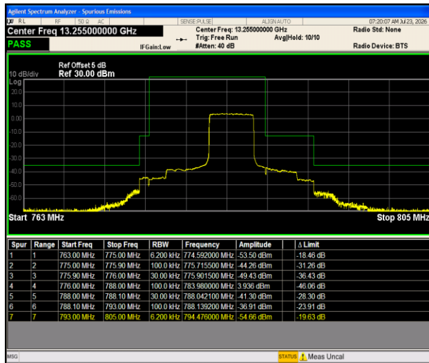
Band13-5MHz-QPSK-23255-25RB#0-PASS
