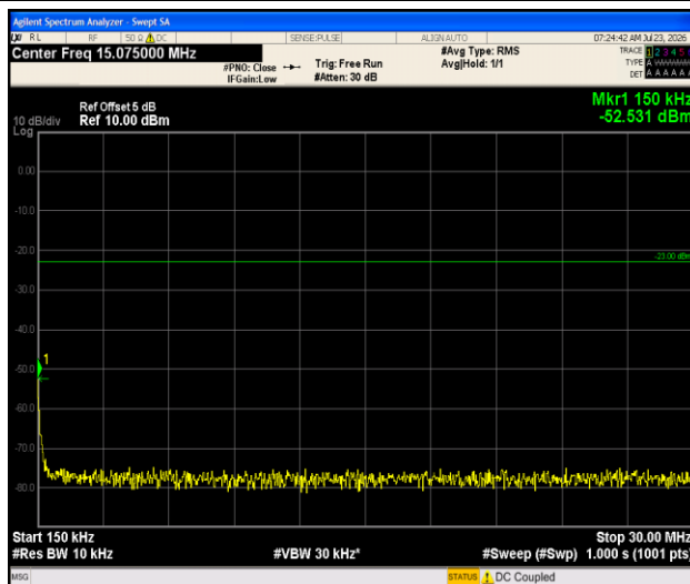
Band13-5MHz-QPSK-23230-1RB#0-0.15~30-PASS
