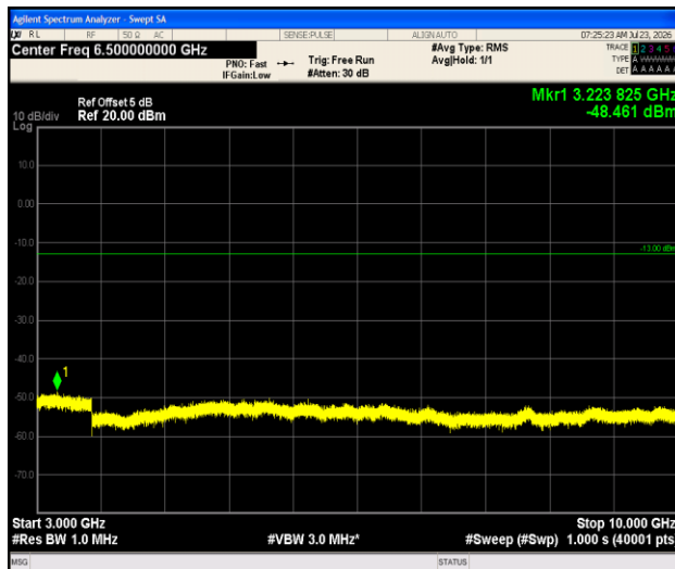
Band13-5MHz-QPSK-23230-1RB#0-3000~10000-PASS
