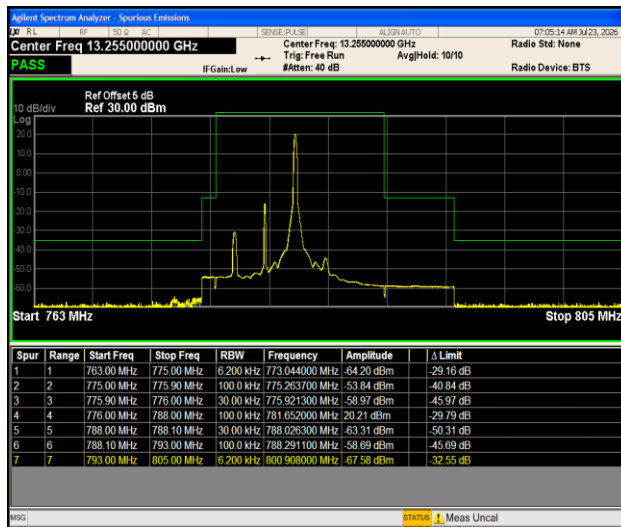
Band13-5MHz- 16QAM-23205-1RB#24-PASS
