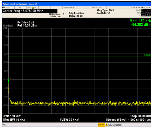
Band13-5MHz- 16QAM-23205-1RB#0-0.15~30-PASS
