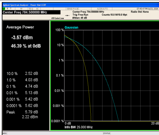
Band13-5MHz- 16QAM-23255-1RB#0-PASS
