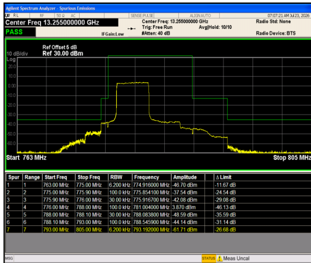
Band13-5MHz-QPSK-23205-25RB#0-PASS
