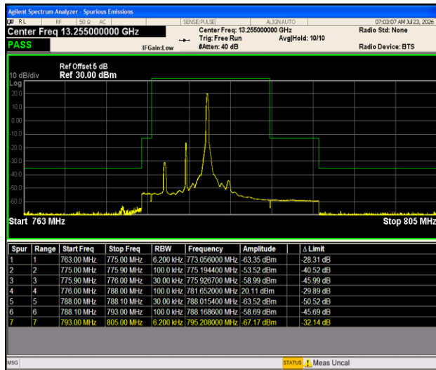
Band13-5MHz-QPSK-23205-1RB#24-PASS
