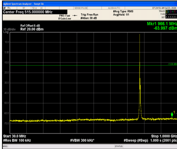
Band13-5MHz-QPSK-23230-1RB#0-30~1000-PASS
