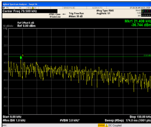
Band13-5MHz-QPSK-23255-1RB#0-0.009~0.15-PASS
