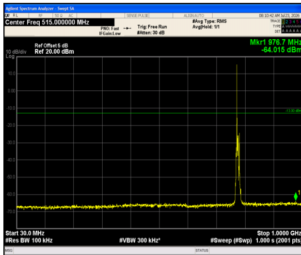
Band13-10MHz-QPSK-23230-1RB#0-30~1000-PASS
