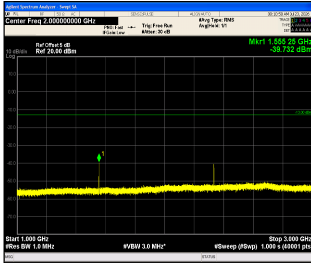
Band13-10MHz-QPSK-23230-1RB#0-1000~3000-PASS
