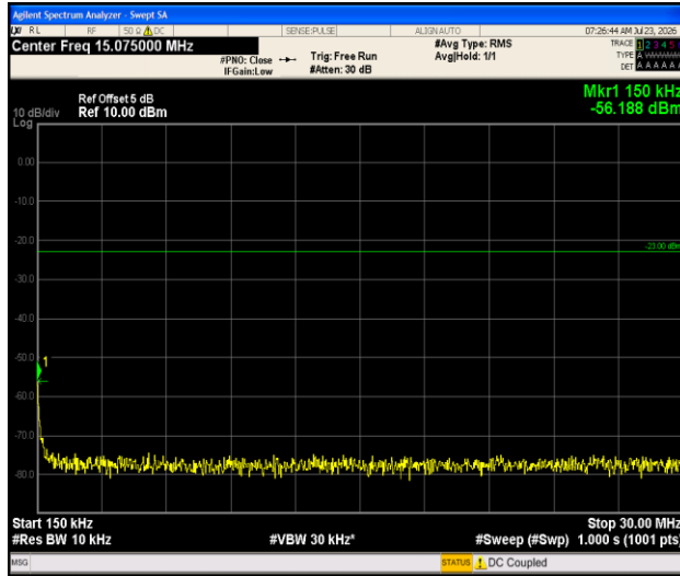
Band13-5MHz-QPSK-23255-1RB#0-0.15~30-PASS
