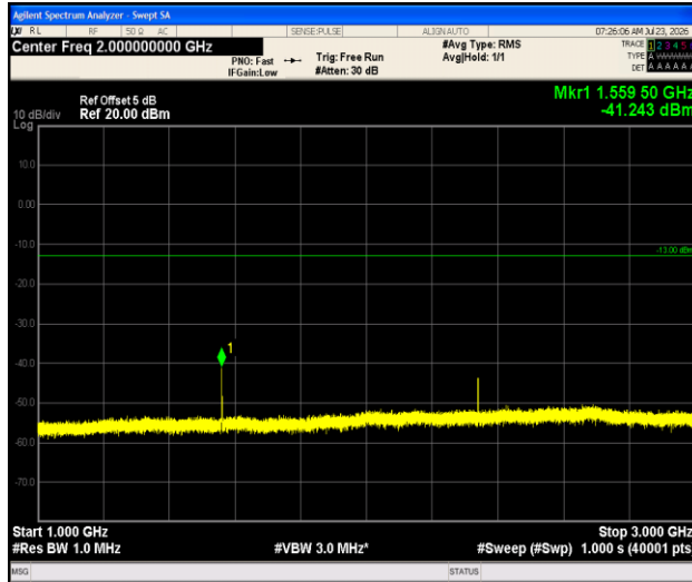
Band13-5MHz- 16QAM-23230-1RB#0-1000~3000-PASS
