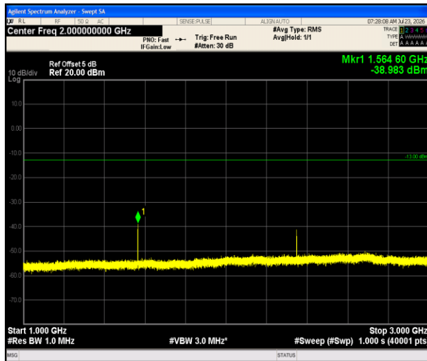
Band13-5MHz- 16QAM-23255-1RB#0-1000~3000-PASS
