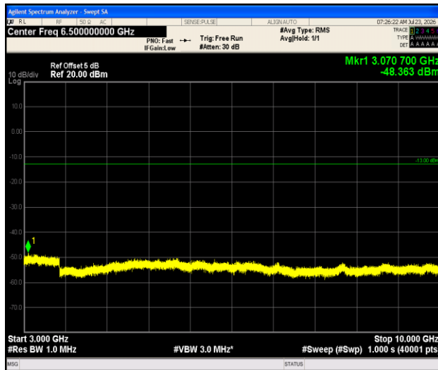
Band13-5MHz- 16QAM-23230-1RB#0-3000~10000-PASS
