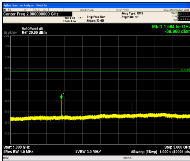
Band13-5MHz-QPSK-23255-1RB#0-1000~3000-PASS
