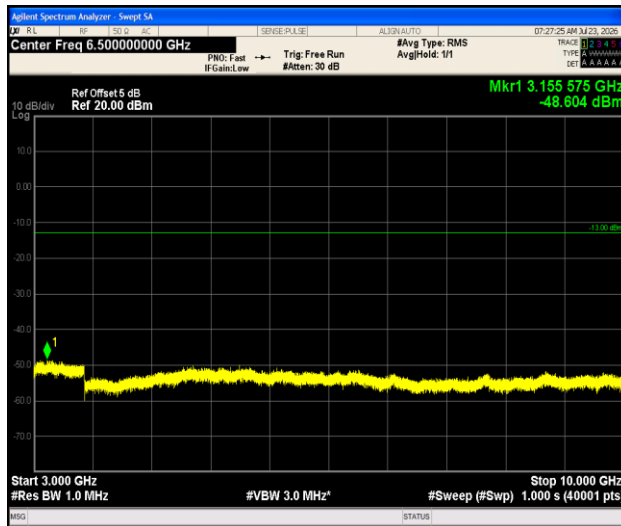
Band13-5MHz-QPSK-23255-1RB#0-3000~10000-PASS
