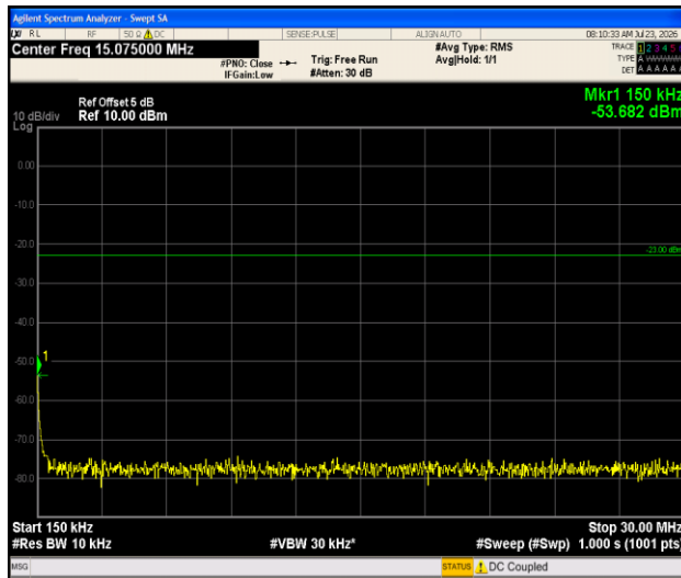
Band13-10MHz-QPSK-23230-1RB#0-0.15~30-PASS
