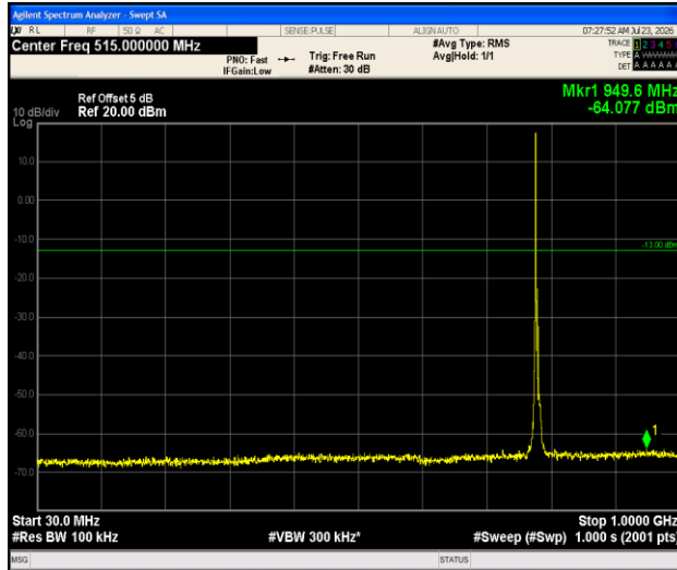
Band13-5MHz- 16QAM-23255-1RB#0-30~1000-PASS
