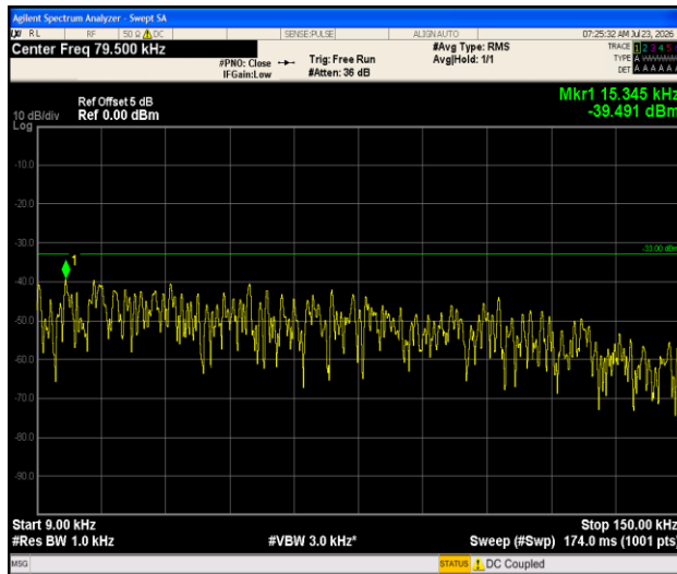
Band13-5MHz- 16QAM-23230-1RB#0-0.009~0.15-PASS
