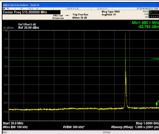
Band13-5MHz- 16QAM-23230-1RB#0-30~1000-PASS
