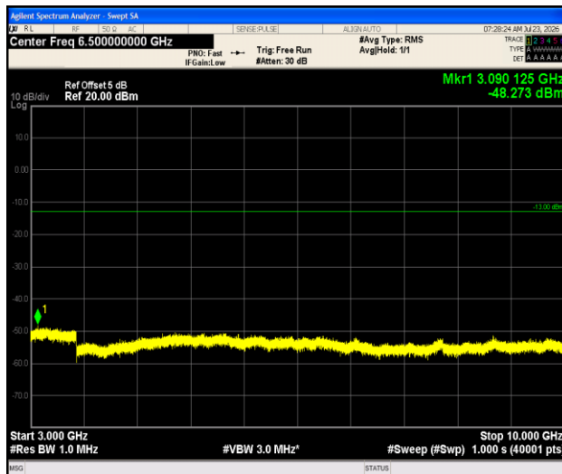
Band13-5MHz- 16QAM-23255-1RB#0-3000~10000-PASS
