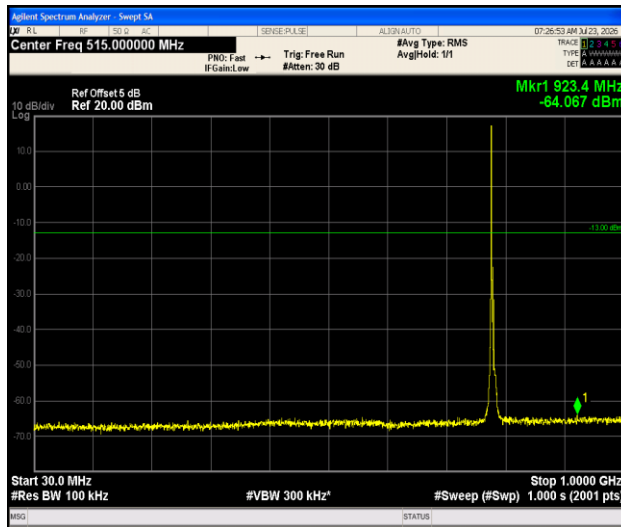
Band13-5MHz-QPSK-23255-1RB#0-30~1000-PASS
