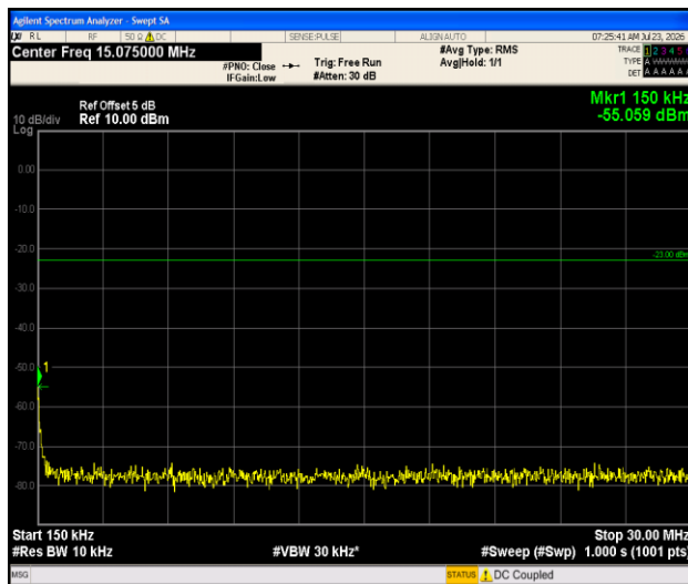
Band13-5MHz- 16QAM-23230-1RB#0-0.15~30-PASS
