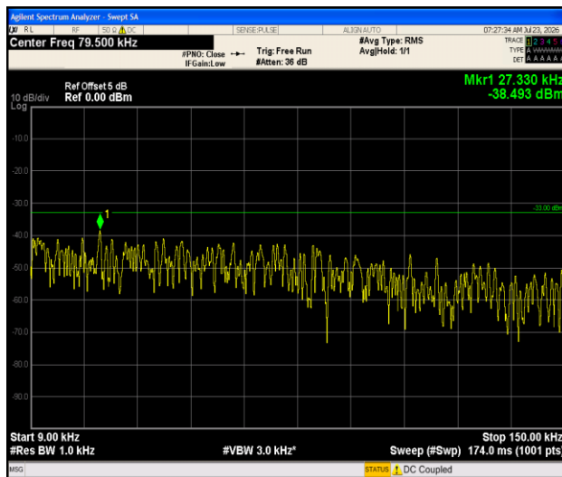
Band13-5MHz- 16QAM-23255-1RB#0-0.009~0.15-PASS
