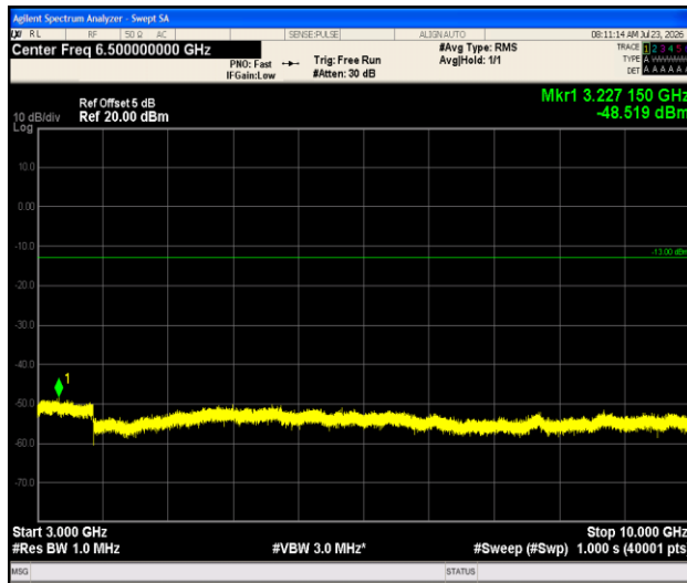
Band13-10MHz-QPSK-23230-1RB#0-3000~10000-PASS
