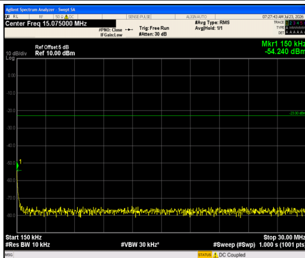
Band13-5MHz- 16QAM-23255-1RB#0-0.15~30-PASS
