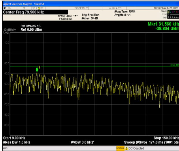
Band13-10MHz-QPSK-23230-1RB#0-0.009~0.15-PASS
