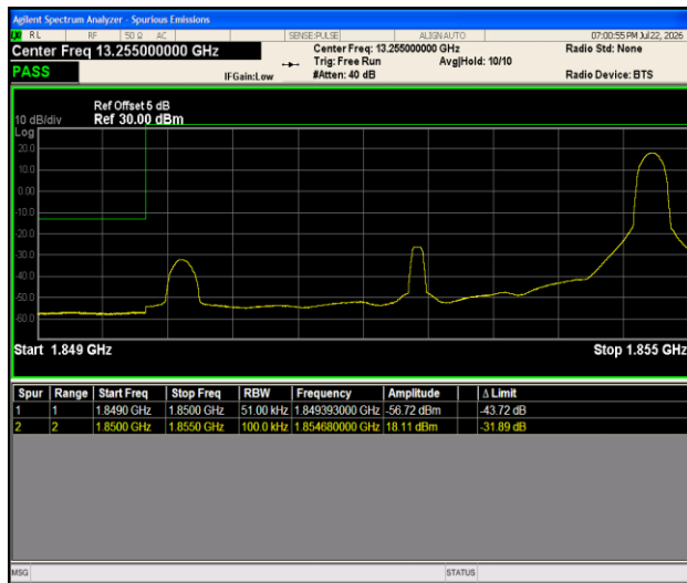
Band2-5MHz-16QAM-18625-1RB#24-PASS
