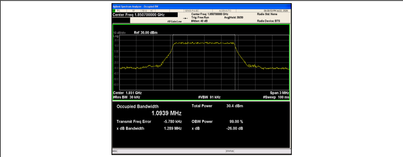
Band2-1.4MHz-QPSK-18607-6RB#0-PASS
