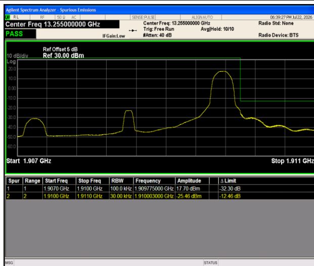
Band2-3MHz-16QAM-19185-1RB#14-PASS
