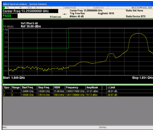
Band2-1.4MHz-QPSK-18607-1RB#5-PASS
