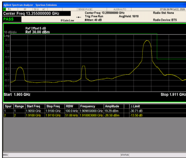
Band2-5MHz-QPSK-19175-1RB#24-PASS
