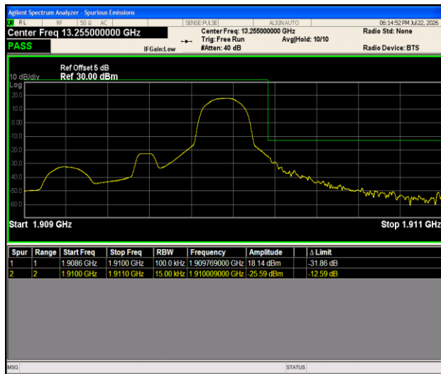
Band2-1.4MHz-16QAM-19193-1RB#5-PASS
