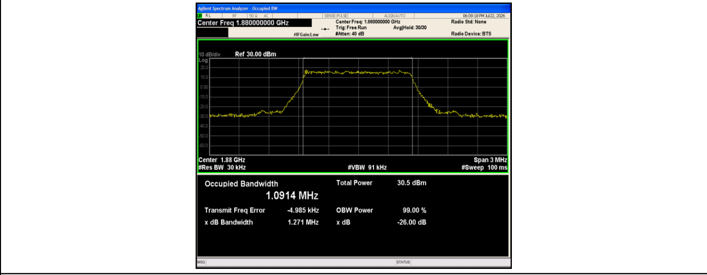
Band2-1.4MHz-QPSK-18900-6RB#0-PASS
