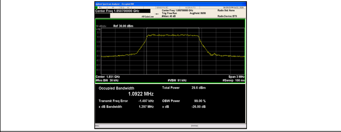
Band2-1.4MHz-16QAM-18607-6RB#0-PASS
