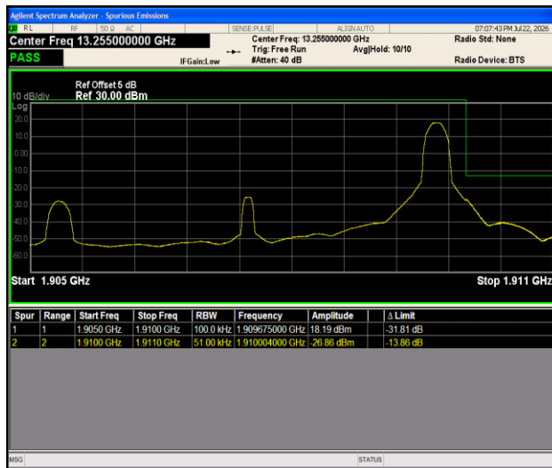
Band2-5MHz-16QAM-19175-1RB#24-PASS
