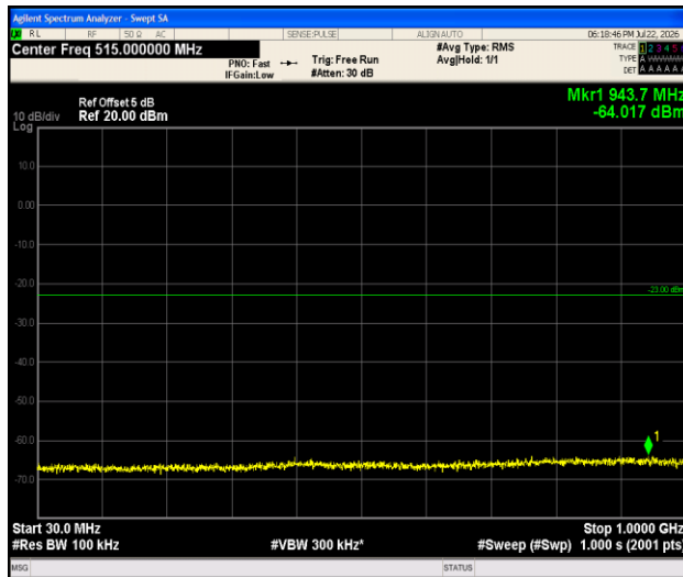
Band2-1.4MHz-QPSK-18900-1RB#0-30~1000-PASS
