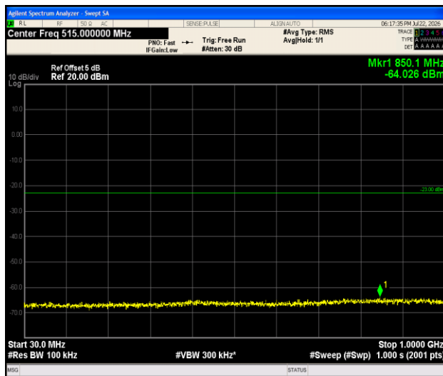
Band2-1.4MHz-16QAM-18607-1RB#0-30~1000-PASS
