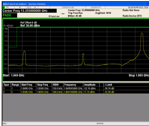
Band2-15MHz-16QAM-18675-1RB#74-PASS
