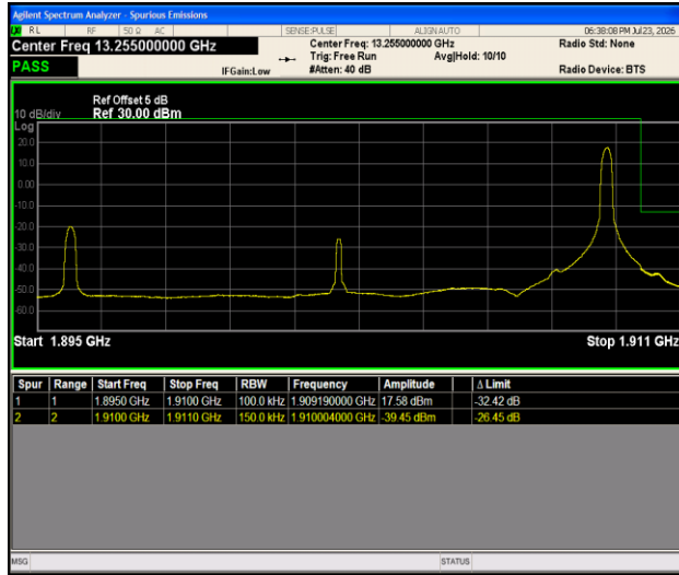
Band2-15MHz-16QAM-19125-1RB#74-PASS
