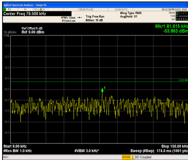
Band2-1.4MHz-QPSK-19193-1RB#0-0.009~0.15-PASS
