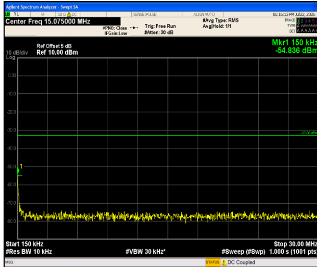
Band2-1.4MHz-QPSK-18607-1RB#0-0.15~30-PASS
