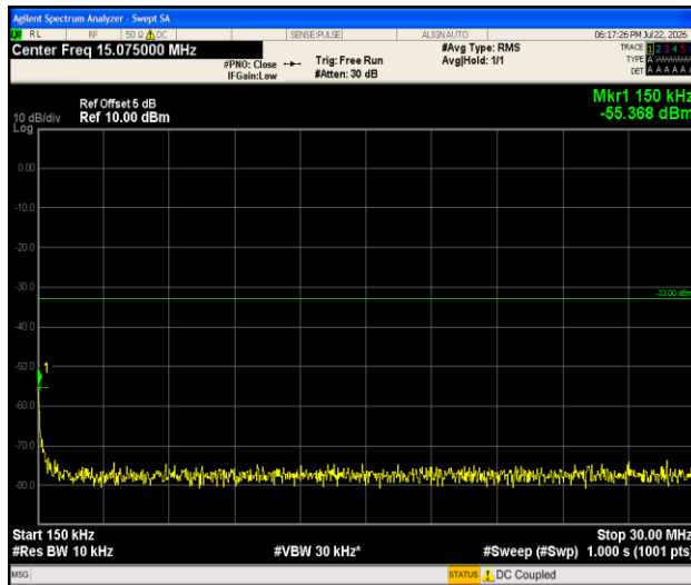
Band2-1.4MHz-16QAM-18607-1RB#0-0.15~30-PASS
