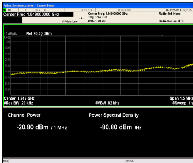
Band2-3MHz-QPSK-18615-1RB#0-1000~3000- PASS-Final
