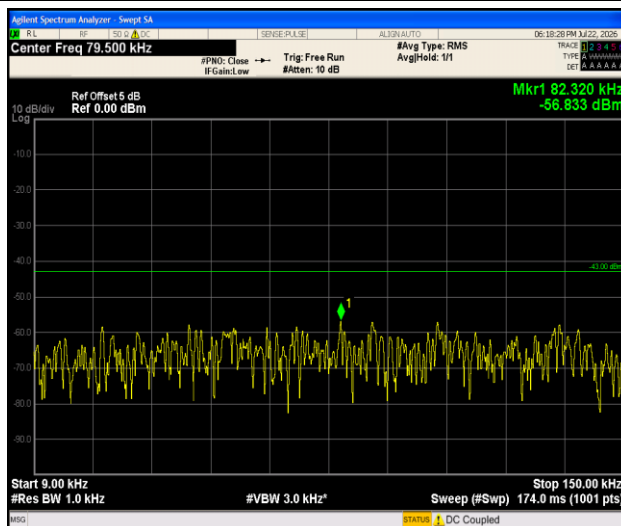
Band2-1.4MHz-QPSK-18900-1RB#0-0.009~0.15-PASS
