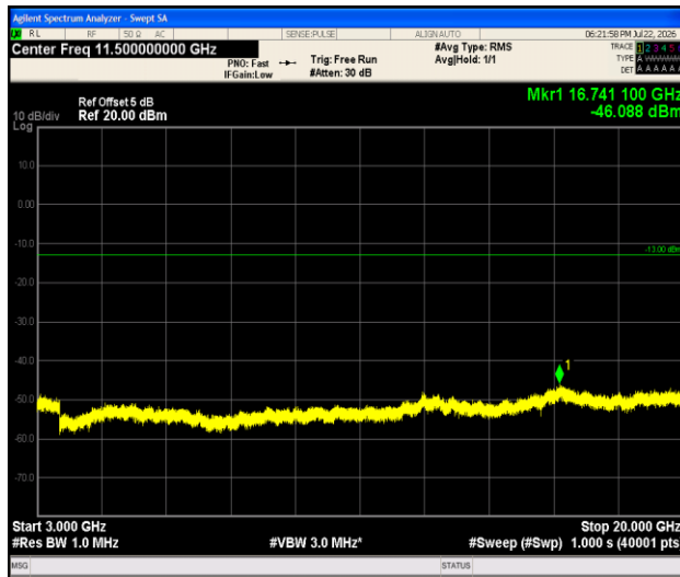
Band2-1.4MHz-QPSK-19193-1RB#0-3000~20000-PASS
