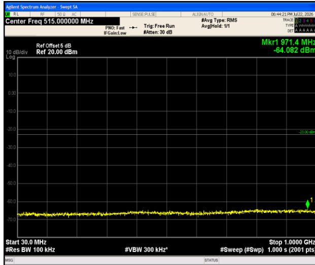
Band2-3MHz-QPSK-18615-1RB#0-30~1000-PASS
