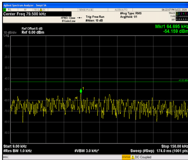
Band2-1.4MHz-16QAM-19193-1RB#0-0.009~0.15-PASS
