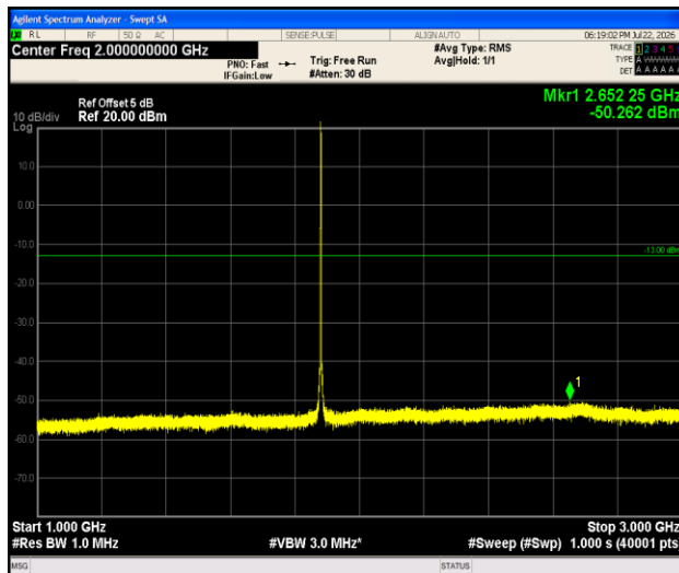
Band2-1.4MHz-QPSK-18900-1RB#0-1000~3000-PASS
