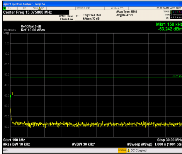
Band2-1.4MHz-16QAM-19193-1RB#0-0.15~30-PASS
