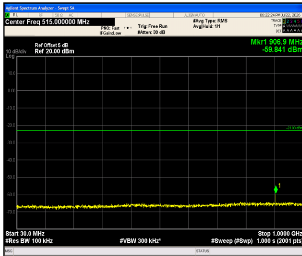
Band2-1.4MHz-16QAM-19193-1RB#0-30~1000-PASS
