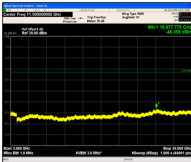
Band2-1.4MHz-16QAM-18607-1RB#0-3000~20000-PASS
