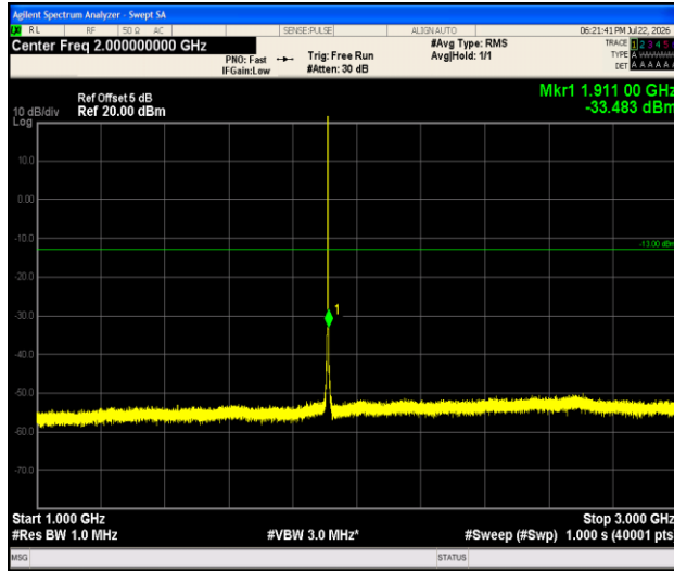
Band2-1.4MHz-QPSK-19193-1RB#0-1000~3000-PASS
