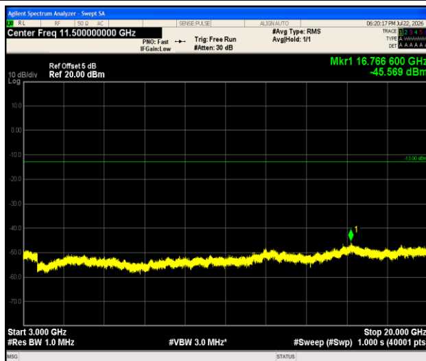
Band2-1.4MHz-16QAM-18900-1RB#0-3000~20000-PASS
