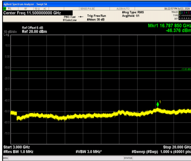
Band2-1.4MHz-16QAM-19193-1RB#0-3000~20000-PASS
