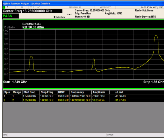
Band2-10MHz-16QAM-18650-1RB#49-PASS
