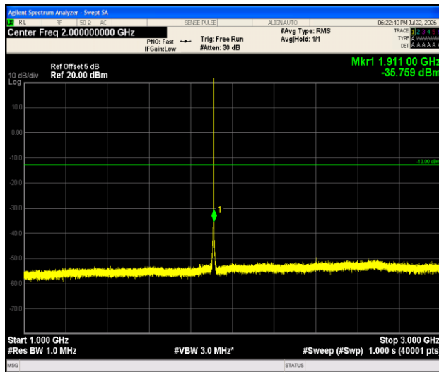
Band2-1.4MHz-16QAM-19193-1RB#0-1000~3000-PASS
