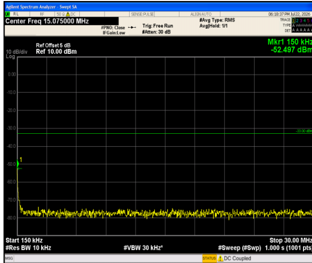
Band2-1.4MHz-QPSK-18900-1RB#0-0.15~30-PASS
