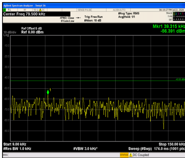
Band2-1.4MHz-16QAM-18900-1RB#0-0.009~0.15-PASS
