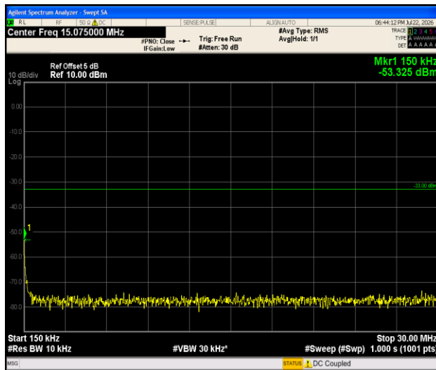
Band2-3MHz-QPSK-18615-1RB#0-0.15~30-PASS
