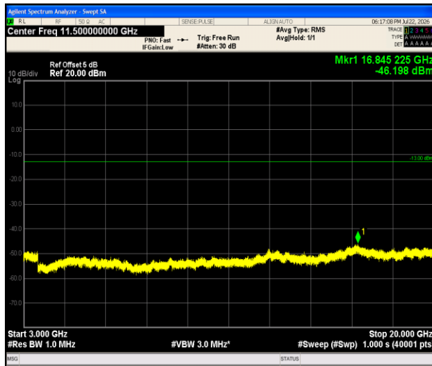
Band2-1.4MHz-QPSK-18607-1RB#0-3000~20000-PASS
