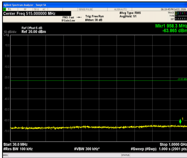
Band2-1.4MHz-16QAM-18900-1RB#0-30~1000-PASS
