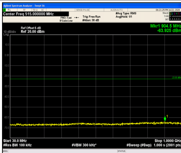
Band2-1.4MHz-QPSK-19193-1RB#0-30~1000-PASS
