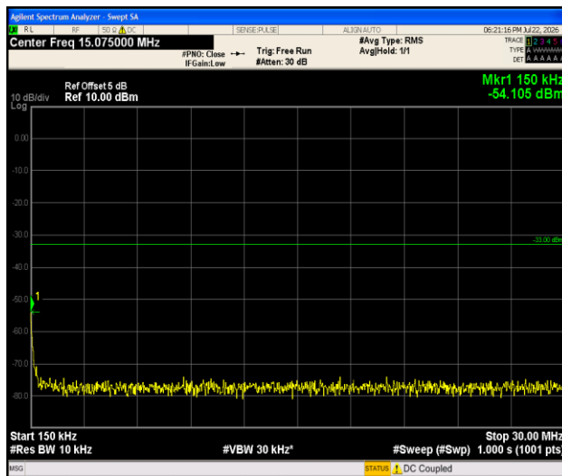
Band2-1.4MHz-QPSK-19193-1RB#0-0.15~30-PASS
