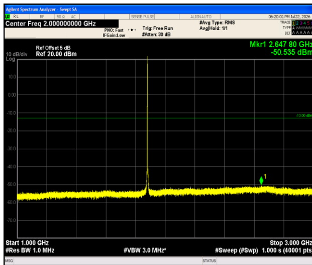
Band2-1.4MHz-16QAM-18900-1RB#0-1000~3000-PASS
