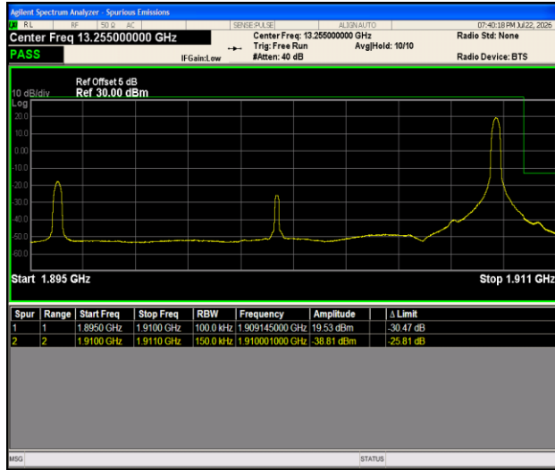
Band2-15MHz-QPSK-19125-1RB#74-PASS
