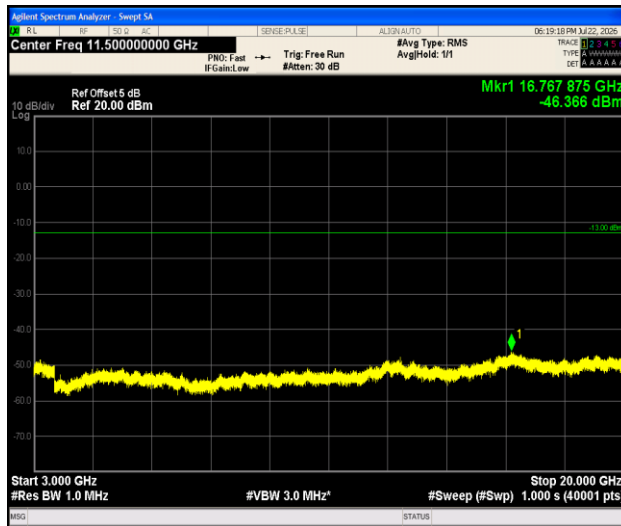
Band2-1.4MHz-QPSK-18900-1RB#0-3000~20000-PASS
