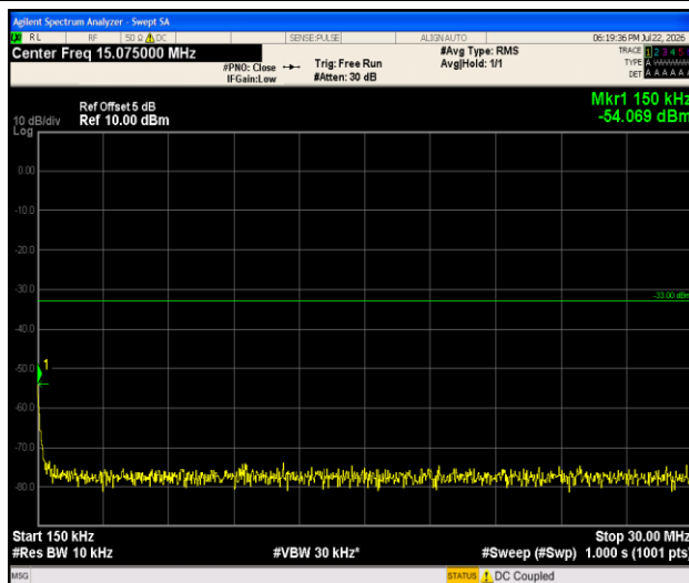
Band2-1.4MHz-16QAM-18900-1RB#0-0.15~30-PASS
