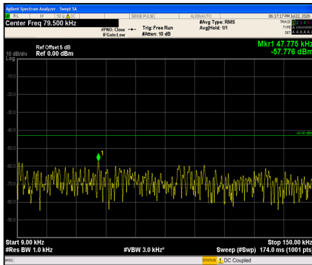
Band2-1.4MHz-16QAM-18607-1RB#0-0.009~0.15-PASS
