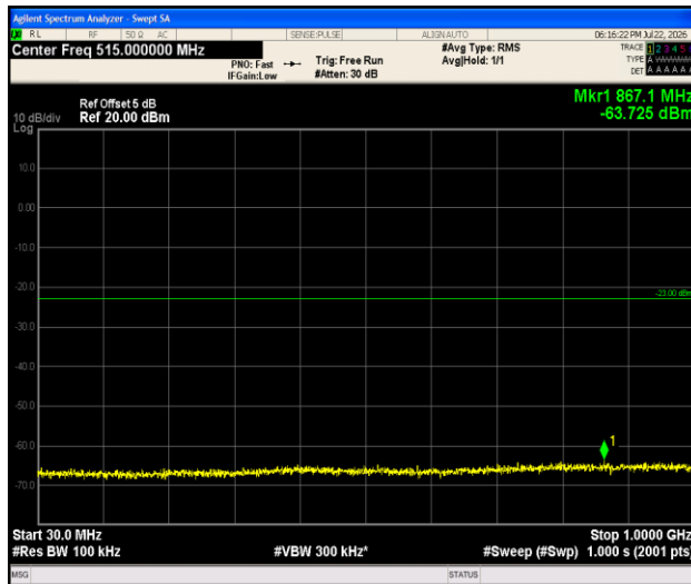
Band2-1.4MHz-QPSK-18607-1RB#0-30~1000-PASS
