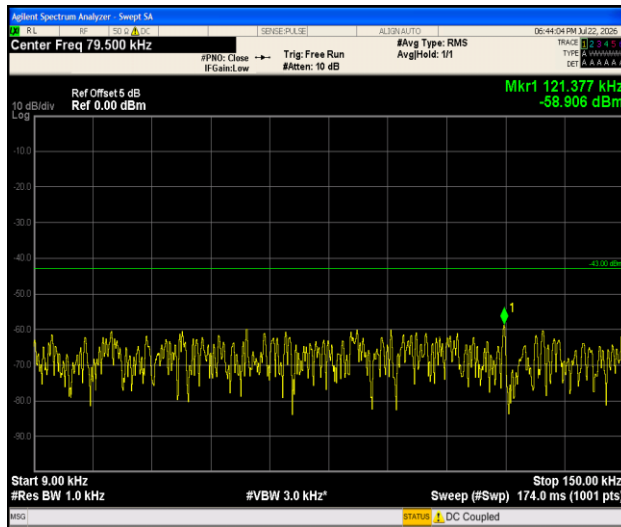
Band2-3MHz-QPSK-18615-1RB#0-0.009~0.15-PASS
