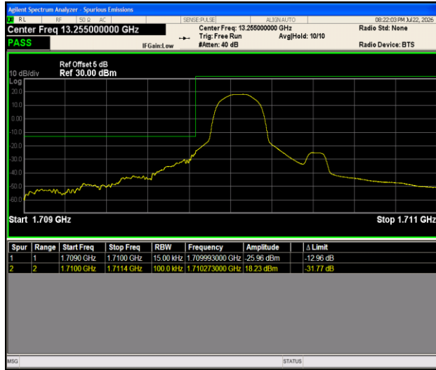
Band4-1.4MHz-16QAM-19957-1RB#0-PASS
