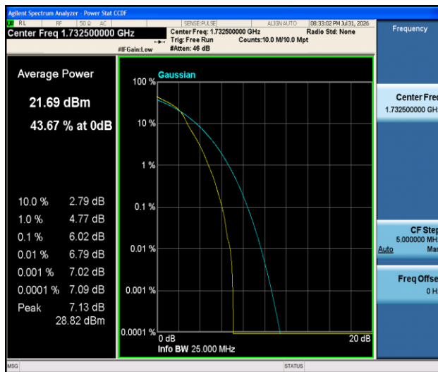
Band4-20MHz-16QAM-20175-1RB#0-PASS
