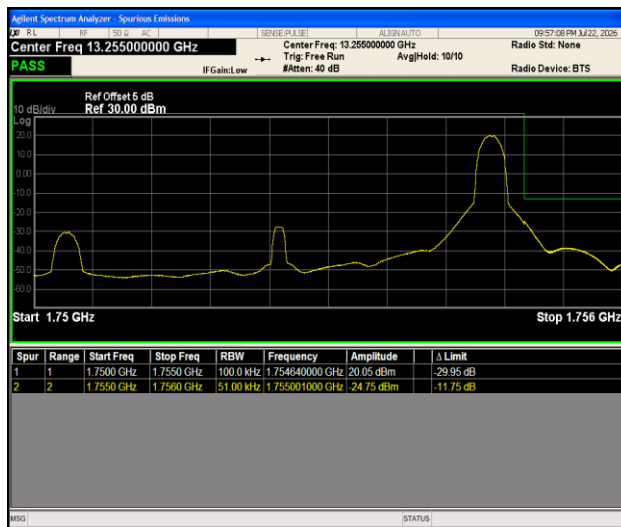
Band4-5MHz-QPSK-20375-1RB#24-PASS
