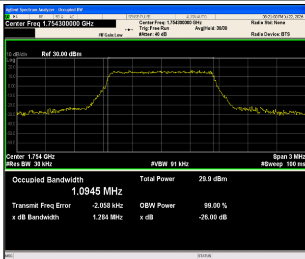
Band4-1.4MHz-16QAM-20393-6RB#0-PASS
