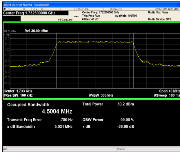
Band4-5MHz-16QAM-20175-25RB#0-PASS
