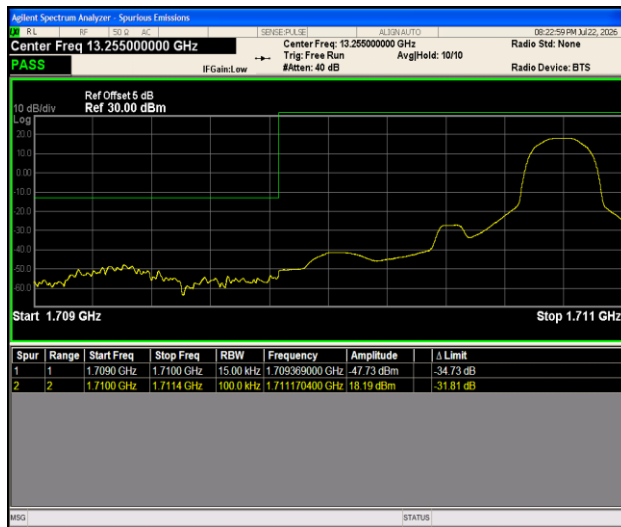
Band4-1.4MHz-16QAM-19957-1RB#5-PASS
