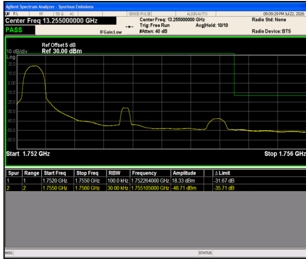
Band4-3MHz-16QAM-20385-1RB#0-PASS
