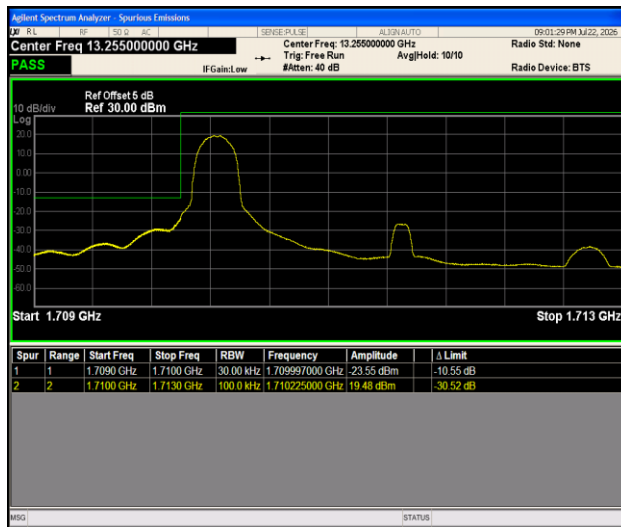
Band4-3MHz-QPSK-19965-1RB#0-PASS
