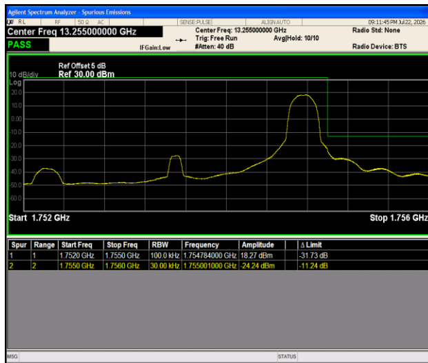
Band4-3MHz-16QAM-20385-1RB#14-PASS
