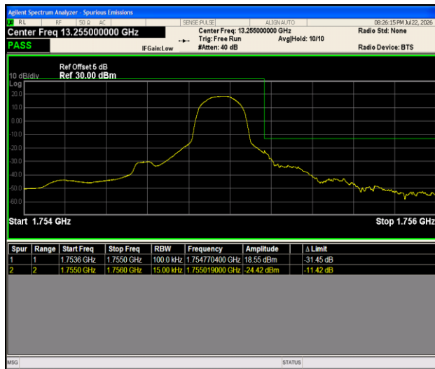
Band4-1.4MHz-16QAM-20393-1RB#5-PASS
