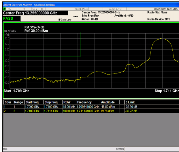
Band4-1.4MHz-QPSK-19957-1RB#5-PASS
