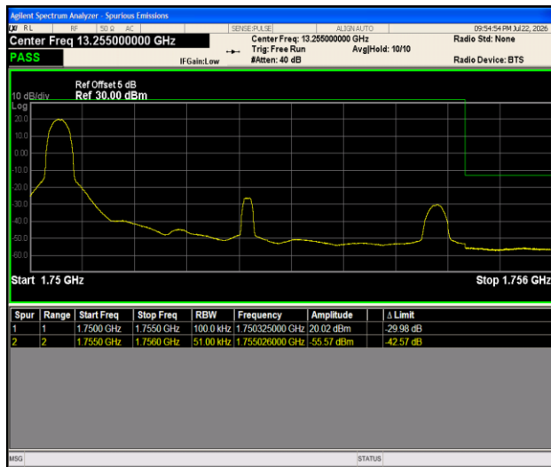
Band4-5MHz-QPSK-20375-1RB#0-PASS
