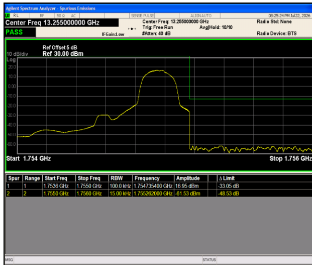
Band4-1.4MHz-QPSK-20393-1RB#5-PASS
