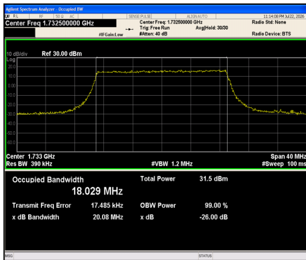
Band4-20MHz-QPSK-20175-100RB#0-PASS
