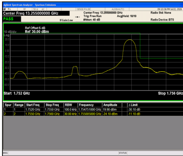
Band4-3MHz-QPSK-20385-1RB#14-PASS
