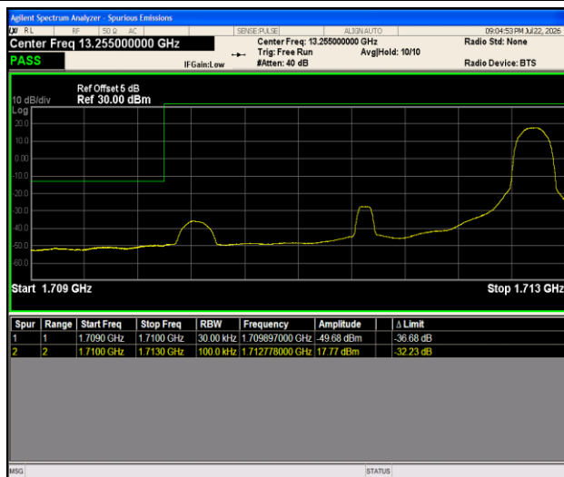
Band4-3MHz-16QAM-19965-1RB#14-PASS
