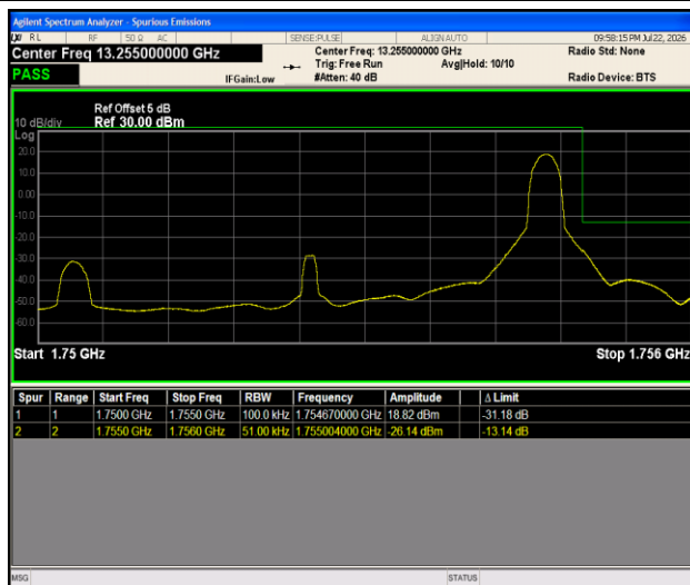
Band4-5MHz-16QAM-20375-1RB#24-PASS
