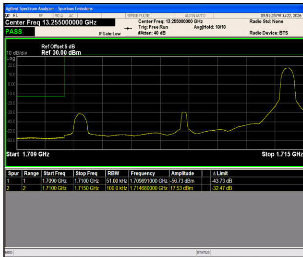
Band4-5MHz-16QAM-19975-1RB#24-PASS
