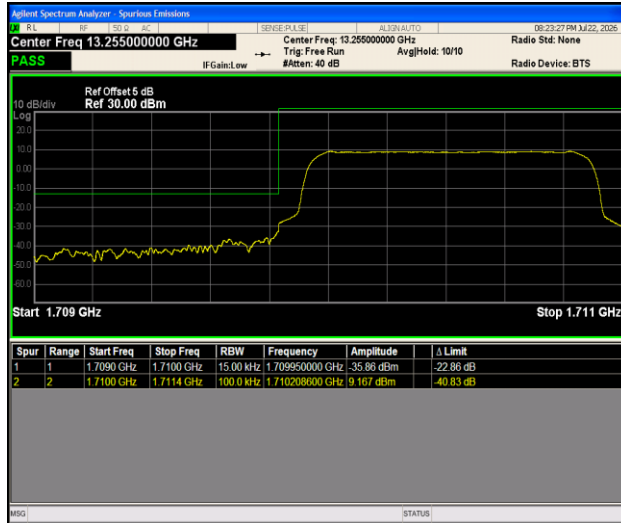
Band4-1.4MHz-QPSK-19957-6RB#0-PASS
