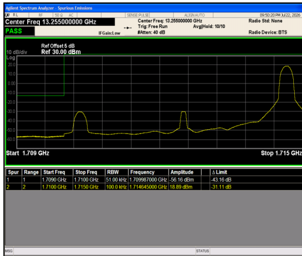
Band4-5MHz-QPSK-19975-1RB#24-PASS
