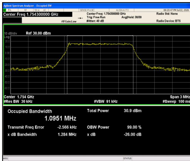
Band4-1.4MHz-QPSK-20393-6RB#0-PASS
