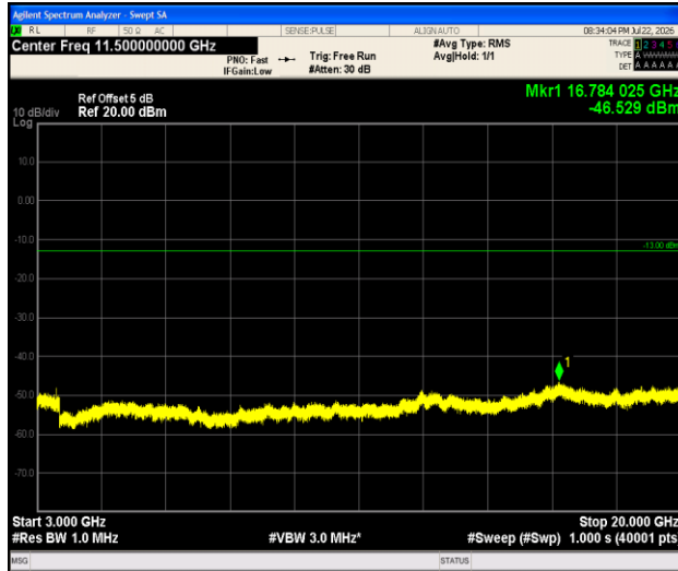
Band4-1.4MHz-16QAM-20393-1RB#0-3000~20000-PASS
