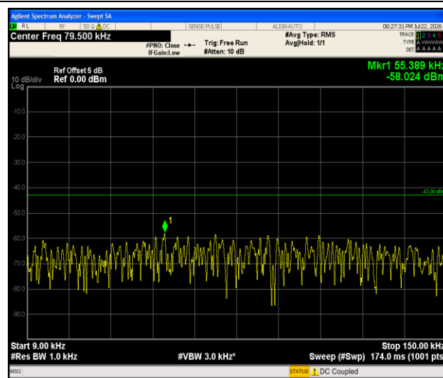
Band4-1.4MHz-QPSK-19957-1RB#0-0.009~0.15-PASS
