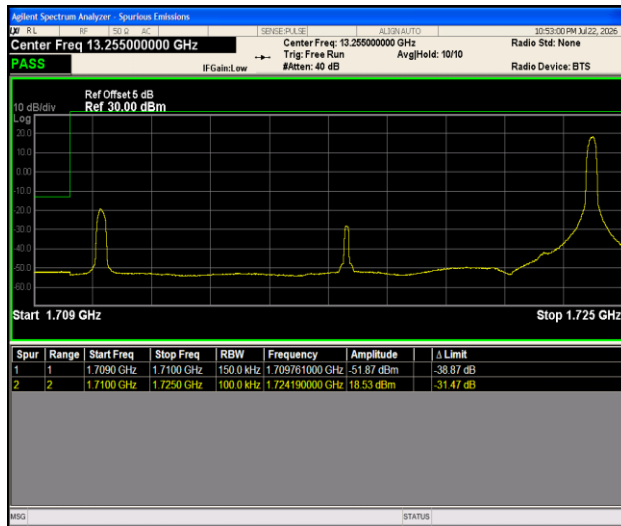
Band4-15MHz-QPSK-20025-1RB#74-PASS
