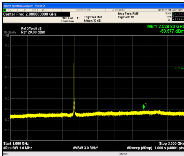
Band4-1.4MHz-QPSK-20175-1RB#0-1000~3000-PASS
