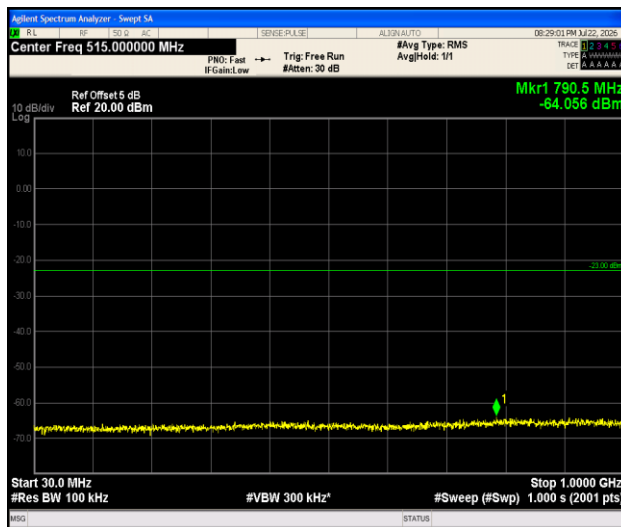
Band4-1.4MHz-16QAM-19957-1RB#0-30~1000-PASS
