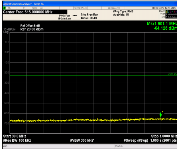
Band4-1.4MHz-16QAM-20175-1RB#0-30~1000-PASS
