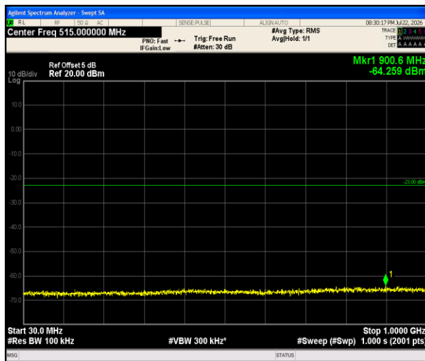
Band4-1.4MHz-QPSK-20175-1RB#0-30~1000-PASS
