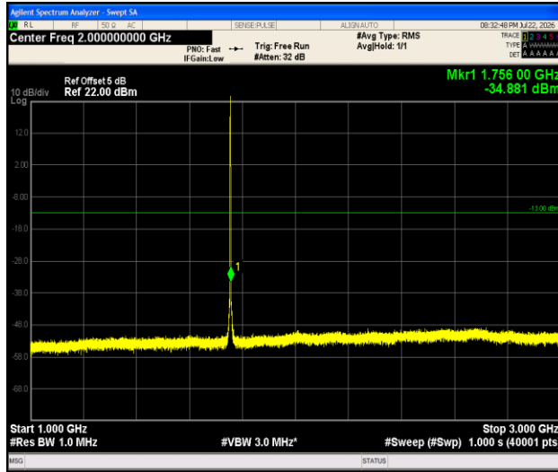
Band4-1.4MHz-QPSK-20393-1RB#0-1000~3000-PASS
