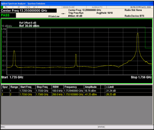
Band4-20MHz-16QAM-20300-1RB#99-PASS
