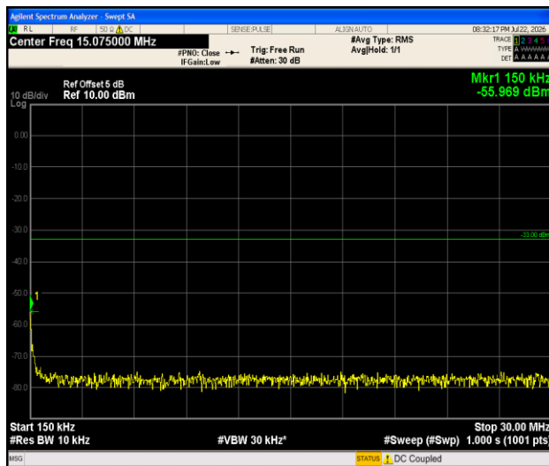
Band4-1.4MHz-QPSK-20393-1RB#0-0.15~30-PASS
