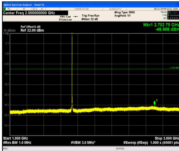
Band4-1.4MHz-16QAM-20175-1RB#0-1000~3000-PASS
