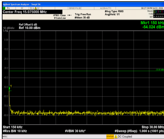
Band4-1.4MHz-QPSK-19957-1RB#0-0.15~30-PASS
