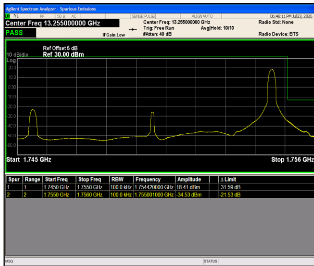
Band4-10MHz-16QAM-20350-1RB#49-PASS
