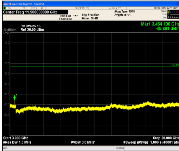
Band4-1.4MHz-QPSK-20175-1RB#0-3000~20000-PASS
