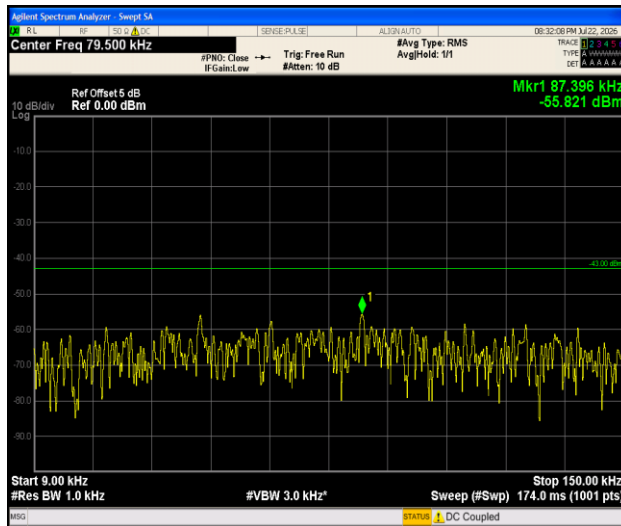
Band4-1.4MHz-QPSK-20393-1RB#0-0.009~0.15-PASS
