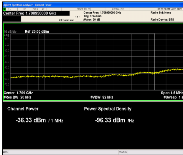
Band4-1.4MHz-16QAM-19957-1RB#0-1000~3000- PASS-Final
