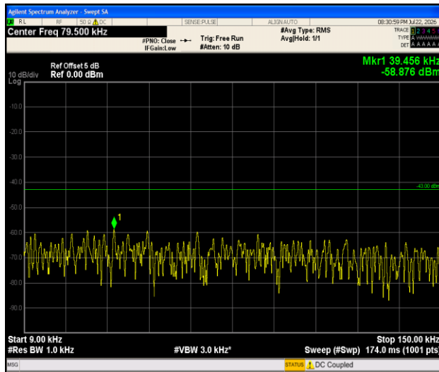
Band4-1.4MHz-16QAM-20175-1RB#0-0.009~0.15-PASS
