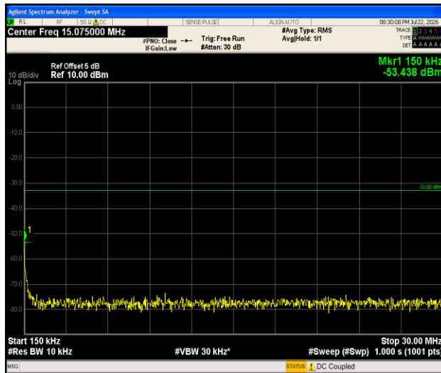
Band4-1.4MHz-QPSK-20175-1RB#0-0.15~30-PASS
