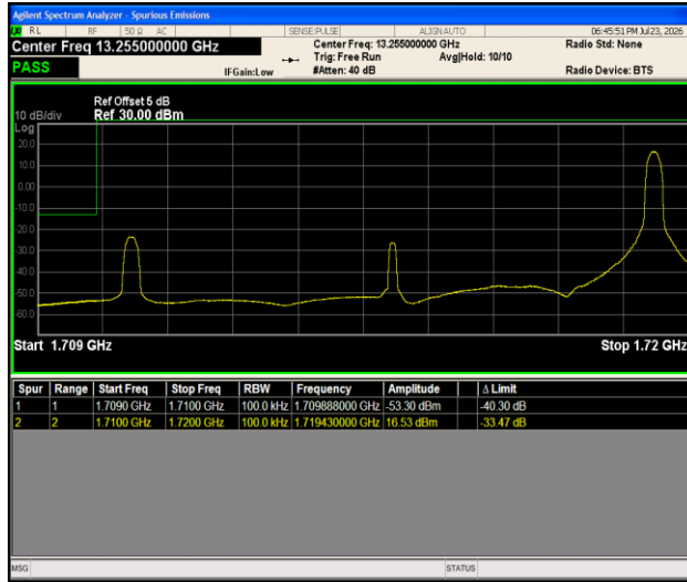
Band4-10MHz-16QAM-20000-1RB#49-PASS
