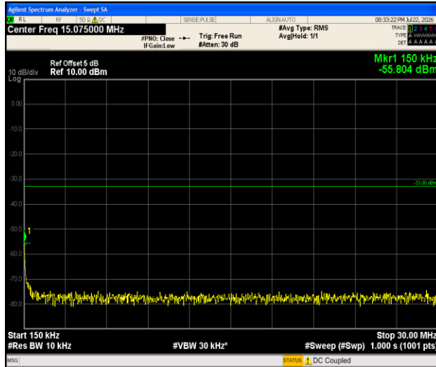
Band4-1.4MHz-16QAM-20393-1RB#0-0.15~30-PASS
