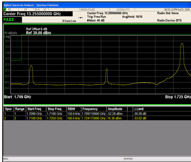
Band4-15MHz-16QAM-20025-1RB#74-PASS
