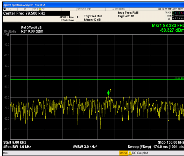
Band4-3MHz-QPSK-19965-1RB#0-0.009~0.15-PASS
