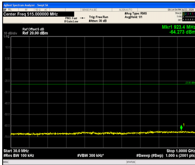
Band4-3MHz-QPSK-19965-1RB#0-30~1000-PASS
