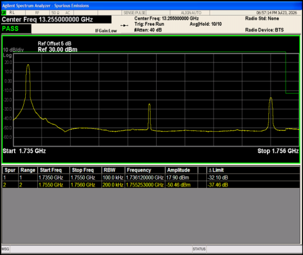
Band4-20MHz-16QAM-20300-1RB#0-PASS
