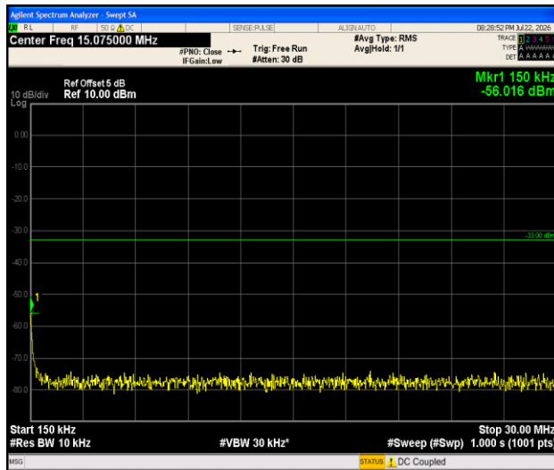
Band4-1.4MHz-16QAM-19957-1RB#0-0.15~30-PASS
