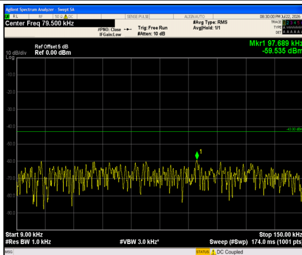
Band4-1.4MHz-QPSK-20175-1RB#0-0.009~0.15-PASS
