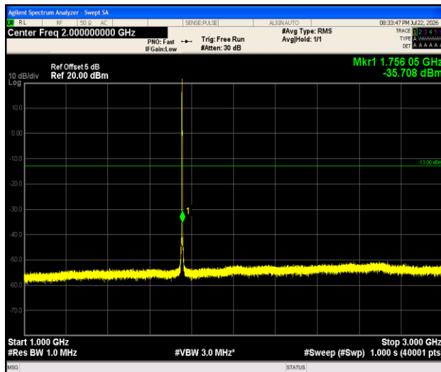
Band4-1.4MHz-16QAM-20393-1RB#0-1000~3000-PASS
