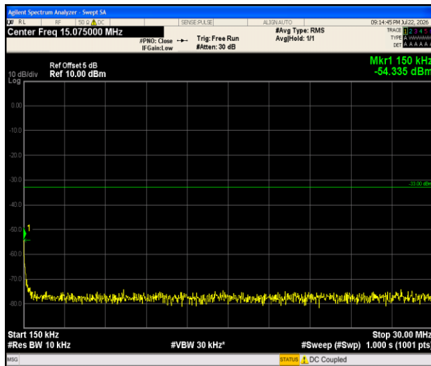
Band4-3MHz-QPSK-19965-1RB#0-0.15~30-PASS
