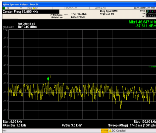
Band4-1.4MHz-16QAM-20393-1RB#0-0.009~0.15-PASS
