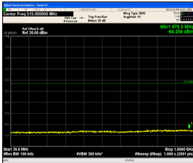
Band4-1.4MHz-16QAM-20393-1RB#0-30~1000-PASS
