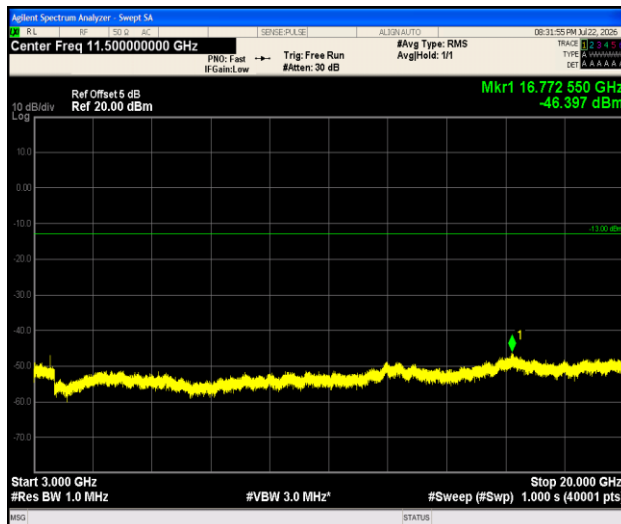
Band4-1.4MHz-16QAM-20175-1RB#0-3000~20000-PASS
