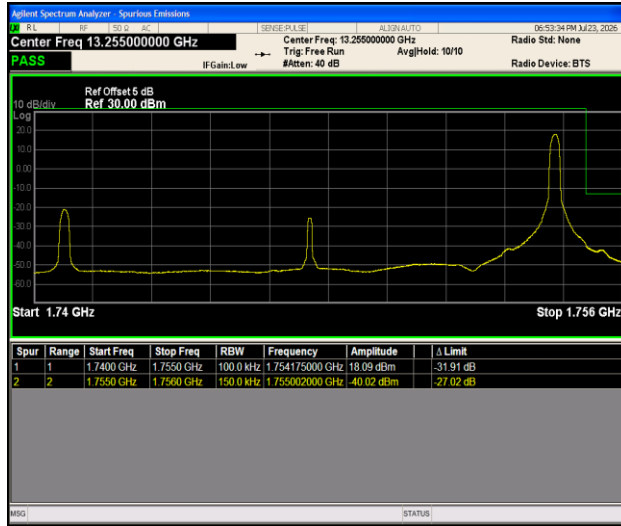
Band4-15MHz-16QAM-20325-1RB#74-PASS
