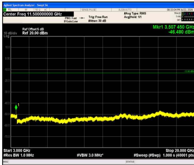
Band4-1.4MHz-QPSK-20393-1RB#0-3000~20000-PASS
