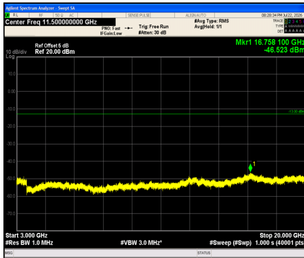
Band4-1.4MHz-QPSK-19957-1RB#0-3000~20000-PASS
