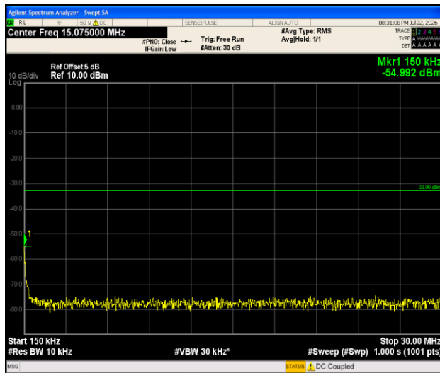
Band4-1.4MHz-16QAM-20175-1RB#0-0.15~30-PASS
