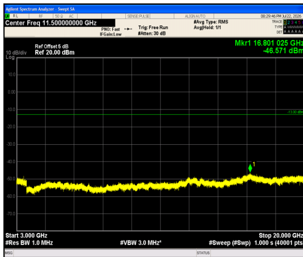
Band4-1.4MHz-16QAM-19957-1RB#0-3000~20000-PASS
