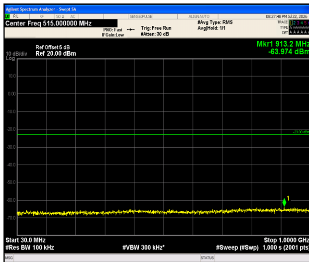
Band4-1.4MHz-QPSK-19957-1RB#0-30~1000-PASS
