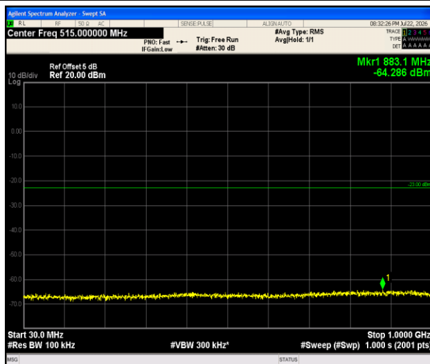
Band4-1.4MHz-QPSK-20393-1RB#0-30~1000-PASS
