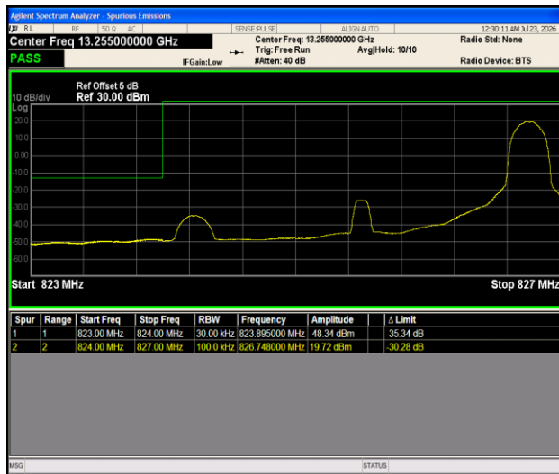
Band5-3MHz-QPSK-20415-1RB#14-PASS
