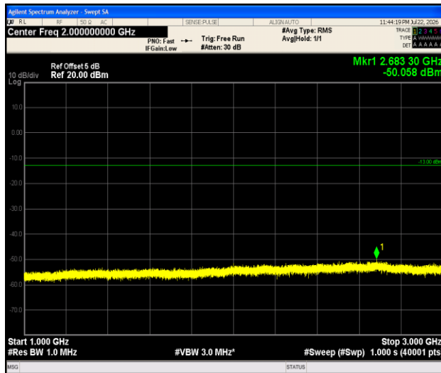
Band5-1.4MHz- 16QAM-20525-1RB#0-1000~3000-PASS
