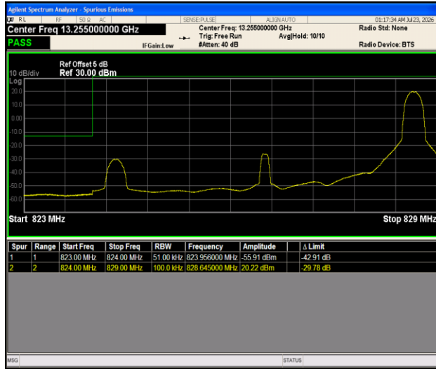
Band5-5MHz- 16QAM-20425-1RB#24-PASS
