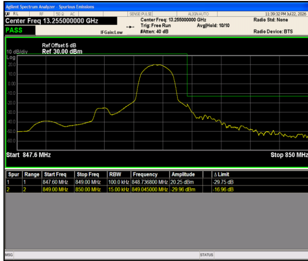
Band5-1.4MHz- 16QAM-20643-1RB#5-PASS
