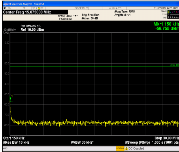
Band5-1.4MHz-QPSK-20525-1RB#0-0.15~30-PASS
