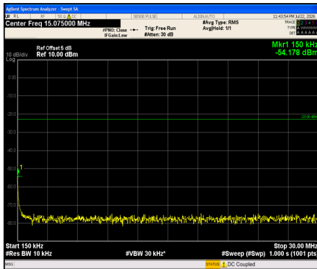
Band5-1.4MHz- 16QAM-20525-1RB#0-0.15~30-PASS
