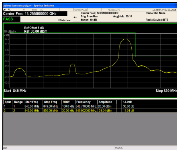
Band5-3MHz-QPSK-20635-1RB#14-PASS
