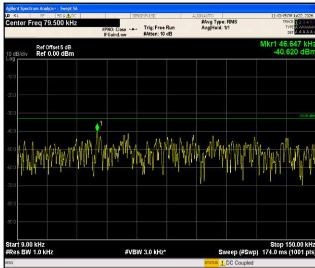
Band5-1.4MHz- 16QAM-20525-1RB#0-0.009~0.15-PASS
