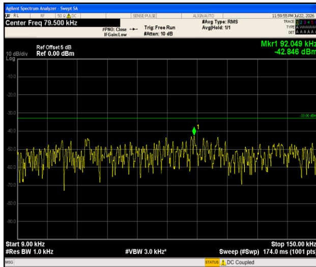
Band5-1.4MHz-QPSK-20643-1RB#0-0.009~0.15-PASS
