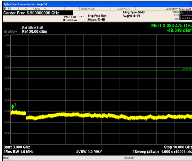
Band5-1.4MHz-QPSK-20525-1RB#0-3000~10000-PASS
