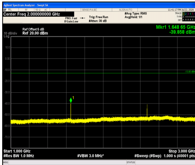
Band5-1.4MHz-QPSK-20407-1RB#0-1000~3000-PASS
