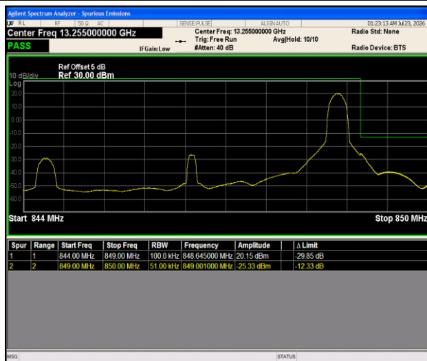
Band5-5MHz-QPSK-20625-1RB#24-PASS
