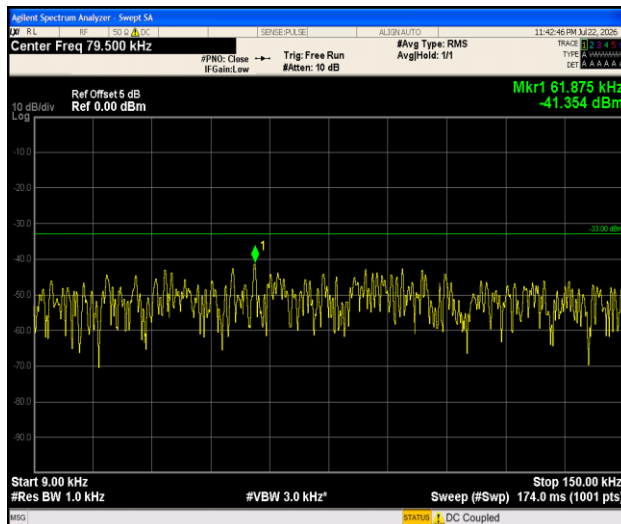
Band5-1.4MHz-QPSK-20525-1RB#0-0.009~0.15-PASS
