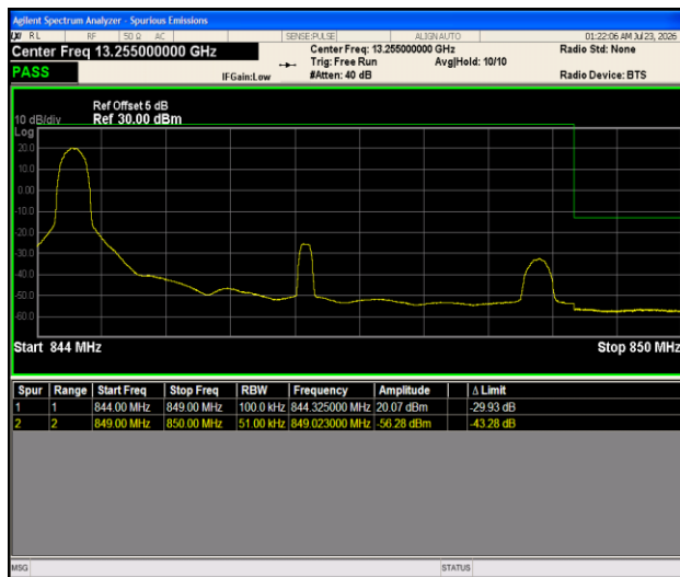
Band5-5MHz- 16QAM-20625-1RB#0-PASS
