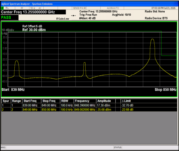
Band5-10MHz-16QAM-20600-1RB#49-PASS
