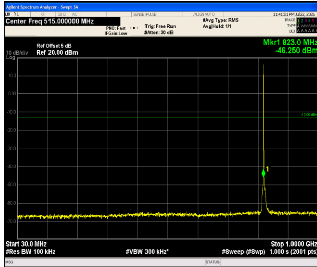
Band5-1.4MHz-QPSK-20407-1RB#0-30~1000-PASS
