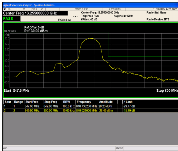
Band5-1.4MHz-QPSK-20643-1RB#5-PASS
