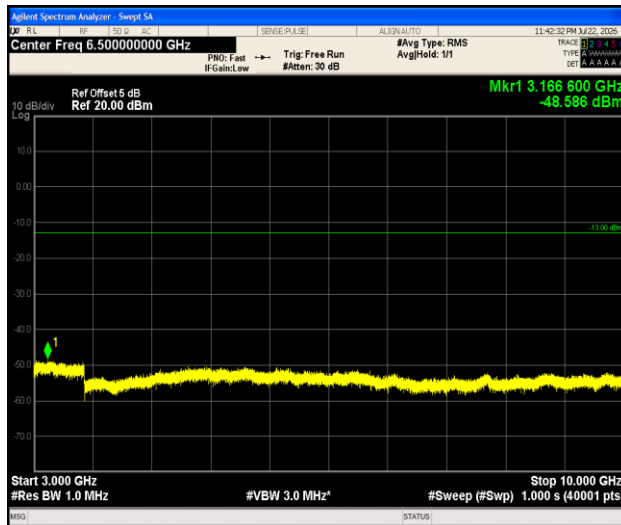
Band5-1.4MHz- 16QAM-20407-1RB#0-3000~10000-PASS
