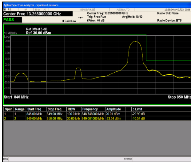
Band5-3MHz- 16QAM-20635-1RB#14-PASS
