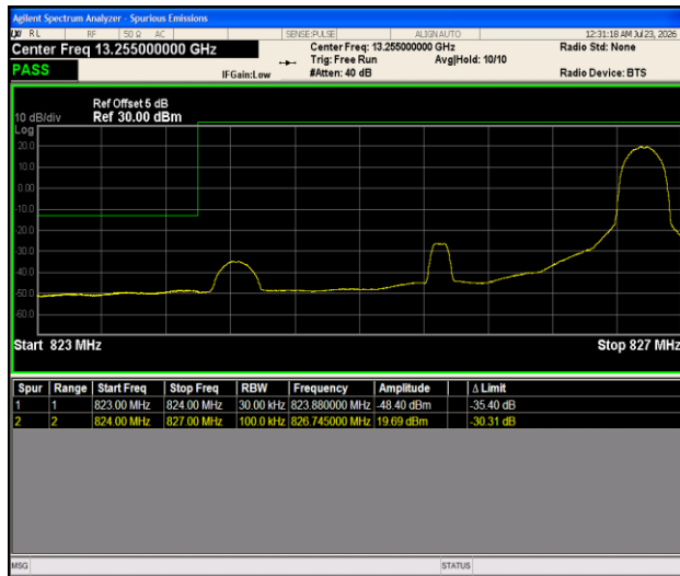
Band5-3MHz- 16QAM-20415-1RB#14-PASS
