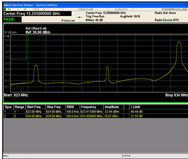
Band5-10MHz-16QAM-20450-1RB#49-PASS
