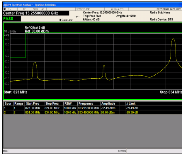
Band5-10MHz-QPSK-20450-1RB#49-PASS
