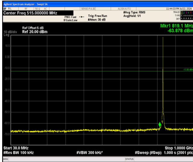
Band5-1.4MHz- 16QAM-20525-1RB#0-30~1000-PASS
