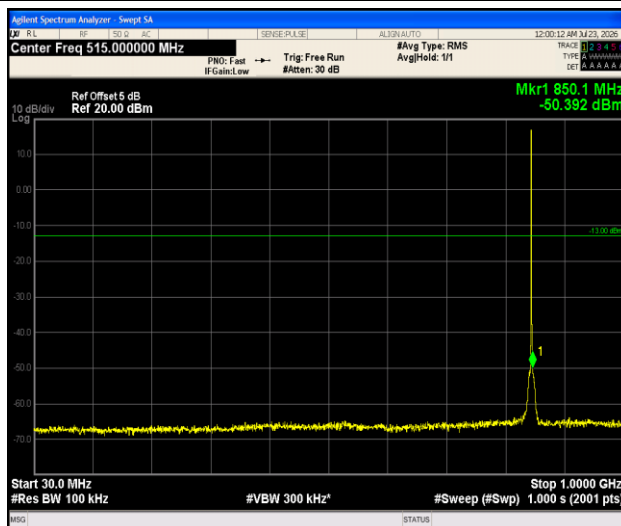
Band5-1.4MHz-QPSK-20643-1RB#0-30~1000-PASS
