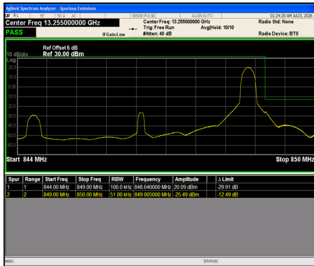
Band5-5MHz- 16QAM-20625-1RB#24-PASS
