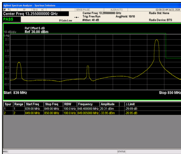
Band5-10MHz-QPSK-20600-1RB#49-PASS
