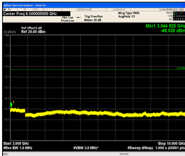
Band5-1.4MHz- 16QAM-20525-1RB#0-3000~10000-PASS
