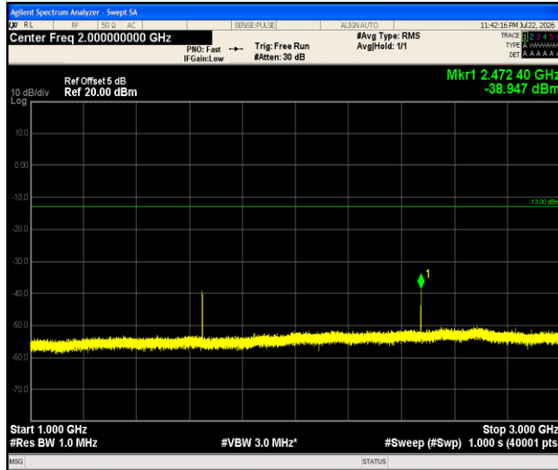
Band5-1.4MHz- 16QAM-20407-1RB#0-1000~3000-PASS
