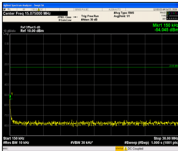
Band5-1.4MHz-QPSK-20643-1RB#0-0.15~30-PASS
