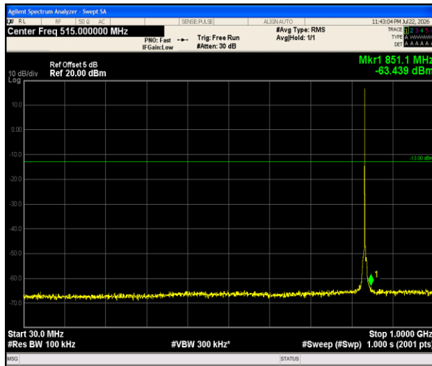
Band5-1.4MHz-QPSK-20525-1RB#0-30~1000-PASS
