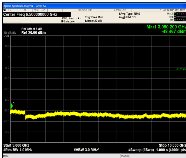
Band5-1.4MHz-QPSK-20407-1RB#0-3000~10000-PASS
