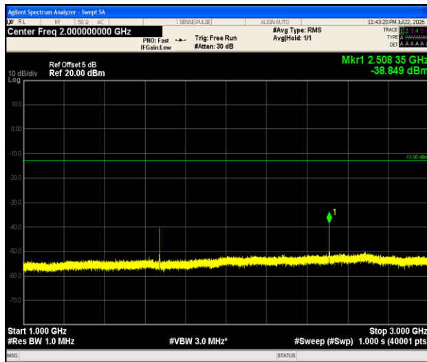
Band5-1.4MHz-QPSK-20525-1RB#0-1000~3000-PASS
