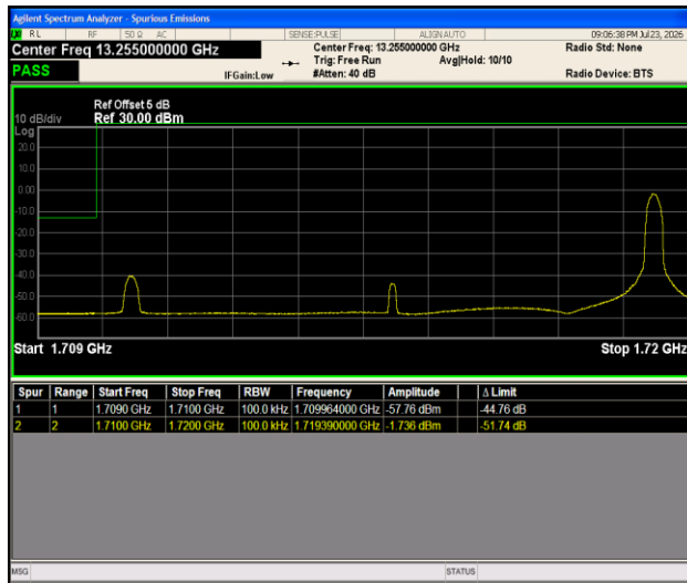
Band66-10MHz-QPSK-132022-1RB#49-PASS
