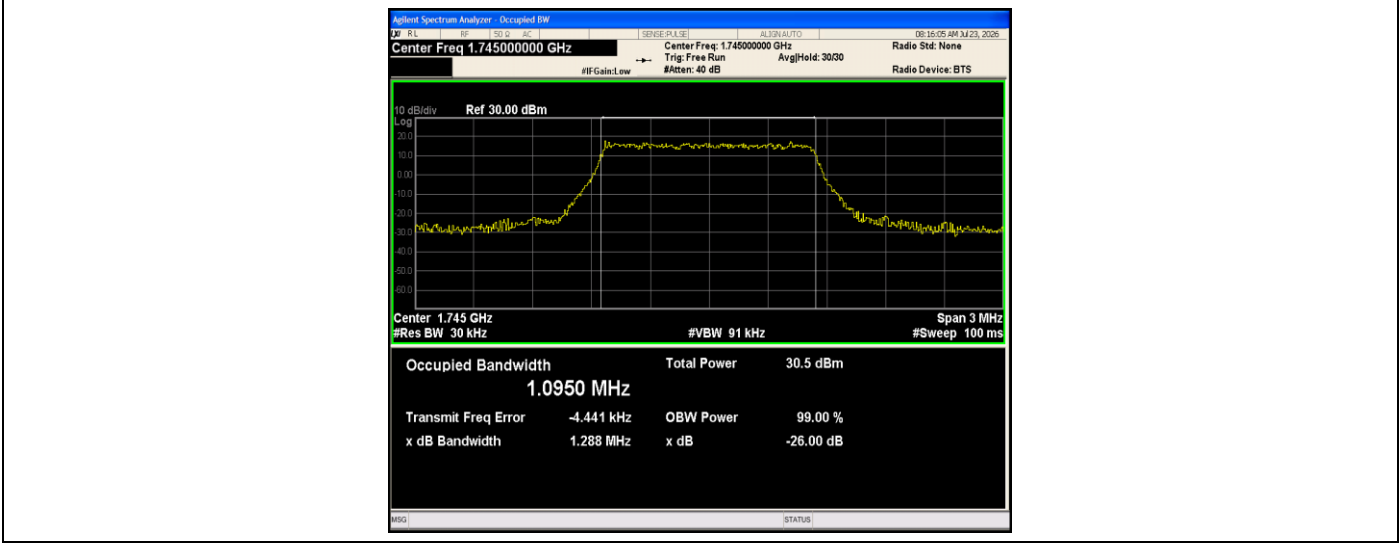
Band66-1.4MHz-QPSK-132322-6RB#0-PASS
