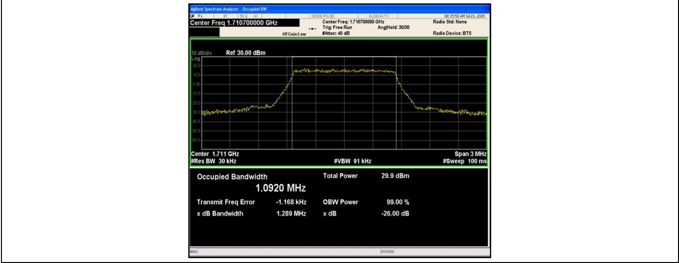
Band66-1.4MHz-16QAM-131979-6RB#0-PASS
