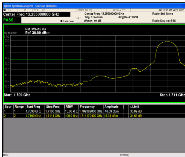
Band66-1.4MHz-16QAM-131979-1RB#5-PASS
