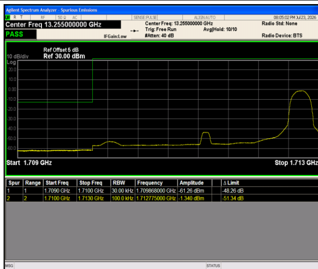
Band66-3MHz-16QAM-131987-1RB#14-PASS
