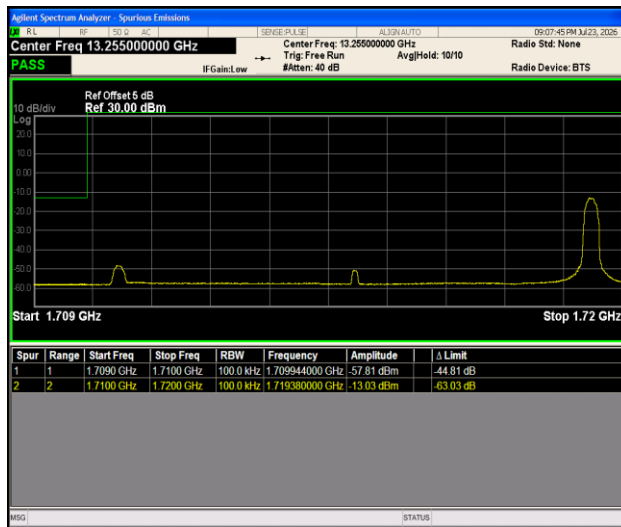
Band66-10MHz-16QAM-132022-1RB#49-PASS
