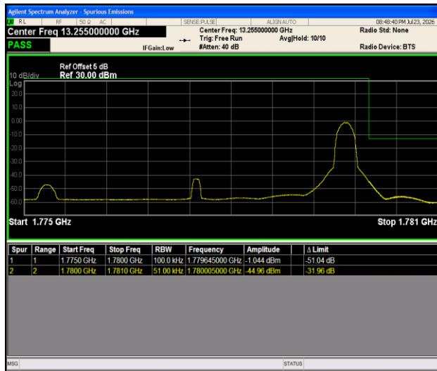
Band66-5MHz-QPSK-132647-1RB#24-PASS
