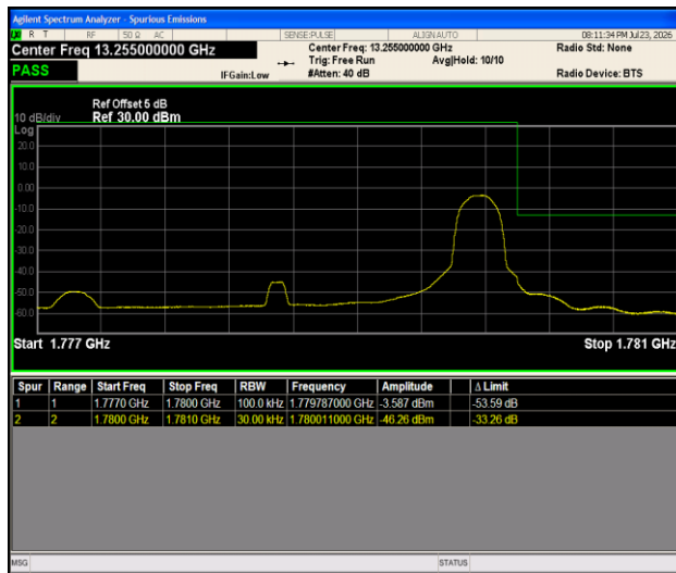
Band66-3MHz-16QAM-132657-1RB#14-PASS
