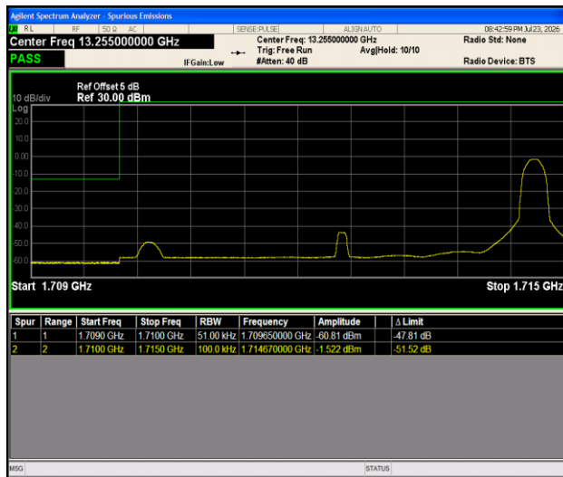
Band66-5MHz-16QAM-131997-1RB#24-PASS
