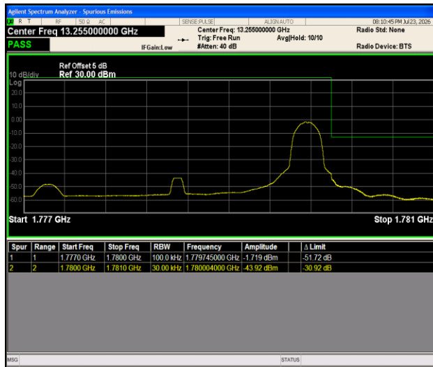
Band66-3MHz-QPSK-132657-1RB#14-PASS
