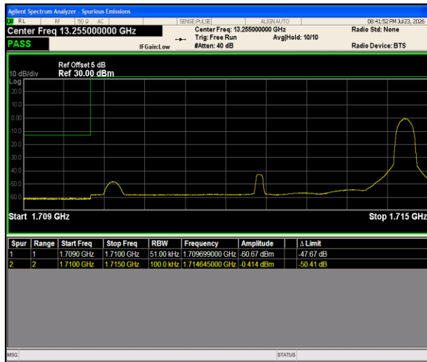
Band66-5MHz-QPSK-131997-1RB#24-PASS
