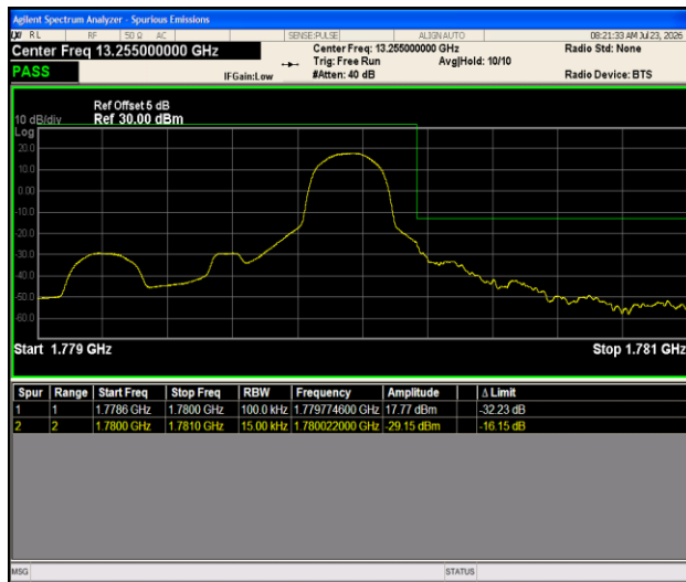
Band66-1.4MHz-16QAM-132665-1RB#5-PASS
