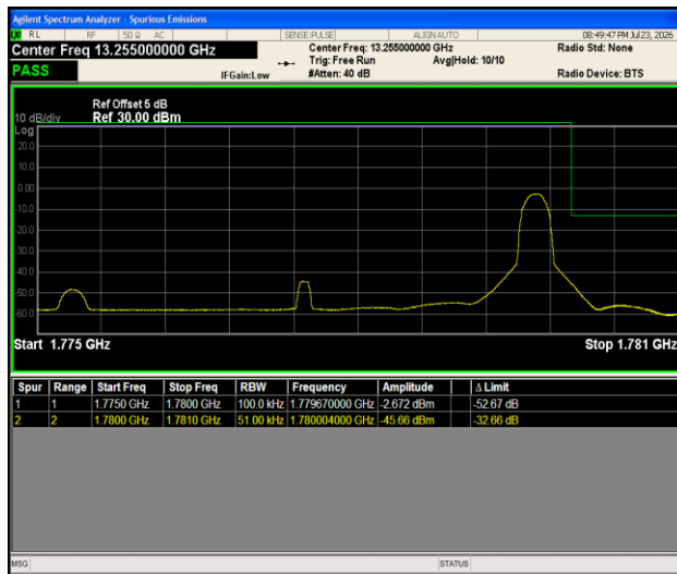
Band66-5MHz-16QAM-132647-1RB#24-PASS
