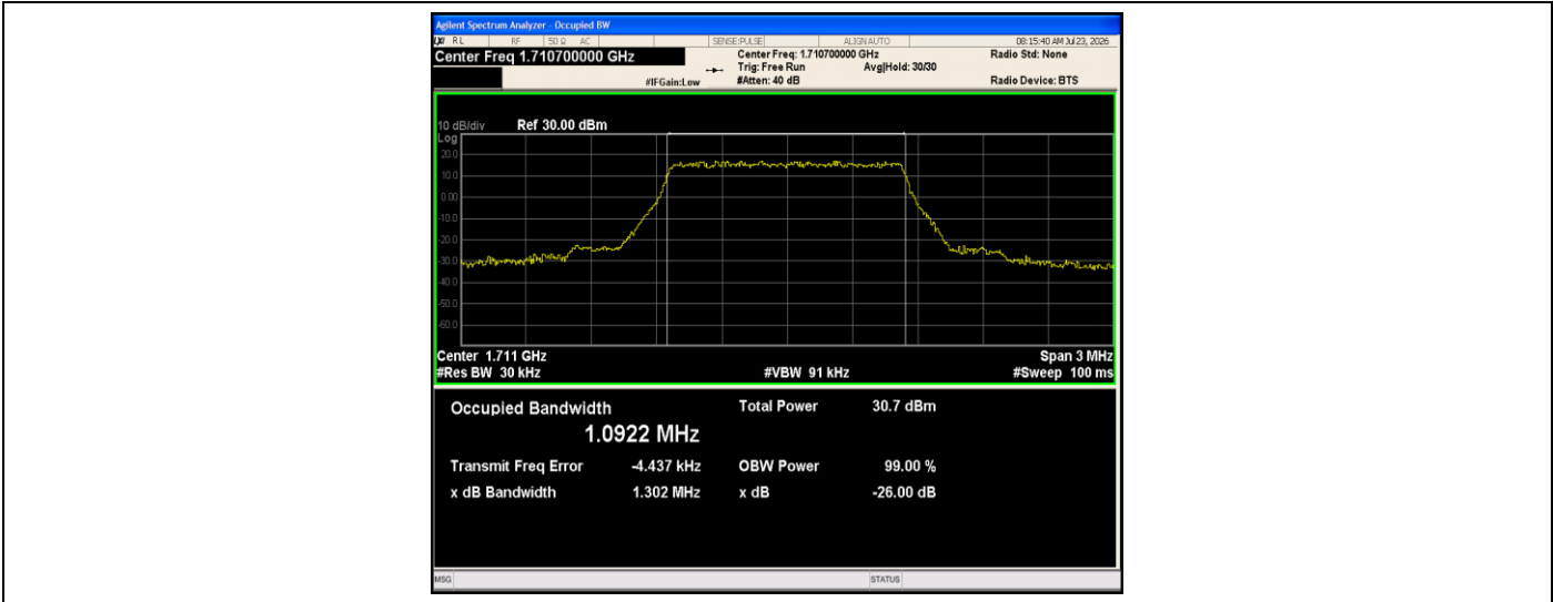
Band66-1.4MHz-QPSK-131979-6RB#0-PASS
