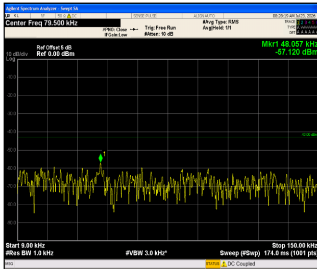
Band66-1.4MHz-16QAM-132665-1RB#0-0.009~0.15-PASS
