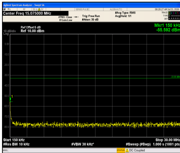
Band66-1.4MHz-16QAM-132665-1RB#0-0.15~30-PASS
