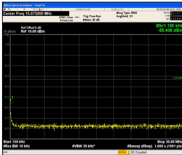
Band66-1.4MHz-QPSK-132322-1RB#0-0.15~30-PASS
