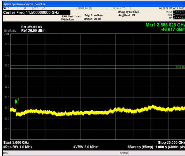
Band66-1.4MHz-QPSK-132665-1RB#0-3000~20000-PASS
