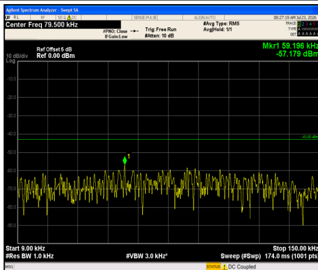
Band66-1.4MHz-QPSK-132665-1RB#0-0.009~0.15-PASS
