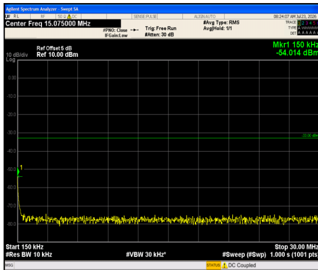
Band66-1.4MHz-16QAM-131979-1RB#0-0.15~30-PASS
