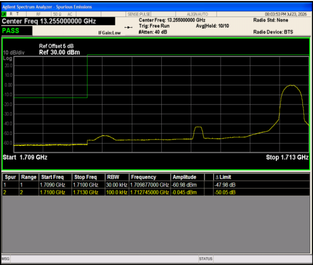
Band66-3MHz-QPSK-131987-1RB#14-PASS
