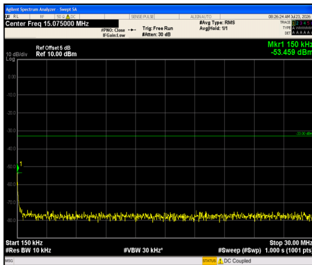
Band66-1.4MHz-16QAM-132322-1RB#0-0.15~30-PASS
