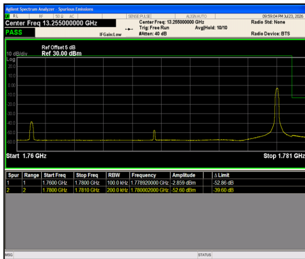
Band66-20MHz-16QAM-132572-1RB#99-PASS
