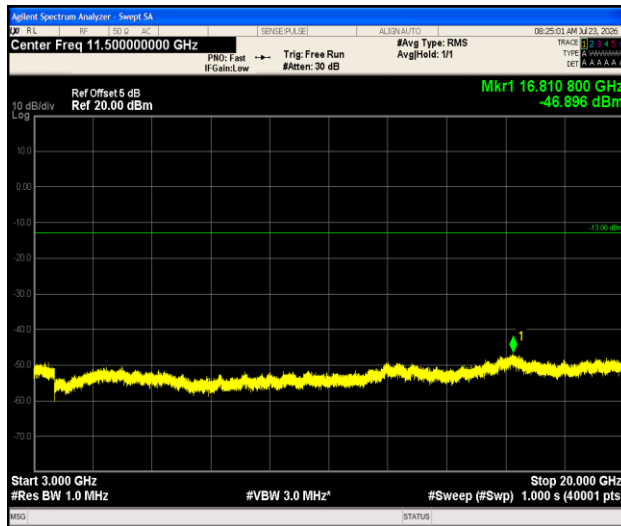
Band66-1.4MHz-16QAM-131979-1RB#0-3000~20000-PASS
