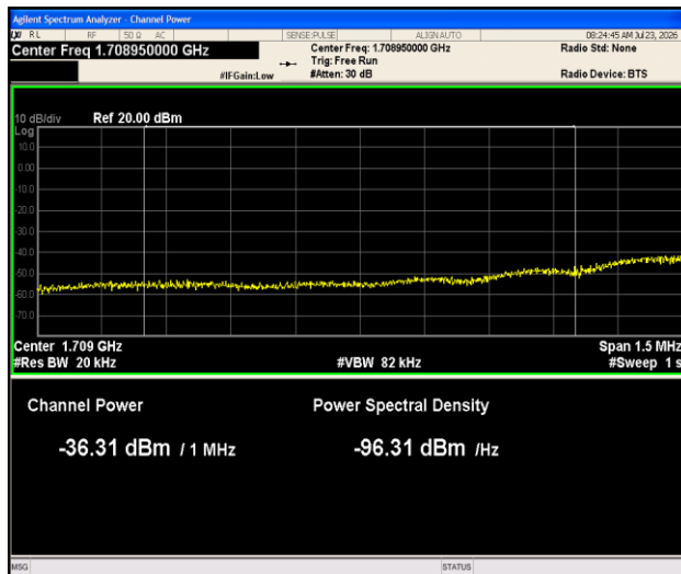
Band66-1.4MHz-16QAM-131979-1RB#0-1000~3000- PASS-Final
