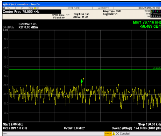
Band66-1.4MHz-16QAM-132322-1RB#0-0.009~0.15-PASS
