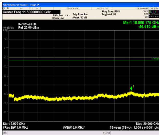
Band66-1.4MHz-16QAM-132322-1RB#0-3000~20000-PASS
