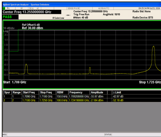
Band66-15MHz-QPSK-132047-1RB#74-PASS
