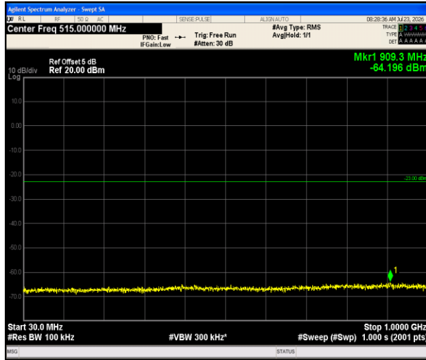
Band66-1.4MHz-16QAM-132665-1RB#0-30~1000-PASS
