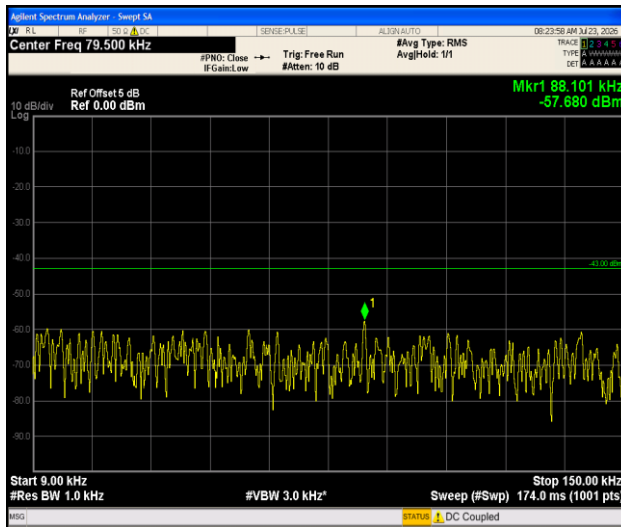
Band66-1.4MHz-16QAM-131979-1RB#0-0.009~0.15-PASS
