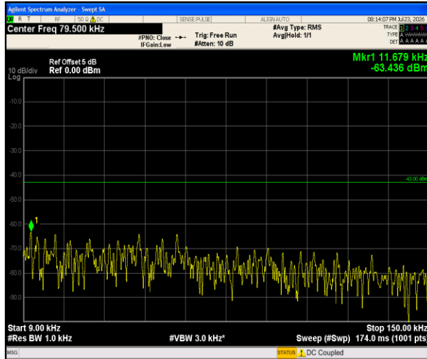
Band66-3MHz-QPSK-131987-1RB#0-0.009~0.15-PASS
