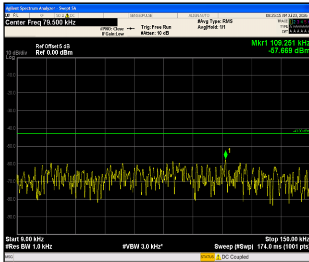
Band66-1.4MHz-QPSK-132322-1RB#0-0.009~0.15-PASS
