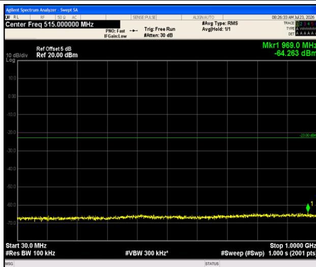
Band66-1.4MHz-16QAM-132322-1RB#0-30~1000-PASS
