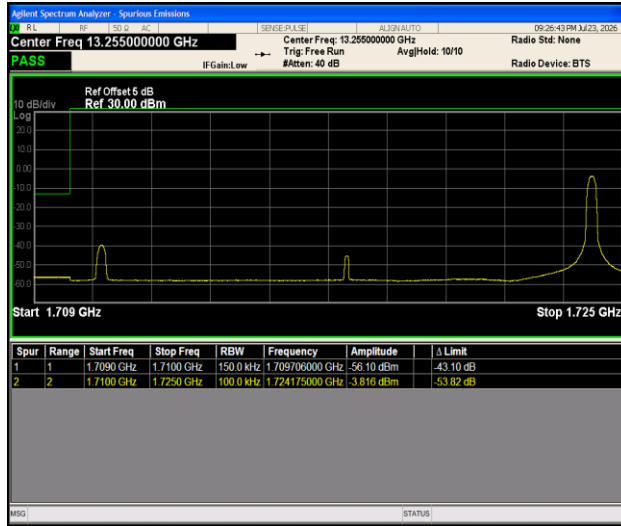
Band66-15MHz-16QAM-132047-1RB#74-PASS
