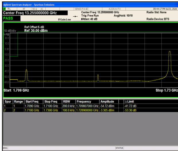
Band66-20MHz-16QAM-132072-1RB#99-PASS
