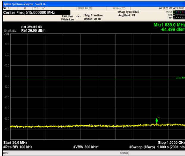
Band66-1.4MHz-QPSK-131979-1RB#0-30~1000-PASS
