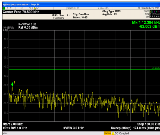
Band66-3MHz-16QAM-131987-1RB#0-0.009~0.15-PASS
