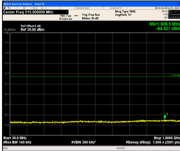
Band66-1.4MHz-16QAM-131979-1RB#0-30~1000-PASS
