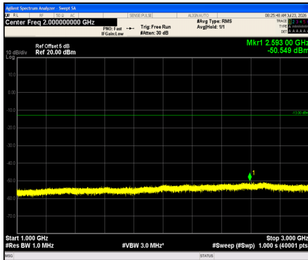
Band66-1.4MHz-QPSK-132322-1RB#0-1000~3000-PASS
