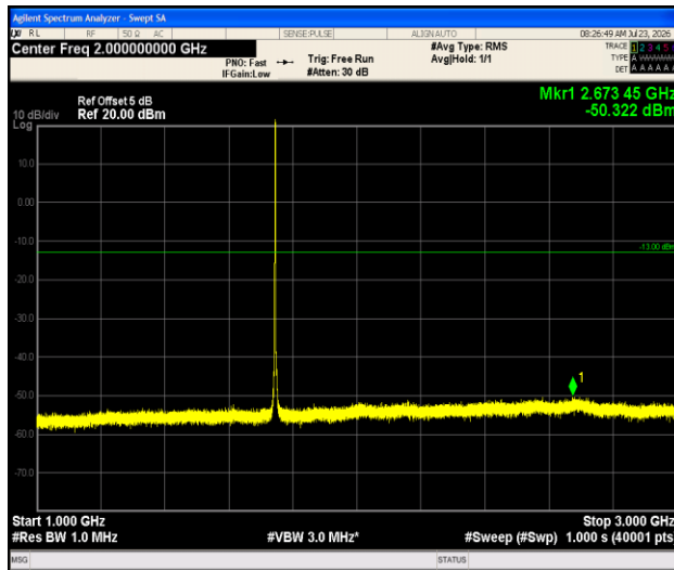
Band66-1.4MHz-16QAM-132322-1RB#0-1000~3000-PASS
