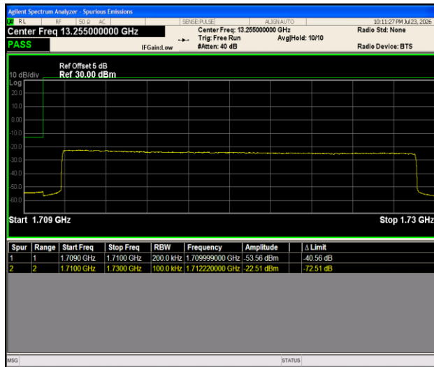
Band66-20MHz-QPSK-132072-100RB#0-PASS
