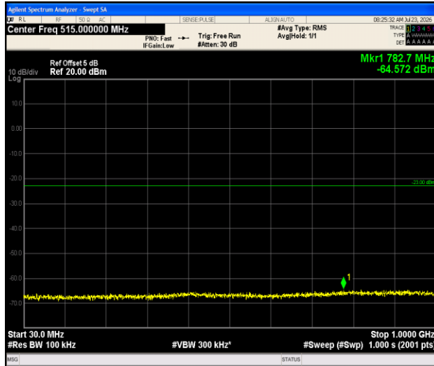
Band66-1.4MHz-QPSK-132322-1RB#0-30~1000-PASS
