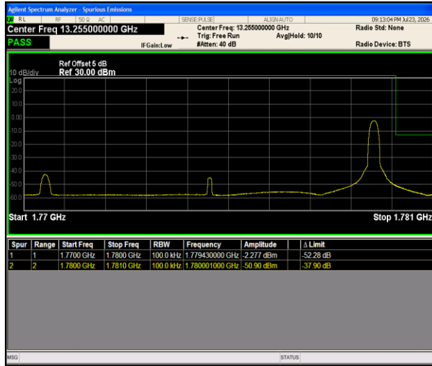
Band66-10MHz-16QAM-132622-1RB#49-PASS
