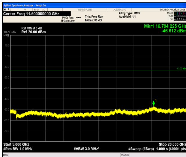
Band66-1.4MHz-QPSK-132322-1RB#0-3000~20000-PASS
