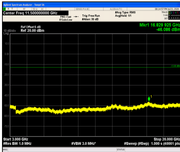
Band66-3MHz-QPSK-131987-1RB#0-3000~20000-PASS
