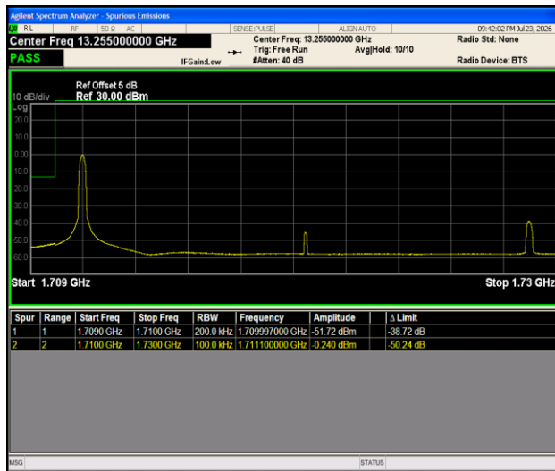
Band66-20MHz-16QAM-132072-1RB#0-PASS
