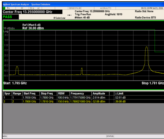
Band66-15MHz-16QAM-132597-1RB#74-PASS
