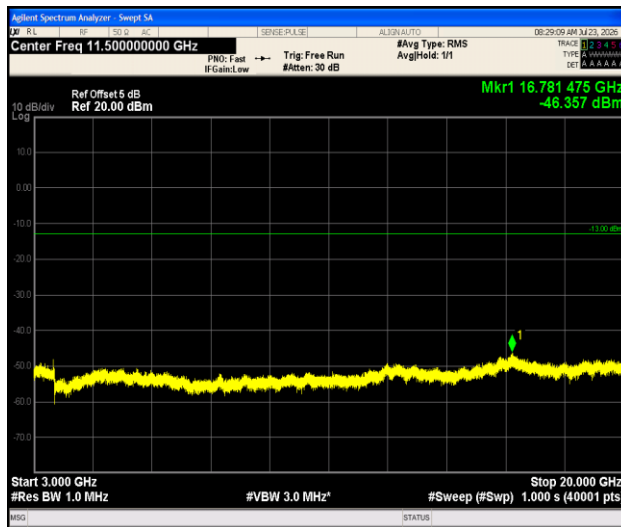
Band66-1.4MHz-16QAM-132665-1RB#0-3000~20000-PASS
