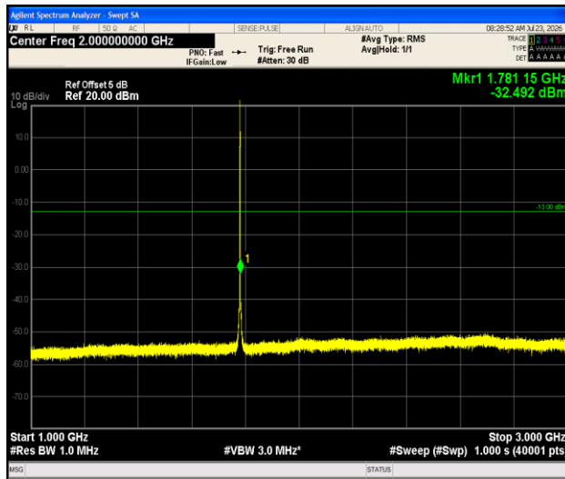
Band66-1.4MHz-16QAM-132665-1RB#0-1000~3000-PASS
