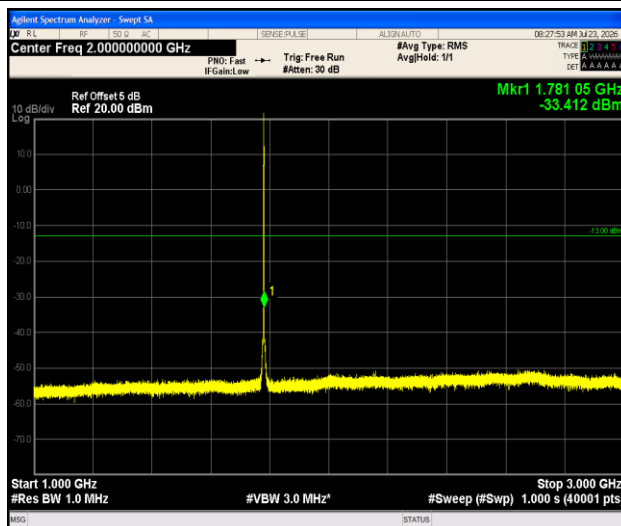
Band66-1.4MHz-QPSK-132665-1RB#0-1000~3000-PASS
