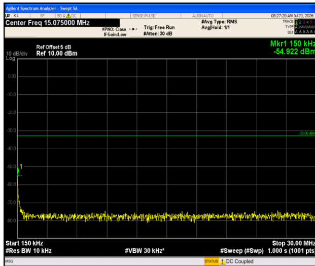
Band66-1.4MHz-QPSK-132665-1RB#0-0.15~30-PASS
