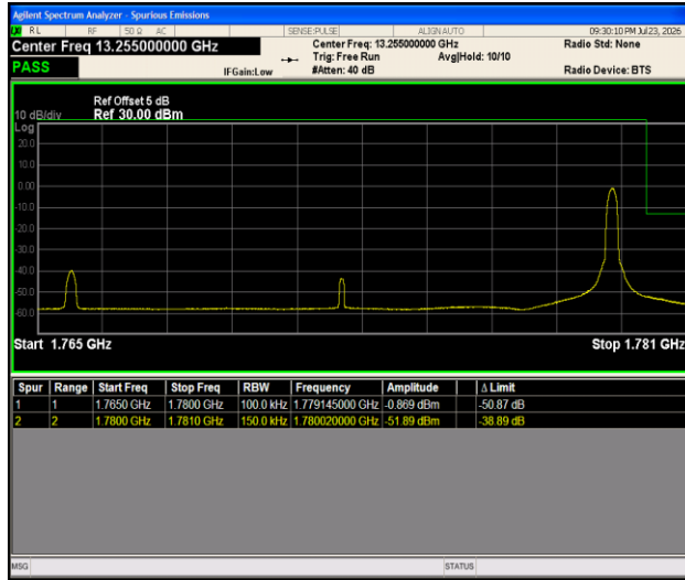
Band66-15MHz-QPSK-132597-1RB#74-PASS
