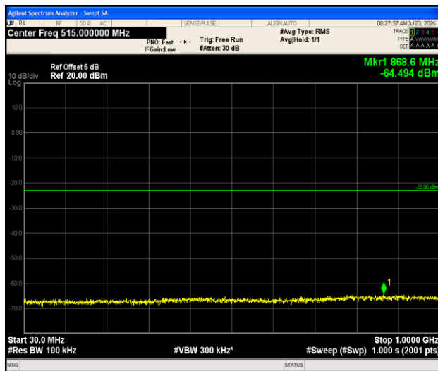
Band66-1.4MHz-QPSK-132665-1RB#0-30~1000-PASS
