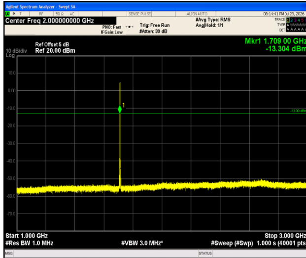
Band66-3MHz-QPSK-131987-1RB#0-1000~3000-PASS
