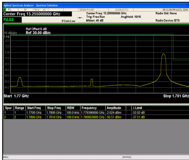
Band66-10MHz-QPSK-132622-1RB#49-PASS
