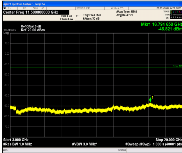
Band66-1.4MHz-QPSK-131979-1RB#0-3000~20000-PASS
