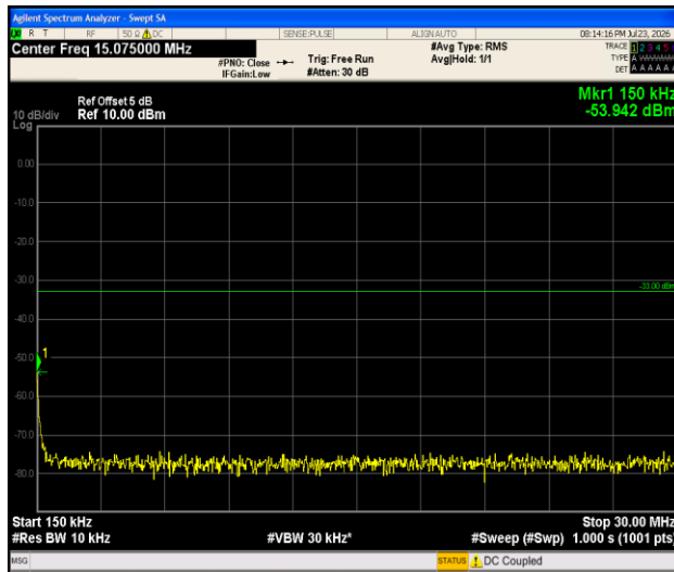
Band66-3MHz-QPSK-131987-1RB#0-0.15~30-PASS
