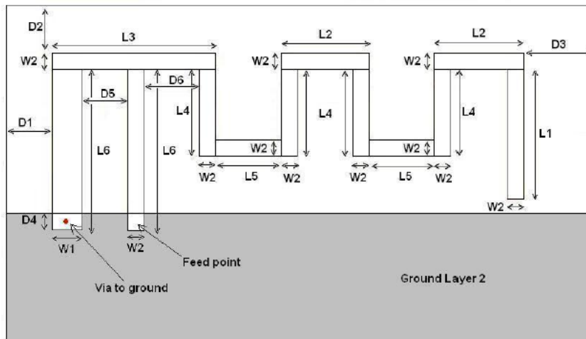
Figure 3: Antenna Dimensions
