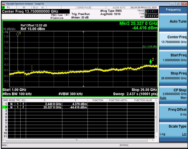
LE_1M-Ant1-2440-1000~26500-PASS
