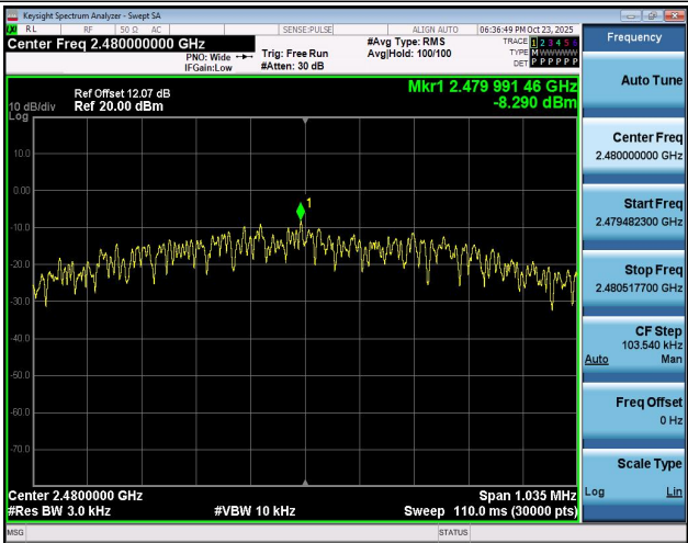
LE_1M-Ant1-2480-PASS
