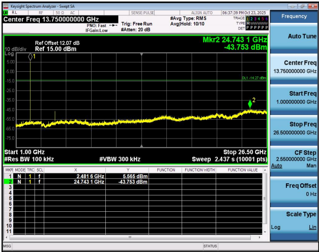
LE_1M-Ant1-2480-1000~26500-PASS
