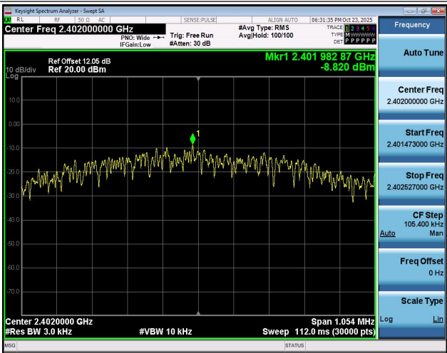
LE_1M-Ant1-2402-PASS
