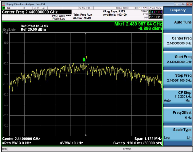
LE_1M-Ant1-2440-PASS
