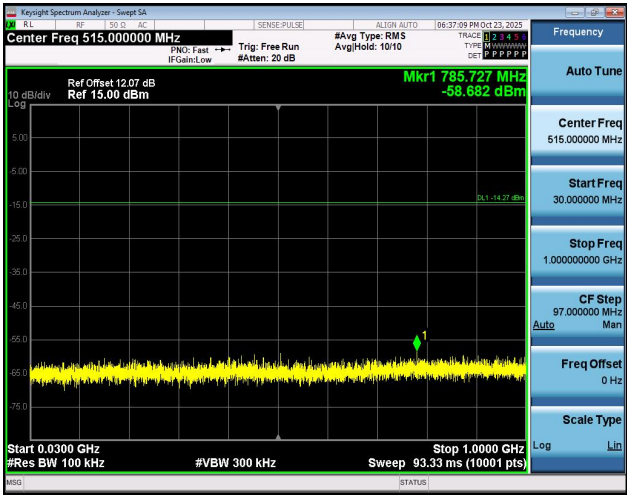
LE_1M-Ant1-2480-30~1000-PASS
