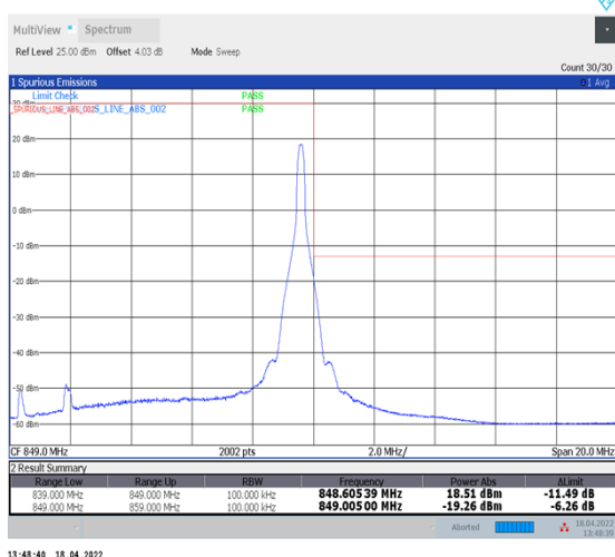
1-N5--15-10-H-5-CP-QPSK-Edge_1RB_Right-1@51-Ant1-seegraph-PASS-see graph
