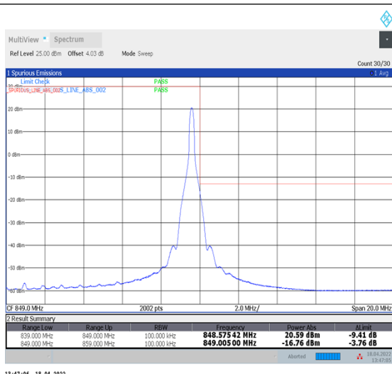
1-N5--15-10-H-2-DFT-PI2BPSK-Edge_1RB_Right-1@51-Ant1-seegraph-PASS-see graph
