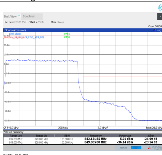
1-N5--15-10-H-3-DFT-PI2BPSK-Outer_Full-50@0-Ant1-seegraph-PASS-see graph
