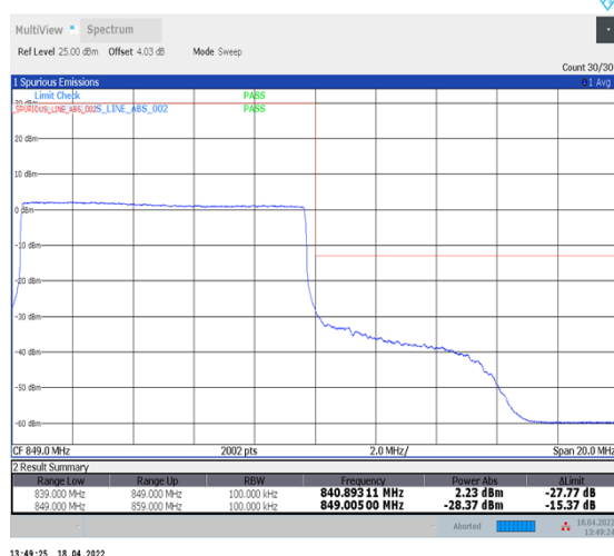
1-N5--15-10-H-6-CP-QPSK-Outer_Full-52@0-Ant1-seegraph-PASS-see graph
