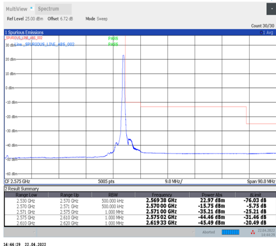
1-N7--15-40-H-2-DFT-PI2BPSK-Edge_1RB_Right-1@215-Ant1-PASS-see graph
