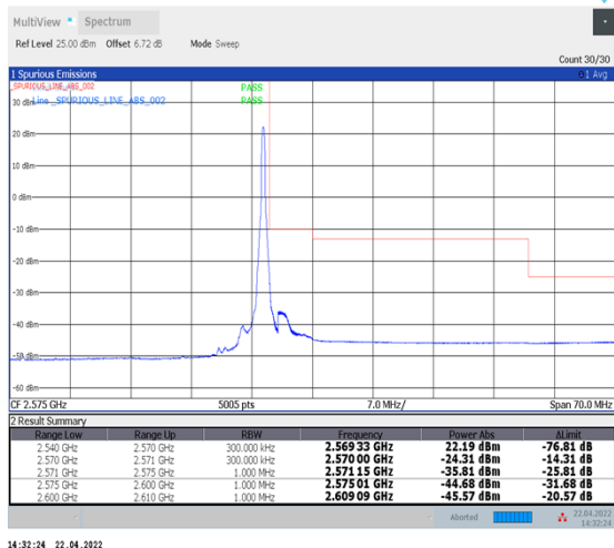
1-N7--15-30-H-2-DFT-PI2BPSK-Edge_1RB_Right-1@159-Ant1-PASS-see graph
