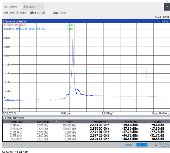
1-N7--15-30-H-5-CP-QPSK-Edge_1RB_Right-1@159-Ant1-PASS-see graph
