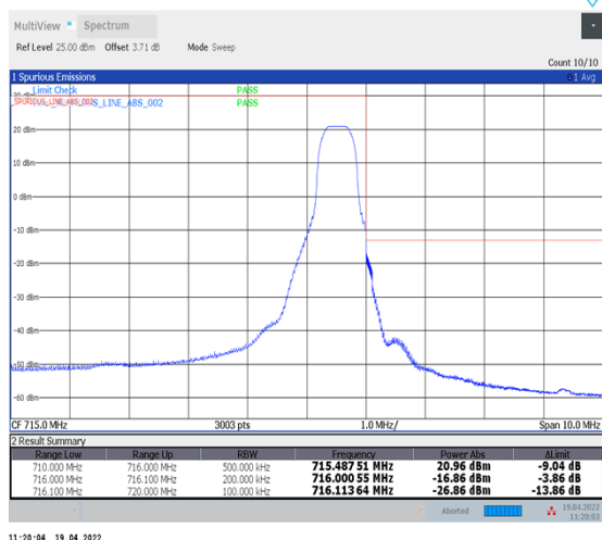
1-N12--15-15-H-5-CP-QPSK-Edge_1RB_Right-1@78-Ant1-PASS-see graph
