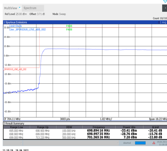
1-N12--15-15-L-6-CP-QPSK-Outer_Full-79@0-Ant1-PASS-see graph
