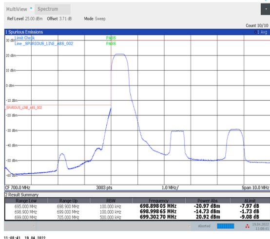
1-N12--15-5-L-4-CP-QPSK-Edge_1RB_Left-1@0-Ant1-PASS-see graph
