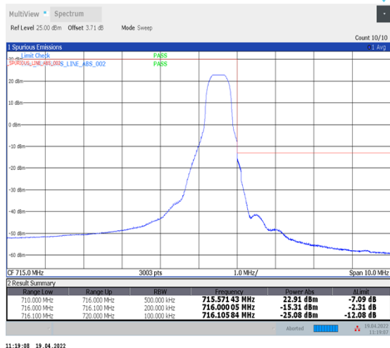
1-N12--15-15-H-2-DFT-PI2BPSK-Edge_1RB_Right-1@78-Ant1-PASS-see graph
