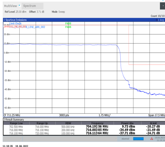
1-N12--15-15-H-3-DFT-PI2BPSK-Outer_Full-75@0-Ant1-PASS-see graph
