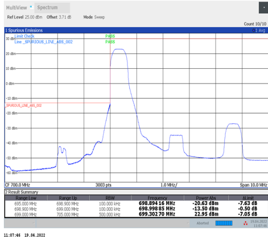
1-N12--15-5-L-1-DFT-PI2BPSK-Edge_1RB_Left-1@0-Ant1-PASS-see graph
