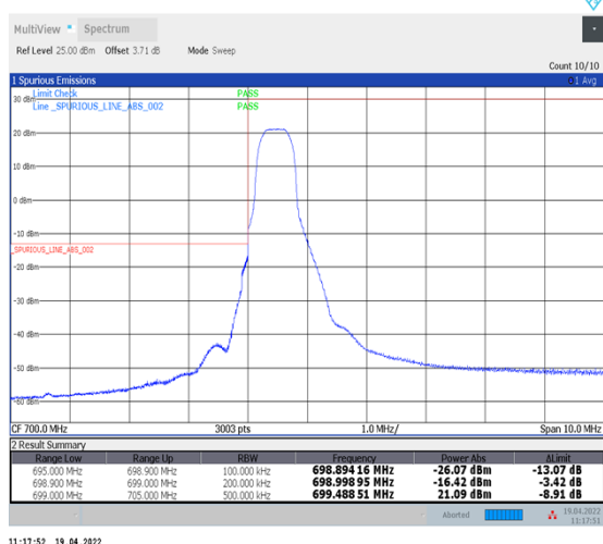
1-N12--15-15-L-4-CP-QPSK-Edge_1RB_Left-1@0-Ant1-PASS-see graph
