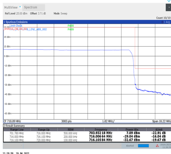
1-N12--15-15-H-6-CP-QPSK-Outer_Full-79@0-Ant1-PASS-see graph
