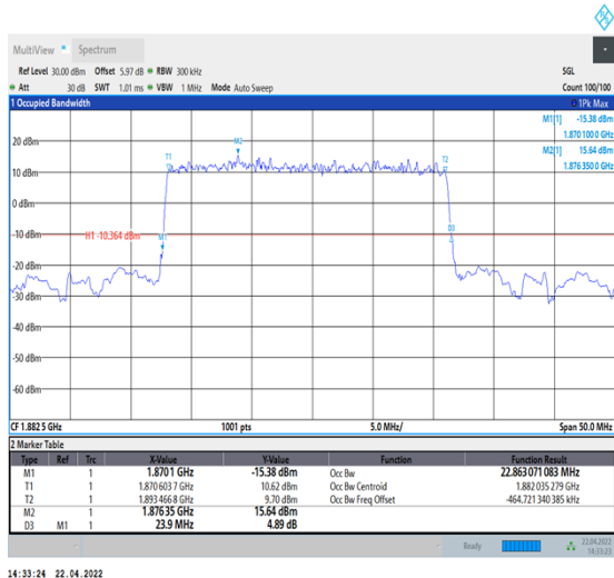
1-N25--15-25-M-2-DFT-PI2BPSK-Outer_Full-128@0-Ant1-22.863-23.900-≤25-PASS
