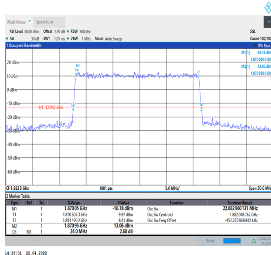
1-N25--15-25-M-3-DFT-16QAM-Outer_Full-128@0-Ant1-22.883-24.000-≤25-PASS
