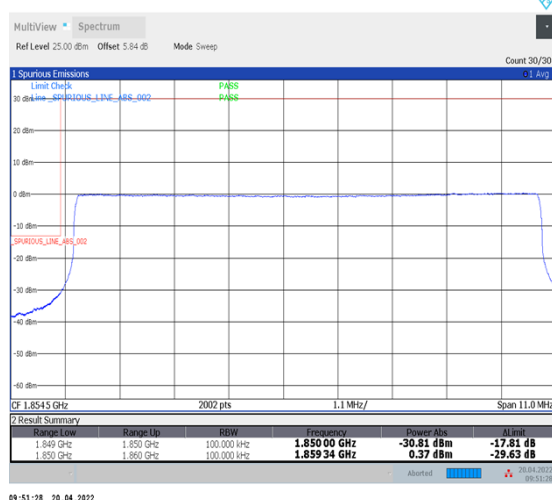
1-N25--15-10-L-6-CP-QPSK-Outer_Full-52@0-Ant1-seegraph-PASS-see graph
