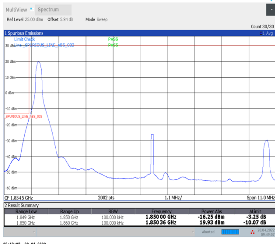
1-N25--15-10-L-1-DFT-PI2BPSK-Edge_1RB_Left-1@0-Ant1-seegraph-PASS-see graph
