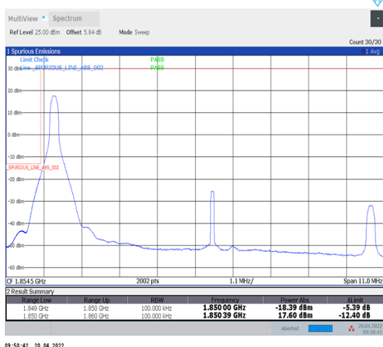
1-N25--15-10-L-4-CP-QPSK-Edge_1RB_Left-1@0-Ant1-seegraph-PASS-see graph
