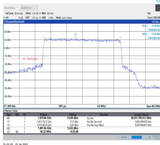
1-N25--15-40-H-4-DFT-64QAM-Outer_Full-216@0-Ant1-38.552-40.320-≤40-PASS
