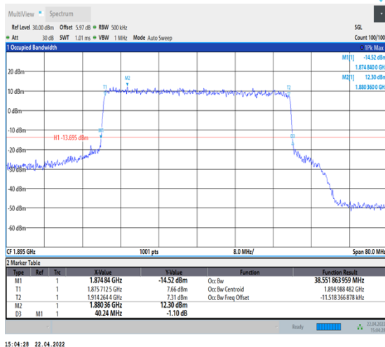
1-N25--15-40-H-7-CP-16QAM-Outer_Full-216@0-Ant1-38.552-40.240-≤40-PASS
