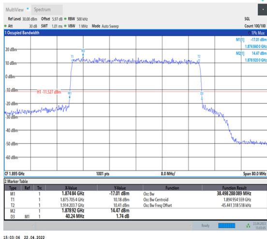
1-N25--15-40-H-1-DFT-QPSK-Outer_Full-216@0-Ant1-38.498-40.240-≤40-PASS
