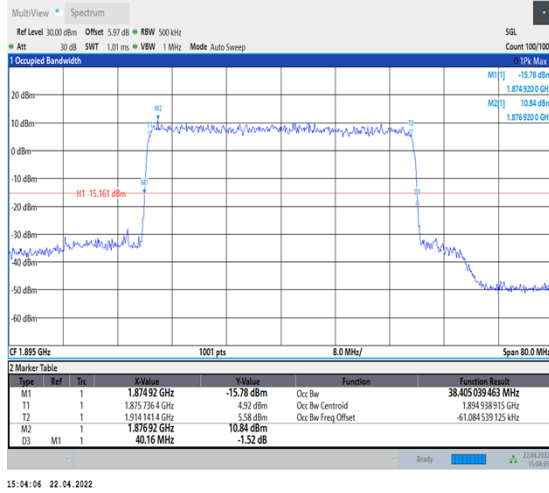
1-N25--15-40-H-5-DFT-256QAM-Outer_Full-216@0-Ant1-38.405-40.160-≤40-PASS
