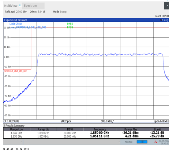
1-N25--15-5-L-3-DFT-PI2BPSK-Outer_Full-25@0-Ant1-seegraph-PASS-see graph
