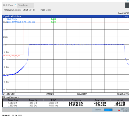
1-N25--15-5-L-6-CP-QPSK-Outer_Full-25@0-Ant1-seegraph-PASS-see graph
