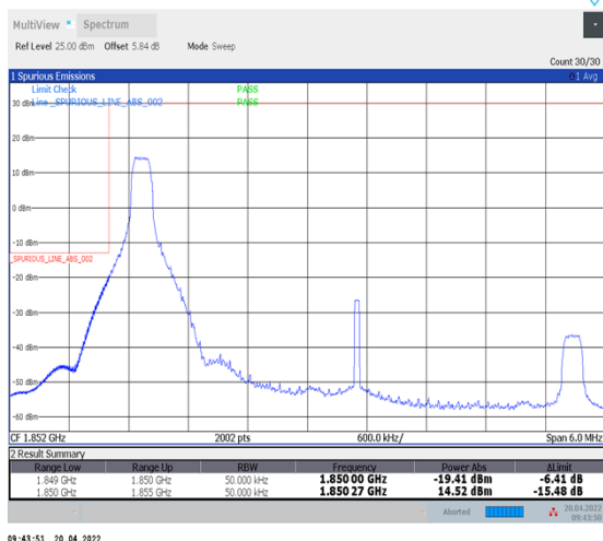
1-N25--15-5-L-4-CP-QPSK-Edge_1RB_Left-1@0-Ant1-seegraph-PASS-see graph
