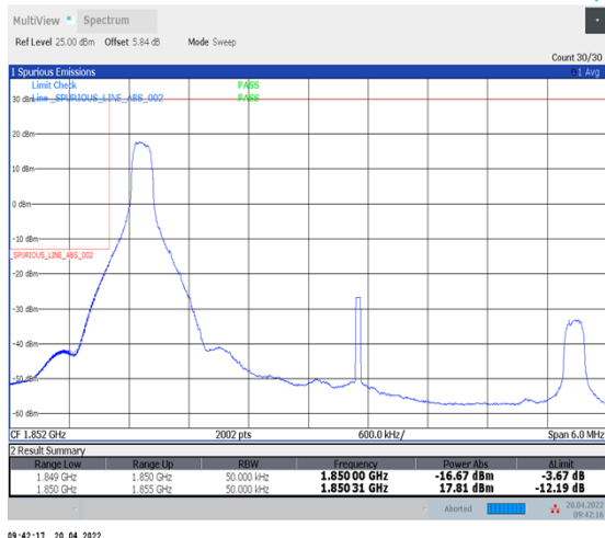
1-N25--15-5-L-1-DFT-PI2BPSK-Edge_1RB_Left-1@0-Ant1-seegraph-PASS-see graph
