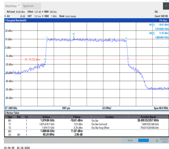
1-N25--15-40-H-8-CP-64QAM-Outer_Full-216@0-Ant1-38.499-40.240-≤40-PASS
