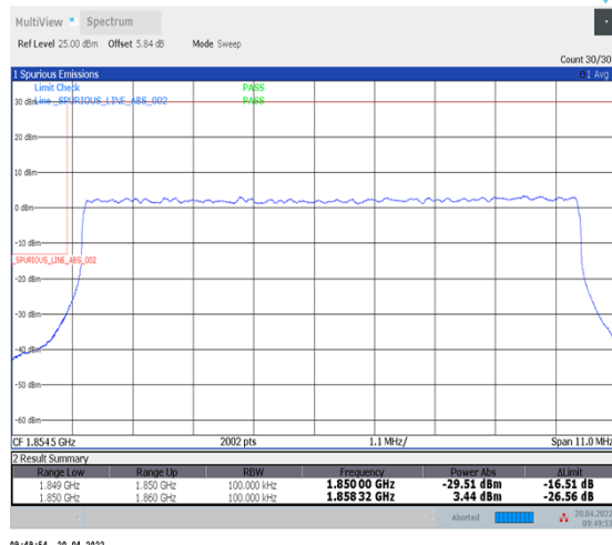
1-N25--15-10-L-3-DFT-PI2BPSK-Outer_Full-50@0-Ant1-seegraph-PASS-see graph
