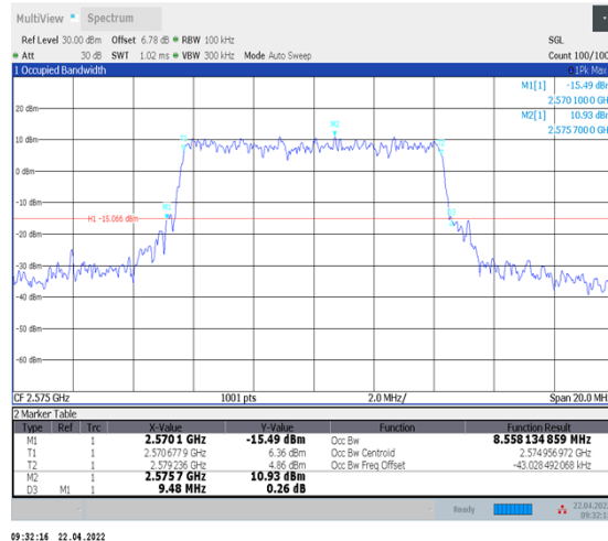
1-N38--30-10-L-4-DFT-64QAM-Outer_Full-24@0- Ant1-8.558-9.480-≤10-PASS
