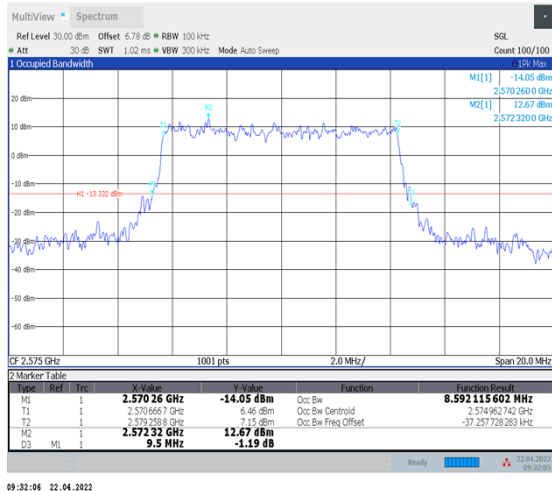
1-N38--30-10-L-3-DFT-16QAM-Outer_Full-24@0- Ant1-8.592-9.500-≤10-PASS
