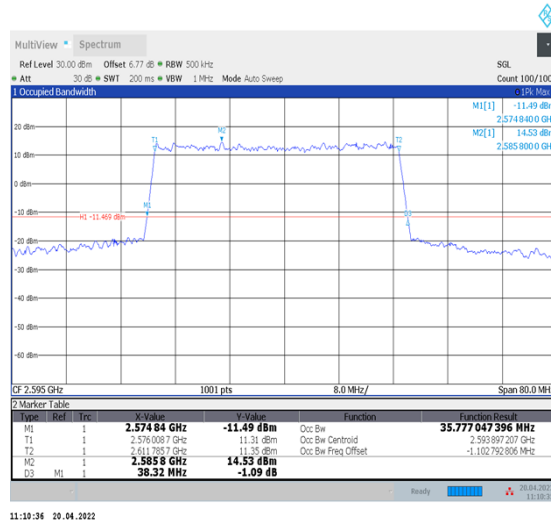
1-N38--30-40-M-3-DFT-16QAM-Out_ Full-100@0-Ant1-35.777-38.320-≤40-PASS
