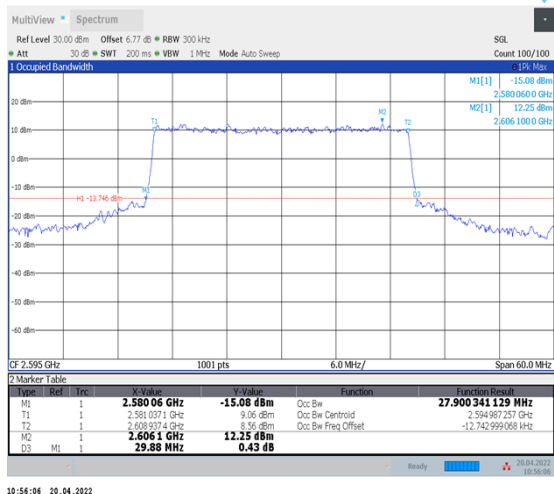
1-N38--30-30-M-7-CP-16QAM-Outer_Full-78@0- Ant1-27.9-29.880-≤30-PASS
