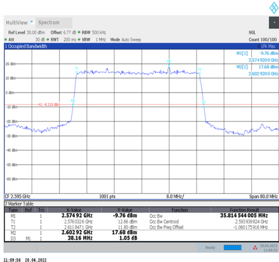
1-N38--30-40-M-2-DFT-PI2BPSK-Out_ Full-100@0-Ant1-35.815-38.160-≤40-PASS
