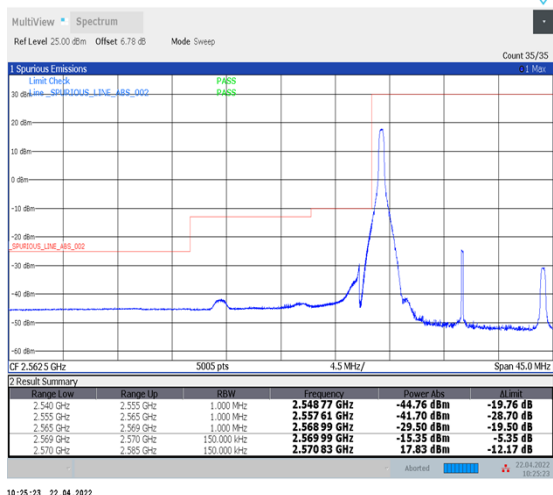
1-N38--30-15-L-4-CP-QPSK-Edge_1RB_Left-1@0-Ant1-PASS-see graph
