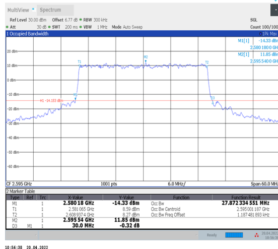
1-N38--30-30-M-8-CP-64QAM-Outer_Full-78@0- Ant1-27.872-30.000-≤30-PASS
