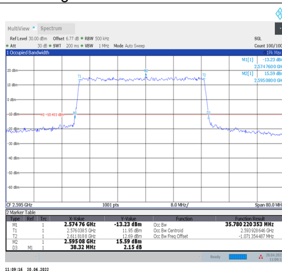
1-N38--30-40-M-1-DFT-QPSK-Out_ Full-100@0-Ant1-35.78-38.320-≤40-PASS
