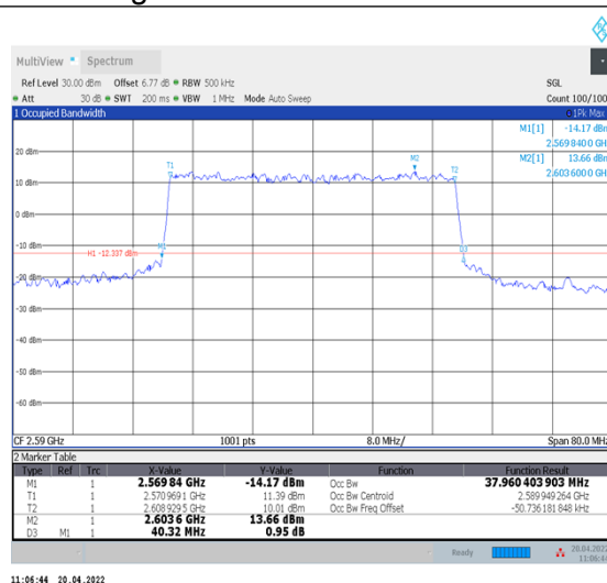
1-N38--30-40-L-6-CP-QPSK-Outer_Full-106@0-Ant1-37.96-40.320-≤40-PASS
