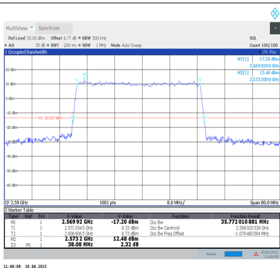
1-N38--30-40-L-5-DFT-256QAM-Outer_Full-100@0-Ant1-35.772-38.080-≤40-PASS
