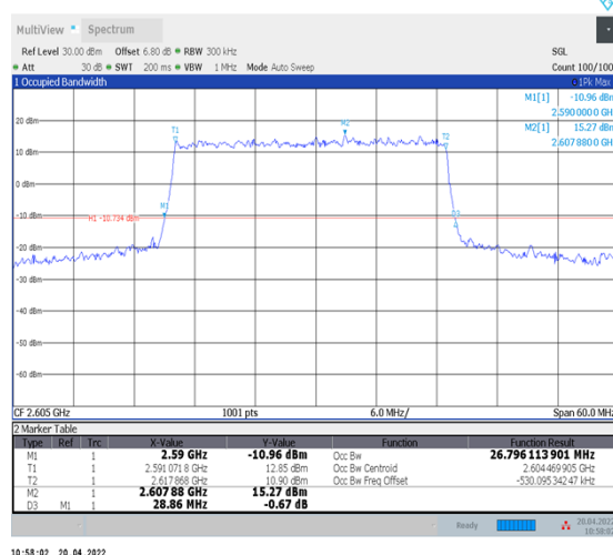
1-N38--30-30-H-1-DFT-QPSK-Outer_Full-75@0- Ant1-26.796-28.860-≤30-PASS
