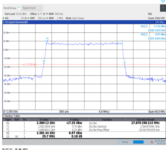
1-N38--30-30-M-9-CP-256QAM-Outer_Full-78@0- Ant1-27.87-29.700-≤30-PASS
