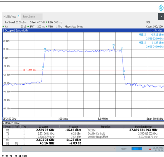
1-N38--30-40-L-9-CP-256QAM-Out_ Full-106@0-Ant1-37.89-40.160-≤40-PASS
