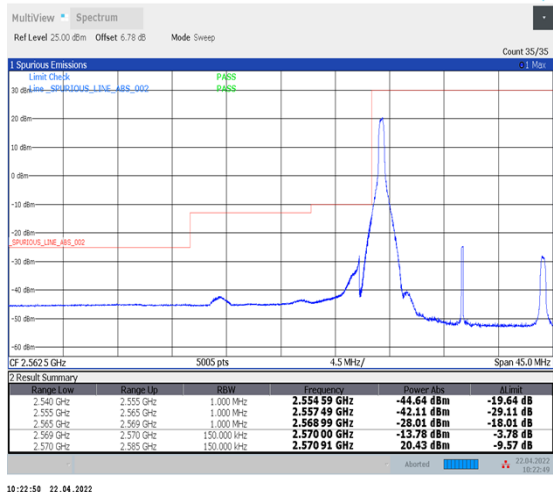
1-N38--30-15-L-1-DFT-PI2BPSK-Edge_1RB_Left-1@0-Ant1-PASS-see graph
