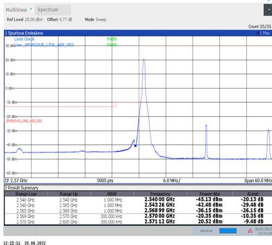
1-N38--30-30-L-4-CP-QPSK-Edge_1RB_Left-1@0-Ant1-PASS-see graph
