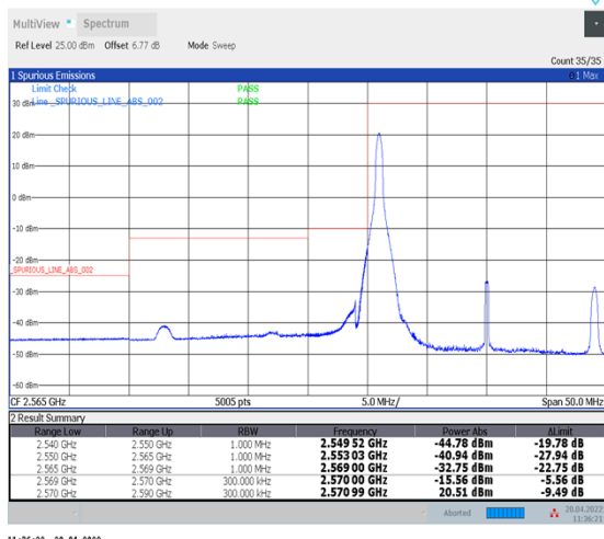
1-N38--30-20-L-4-CP-QPSK-Edge_1RB_Left-1@0-Ant1-PASS-see graph
