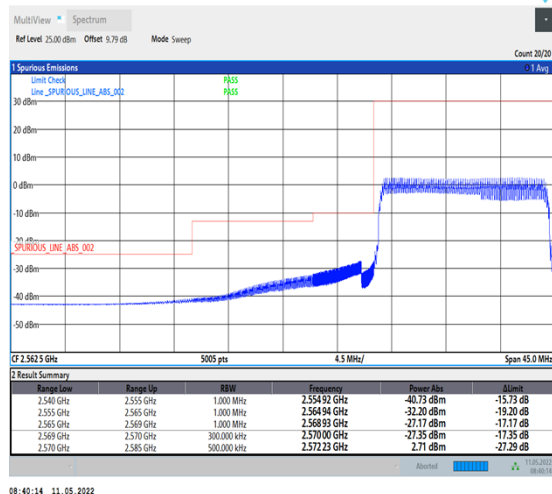
1-N38-PC2-30-15-L-6-CP-QPSK-Outer_Full-38@0-Ant1-PASS-see graph
