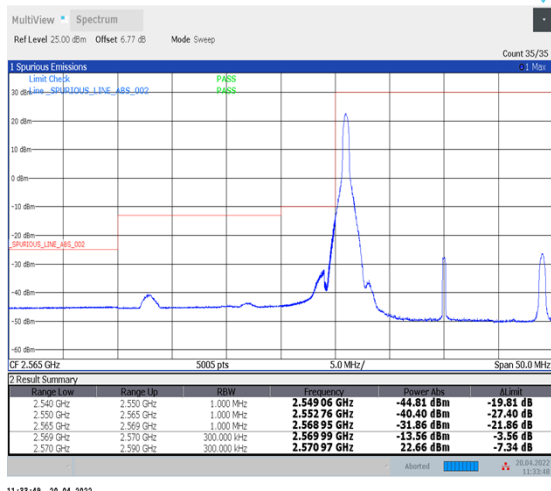
1-N38--30-20-L-1-DFT-PI2BPSK-Edge_1RB_Left-1@0-Ant1-PASS-see graph
