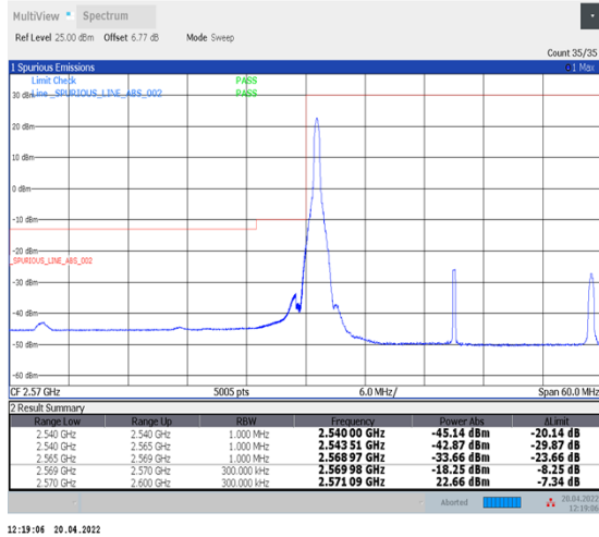
1-N38--30-30-L-1-DFT-PI2BPSK-Edge_1RB_Left-1@0-Ant1-PASS-see graph
