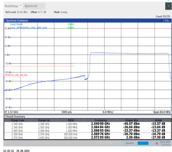
1-N38--30-30-L-6-CP-QPSK-Outer_Full-78@0-Ant1-PASS-see graph
