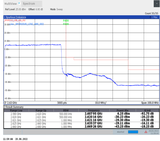
1-N38--30-40-H-3-DFT-PI2BPSK-Outer_Full-100@0-Ant1-PASS-see graph
