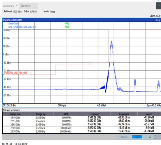
1-N38-PC2-30-15-L-4-CP-QPSK-Edge_1RB_Left-1@0-Ant1-PASS-see graph
