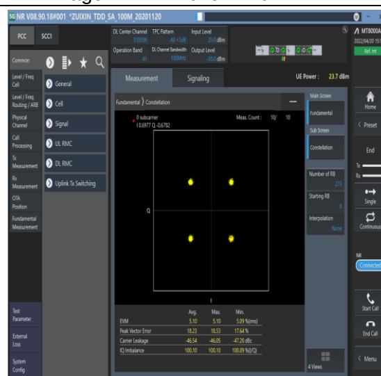
1-N41--30-100-M-6-CP-QPSK-Out_Full-273@0-Ant1-see graph-PASS
