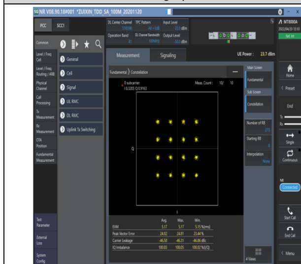
1-N41--30-100-M-7-CP-16QAM-Out_Full-273@0-Ant1-see graph-PASS
