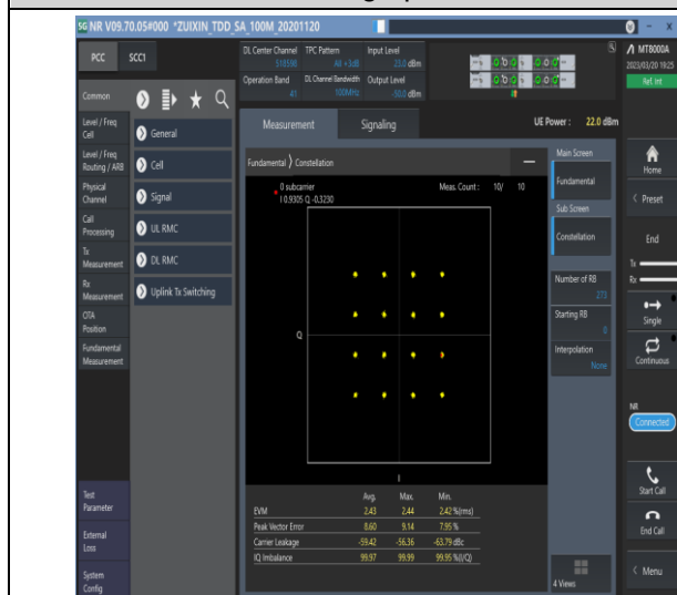
1-N41-30-100-M-7-CP-16QAM-Outer_Full-273@0-An t1-see graph-PASS
