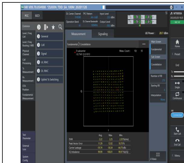
1-N41-30-100-M-5-DFT-256QAM-Outer_Full-270@0-0-Ant1-see graph-PASS
