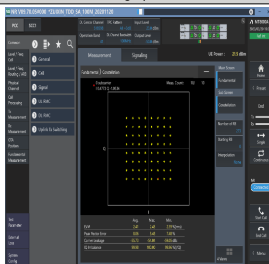
1-N41-30-100-M-8-CP-64QAM-Outer_Full-273@0-Ant1-see graph-PASS
