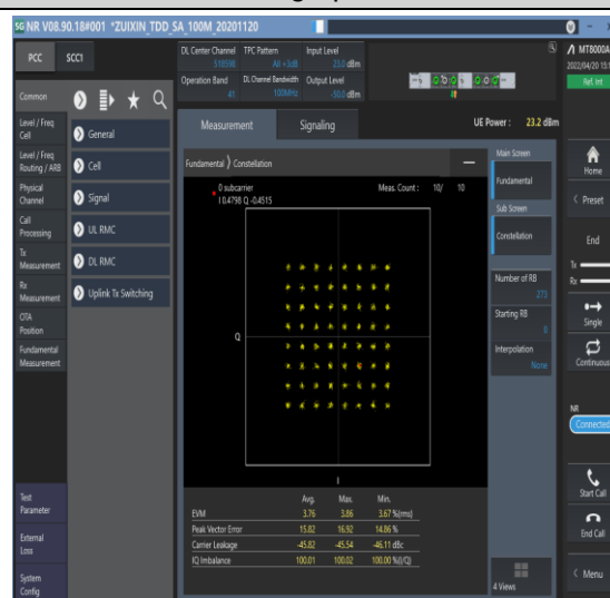
1-N41--30-100-M-8-CP-64QAM-Out_Full-273@0-Ant1-see graph-PASS
