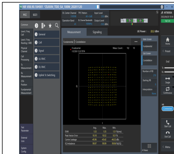
1-N41--30-100-M-5-DFT-256QAM-Out_Full-270@0-Ant1-see graph-PASS
