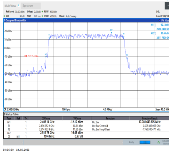
1-N41-PC1-30-20-L-2-DFT-PI2BPSK-Outer_Full-50@ @Ant1-17.782-19.400-≤20-PASS
