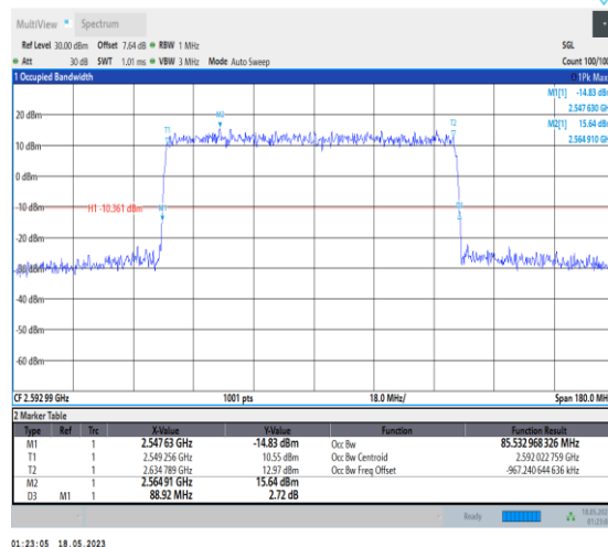
1-N41-PC1-30-90-M-4-DFT-64QAM-Outer_Full-240 @0-Ant1-85.533-88.920-≤90-PASS
