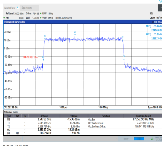
1-N41-PC1-30-90-M-6-CP-QPSK-Outer_Full-245@0 -Ant1-87.255-90.720-≤90-PASS
