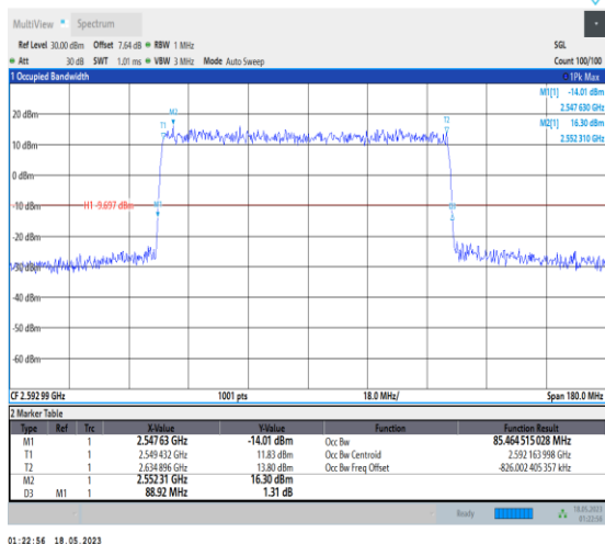
1-N41-PC1-30-90-M-3-DFT-16QAM-Outer_Full-240 @0-Ant1-85.465-88.920-≤90-PASS
