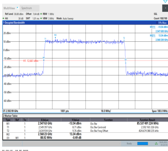
1-N41-PC1-30-90-M-5-DFT-256QAM-Outer_Full-240 @0-Ant1-85.537-88.920-≤90-PASS
