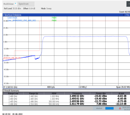
1-N41--30-20-L-6-CP-QPSK-Outer_Full-51@0-Ant1-PASS-see graph
