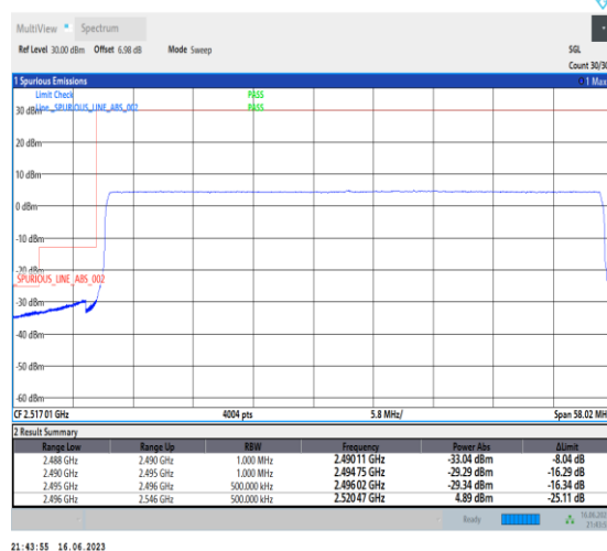
1-N41-PC1-30-50-L-6-CP-QPSK-Outer_Full-133@0-Ant1-1--PASS-see graph
