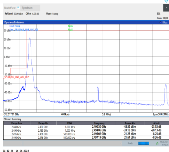
1-N41-PC1-30-50-L-4-CP-QPSK-Edge_1RB_Left-1@0-Ant1-1--PASS-see graph
