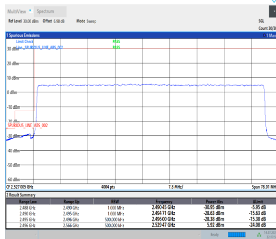
1-N41-PC1-30-70-L-3-DFT-PI2BPSK-Outer_Full-180@0-Ant1-1--PASS-see graph
