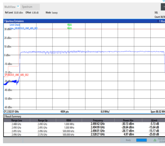
1-N41-PC1-30-80-L-3-DFT-PI2BPSK-Outer_Full-216@0-Ant1-1--PASS-see graph
