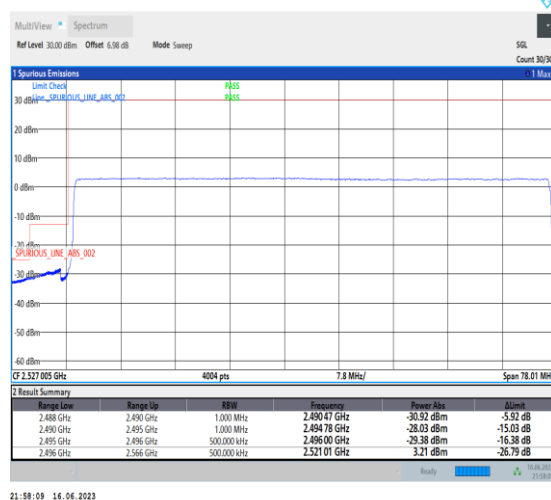
1-N41-PC1-30-70-L-6-CP-QPSK-Outer_Full-189@0-Ant1-1--PASS-see graph
