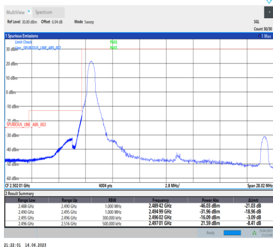
1-N41-PC1-30-20-L-4-CP-QPSK-Edge_1RB_Left-1@0-Ant1-1--PASS-see graph
