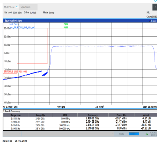
1-N41-PC1-30-20-L-6-CP-QPSK-Outer_Full-51@0-Ant1-1--PASS-see graph
