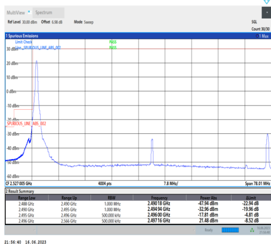
1-N41-PC1-30-70-L-4-CP-QPSK-Edge_1RB_Left-1@0-Ant1-1--PASS-see graph
