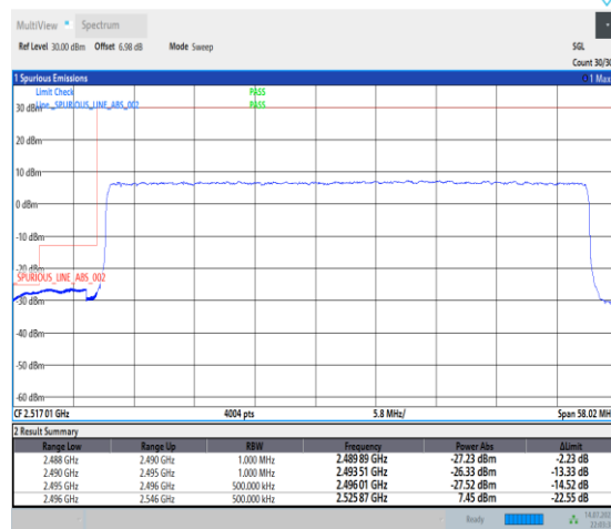
1-N41-PC1-30-50-L-3-DFT-PI2BPSK-Outer_Full-128@0-Ant1-1--PASS-see graph
