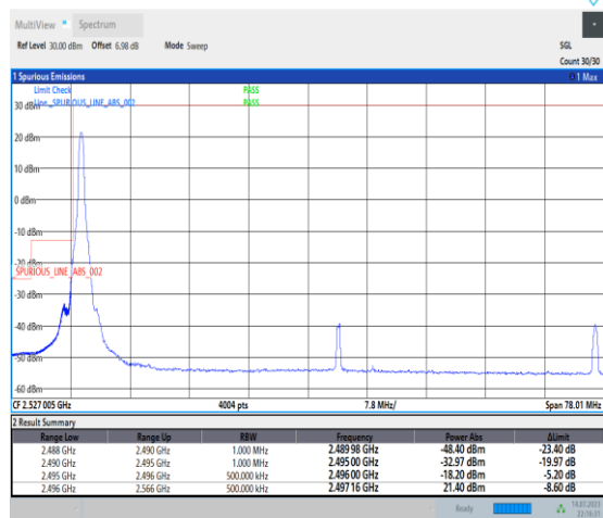
1-N41-PC1-30-70-L-1-DFT-PI2BPSK-Edge_1RB_Left-1@0-Ant1-1--PASS-see graph
