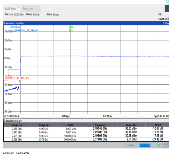
1-N41-PC1-30-80-L-6-CP-QPSK-Outer_Full-217@0-Ant1-1--PASS-see graph
