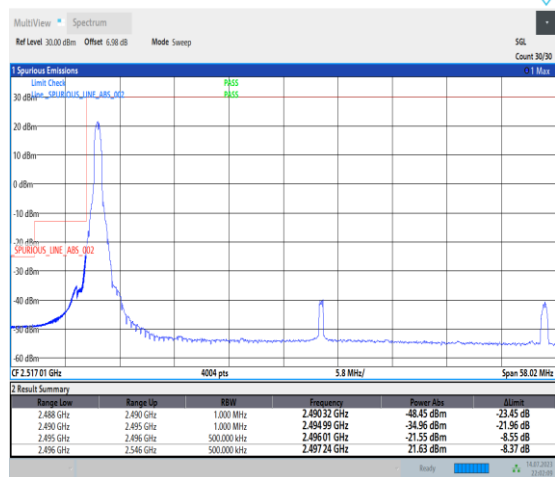
1-N41-PC1-30-50-L-1-DFT-PI2BPSK-Edge_1RB_Left-1@0-Ant1-1--PASS-see graph
