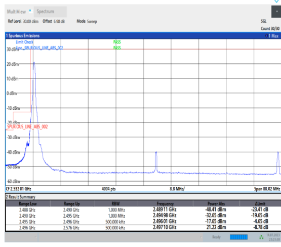
1-N41-PC1-30-80-L-1-DFT-PI2BPSK-Edge_1RB_Left-1@0-Ant1-1--PASS-see graph
