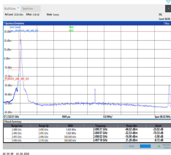
1-N41-PC1-30-80-L-4-CP-QPSK-Edge_1RB_Left-1@0-Ant1-1--PASS-see graph
