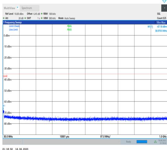
1-N41-PC1-30-100-H-1-DFT-QPSK-Edge_1RB_Left-1@0-30-1000-Ant1-30.97--67.18--35-PASS
