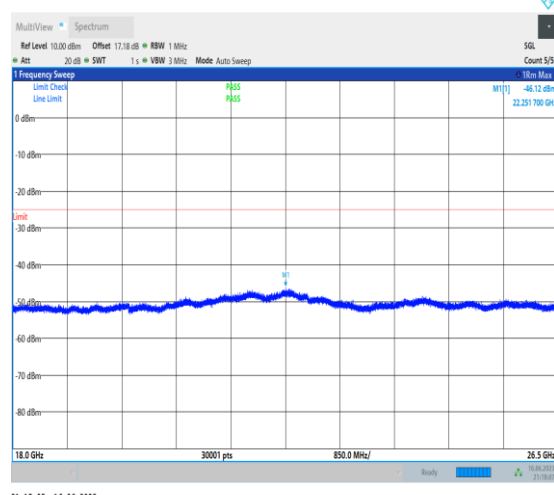
1-N41-PC1-30-100-M-1-DFT-QPSK-Edge_1RB_Left- 1@0-18000-26500-Ant1-22251.70--46.12--25-PASS
