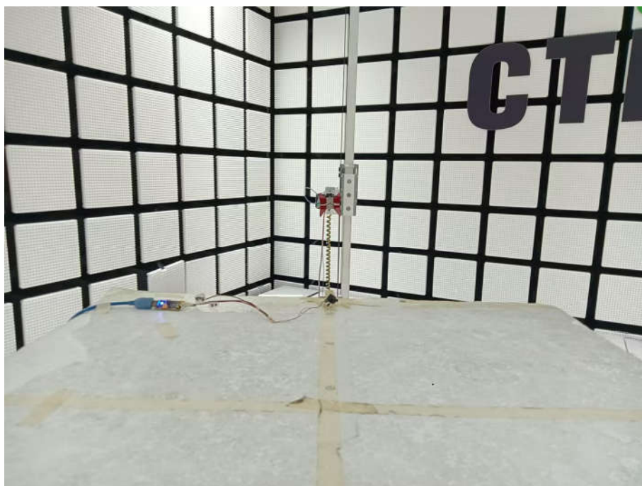
Radiated spurious emission Test Setup-4 Ear R (Above 1GHz)
