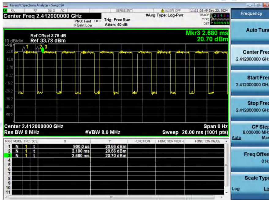
Duty_Cycle_NVNT_ANT1_802_11n(HT20)_2412
