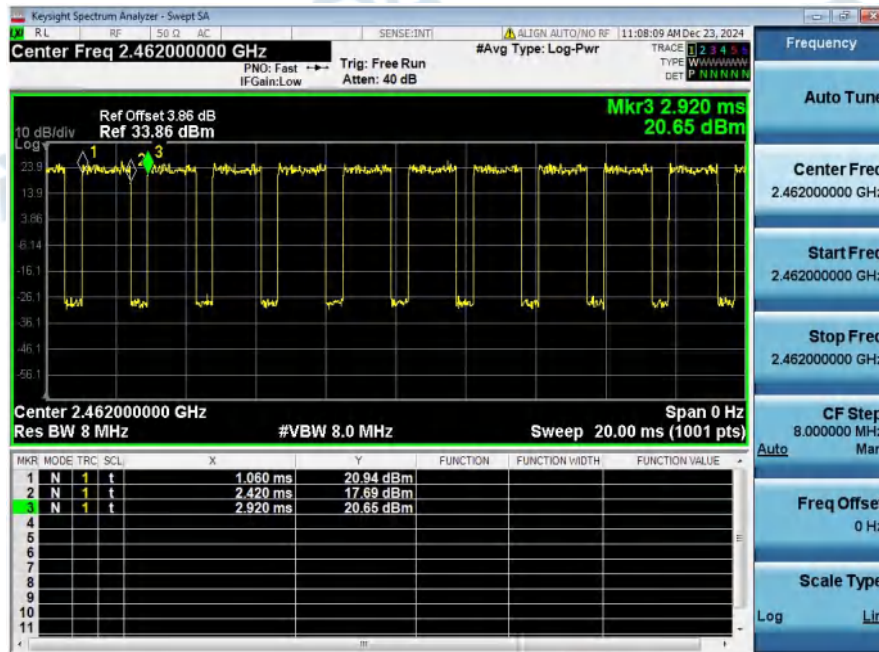
Duty_Cycle_NVNT_ANT1_802_11g_2462
