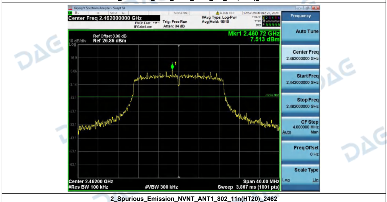
1_Reference_Level_NVNT_ANT1_802_11n(HT20)_2462
