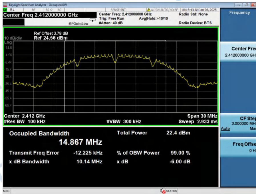
-6dB_Bandwidth_NVNT_ANT1_802_11b_2412
