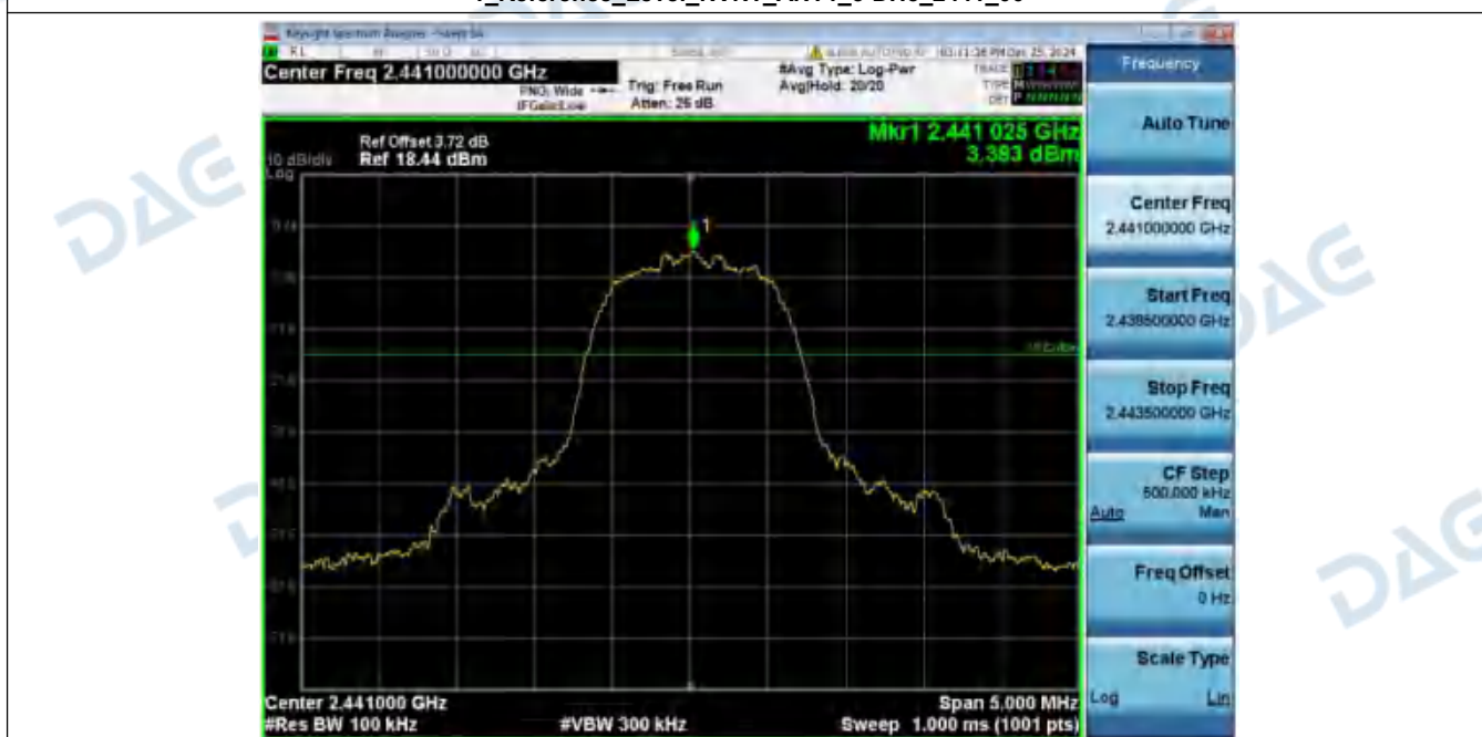
2_Spurious_Emissions_NVNT_ANT1_3-DH5_2441_00
