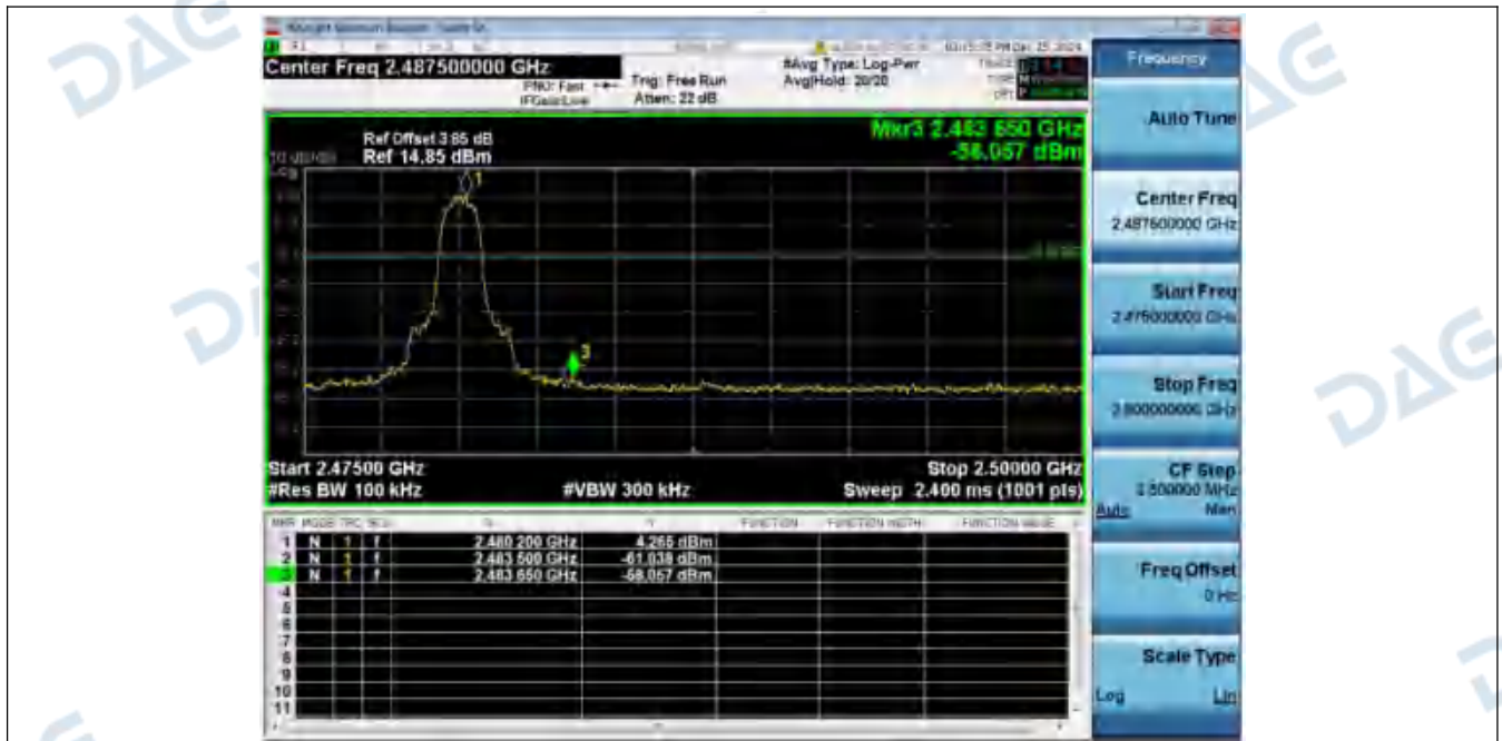
1_Reference_Level_Hopping_NVNT_ANT1_3-DH5_Hopping
