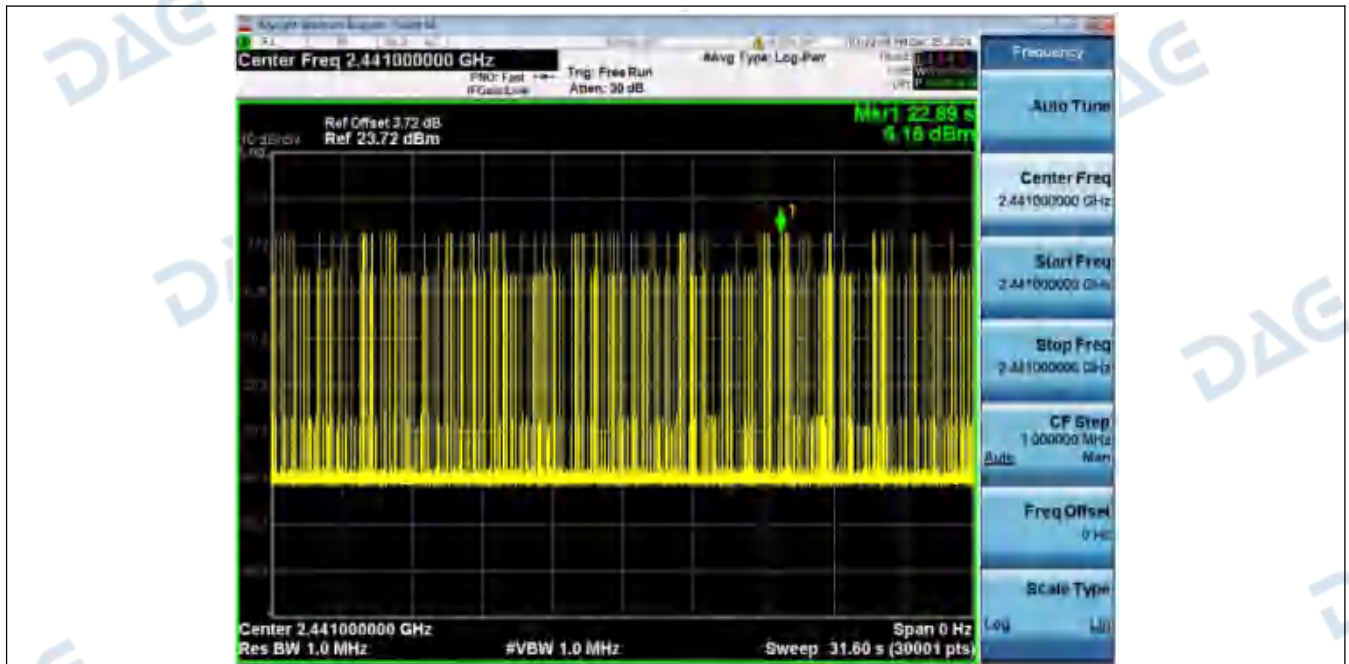
Dwell_Time_(Hopping)_NVNT_ANT1_2-DH5_2441_00_One_Burst_Time
