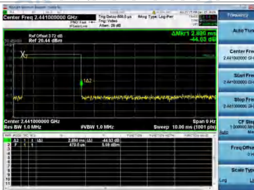
Dwell_Time_(Hopping)_NVNT_ANT1_1-DH5_2441_00_Accumulated
