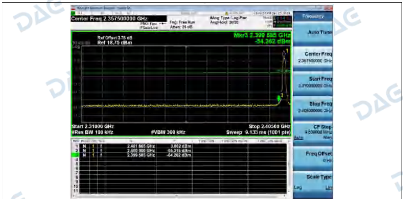
1_Reference_Level_Hopping_NVNT_ANT1_2-DH5_Hopping
