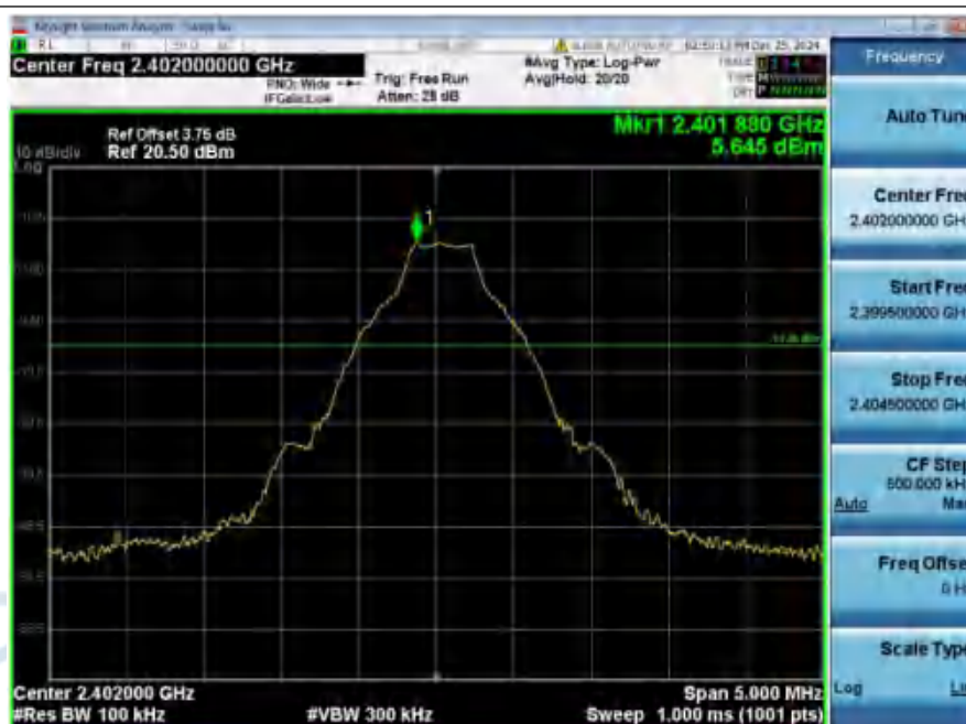
2_Bandedge_NVNT_ANT1_1-DH5_2402_00
