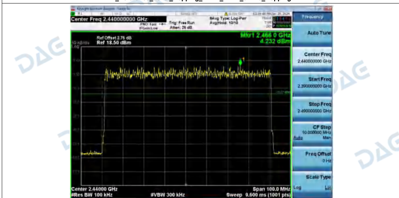
2_Band_Edge_(Hopping)_NVNT_ANT1_3-DH5_Hopping
