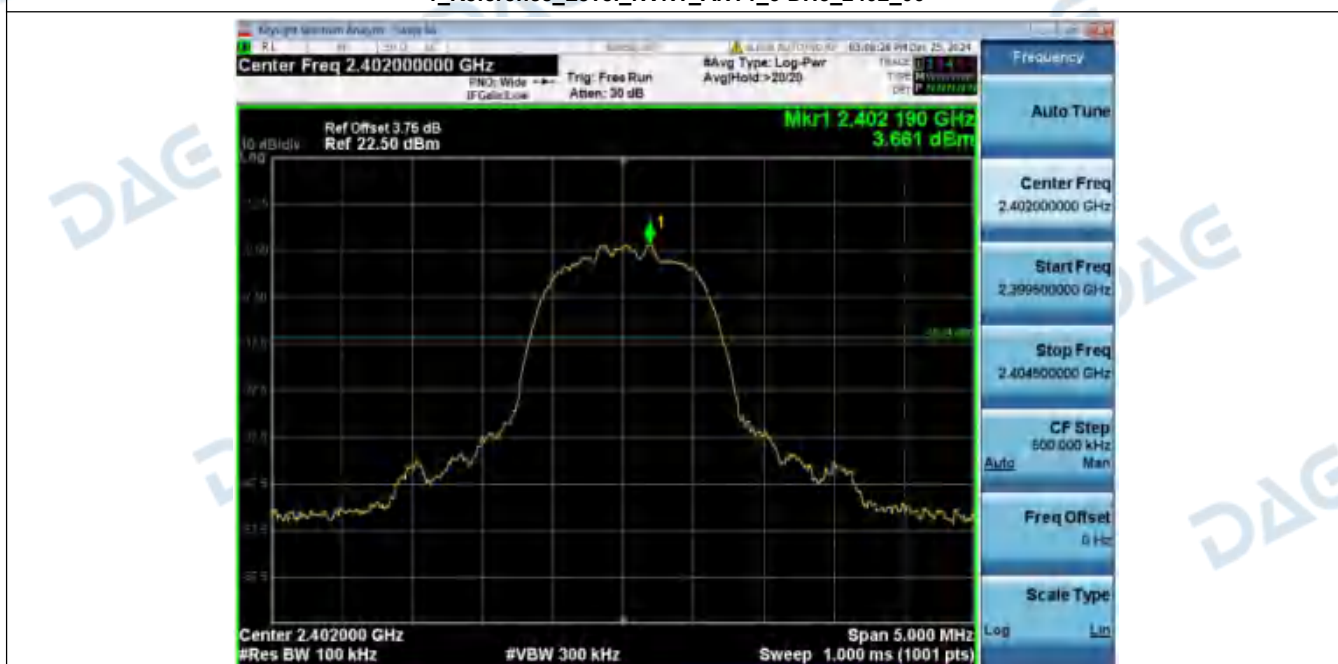
2_Spurious_Emissions_NVNT_ANT1_3-DH5_2402_00
