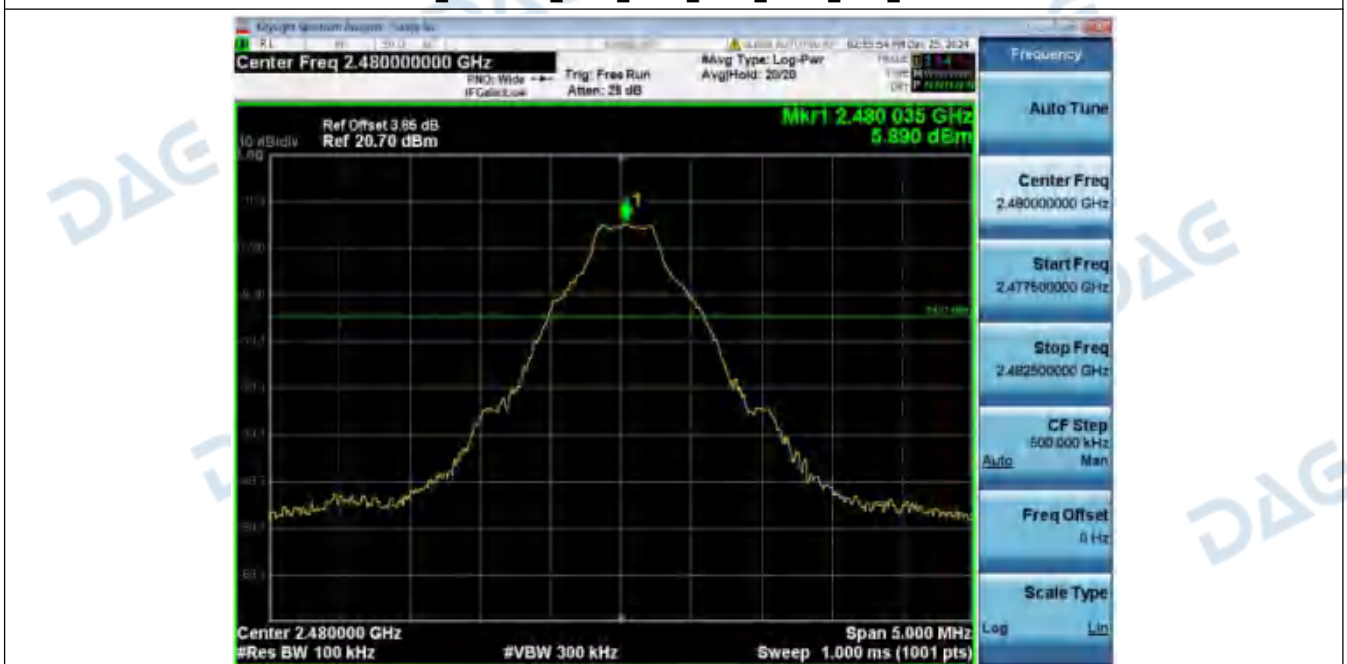
2_Bandedge_NVNT_ANT1_1-DH5_2480_00
