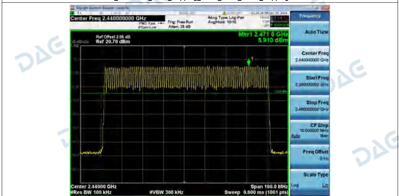
2_Band_Edge_(Hopping)_NVNT_ANT1_1-DH5_Hopping
