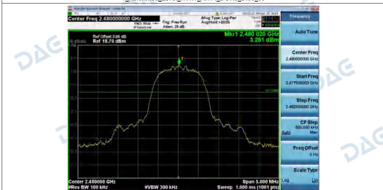
2_Spurious_Emissions_NVNT_ANT1_2-DH5_2480_00
