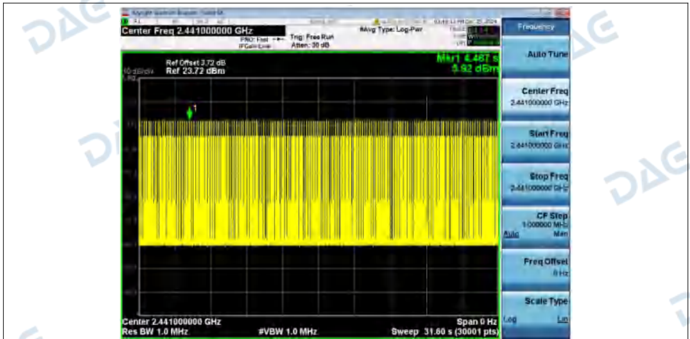
Dwell_Time_(Hopping)_NVNT_ANT1_3-DH3_2441_00_One_Burst_Time
