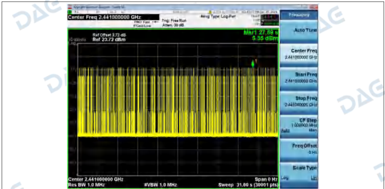
Dwell_Time_(Hopping)_NVNT_ANT1_3-DH1_2441_00_One_Burst_Time
