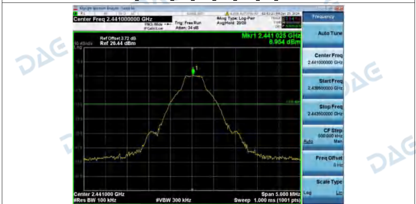
2_Spurious_Emissions_NVNT_ANT1_1-DH5_2441_00
