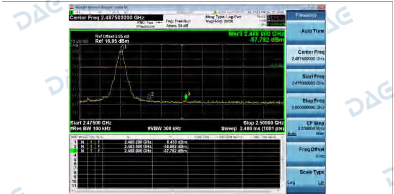
1_Reference_Level_Hopping_NVNT_ANT1_1-DH5_Hopping
