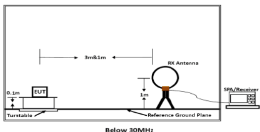
Figure 1. Below 30MHz
