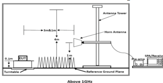
Figure 3. Above 1GHz
