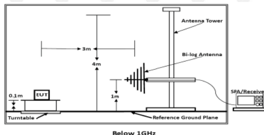
Figure 2. 30MHz to 1GHz
